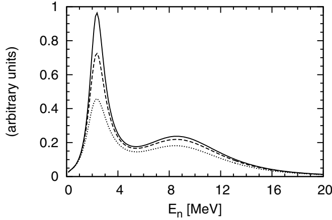
FIG. 3. The differential capture rate d^5\Gamma_{nn}/(d\mathbf{p}_\gamma d\mathbf{p}_1 dE_1) calculated with the AV18 potential [70] and using the transition operator from Eq. (2.4) as a function of the neutron energy E_n \equiv E_1 for three different angles between the emitted photon and neutron momentum \theta_{\gamma 1} : 179^\circ (solid line), 175^\circ (dashed line), and 171^\circ (dotted line). All the results correspond to a_{nn} = -18.8 fm.
