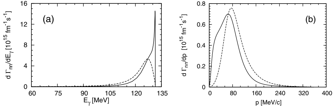
FIG. 2. The differential capture rate d\Gamma_{nn}/dE_\gamma as a function of the photon energy E_\gamma (a) and the differential capture rate d\Gamma_{nn}/dp as a function of the magnitude of the relative nn momentum p (b) for the \pi^- + ^2\text{H} \rightarrow \gamma + n + n process, calculated with the AV18 potential [70] and using the transition operator from Eq. (2.4). The dashed curves show the plane wave results and the solid curves are used for the full results.
