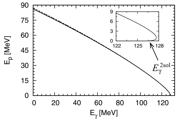
FIG. 7. The kinematically allowed region in the E_\gamma - E_p plane calculated relativistically (solid curve) and nonrelativistically (dashed curve) for the \pi^- + {}^3\text{He} \rightarrow \gamma + n + n + p process. The inset focuses on the highest photon energy region. Note that the minimal proton kinetic energy is zero for E_\gamma \leq E_\gamma^{2\text{sol}} . The lines practically overlap except for very small photon energies.
