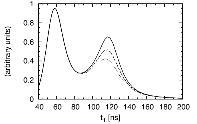
FIG. 5. The differential capture rate d^5\Gamma_{nn}/(d\mathbf{p}_\gamma d\mathbf{p}_1 dt_1) (neutron time-of-flight spectrum for a flight path of 2.55 m) obtained from the results shown in Fig. 4. The results corresponding to different a_{nn} values, represented by the same lines as in Fig. 4, are normalized at the (left) QFS peak.
