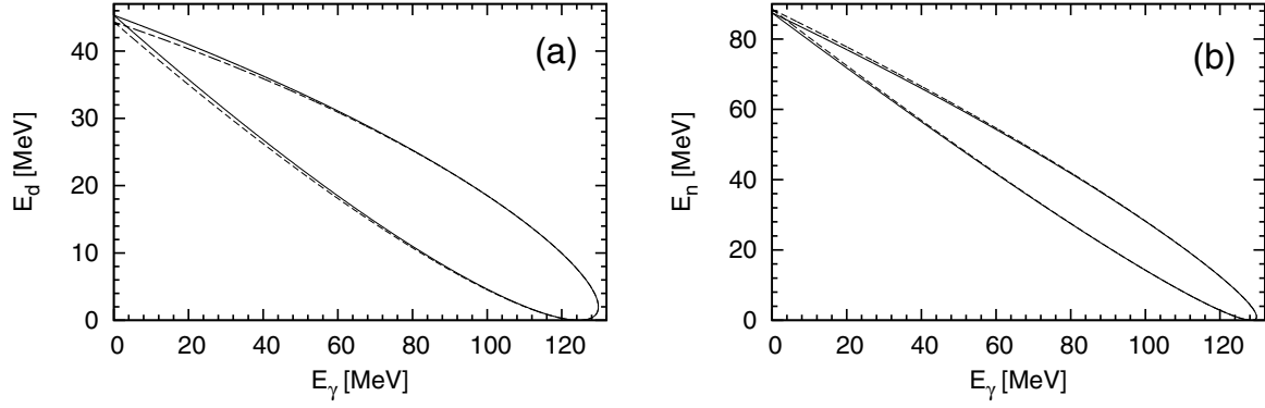
FIG. 6. The kinematically allowed region in the E_\gamma - E_d (a) and E_\gamma - E_n (b) plane calculated relativistically (solid curve) and nonrelativistically (dashed curve) for the \pi^- + {}^3\text{He} \rightarrow \gamma + n + d process. The lines overlap except for small photon energies.
