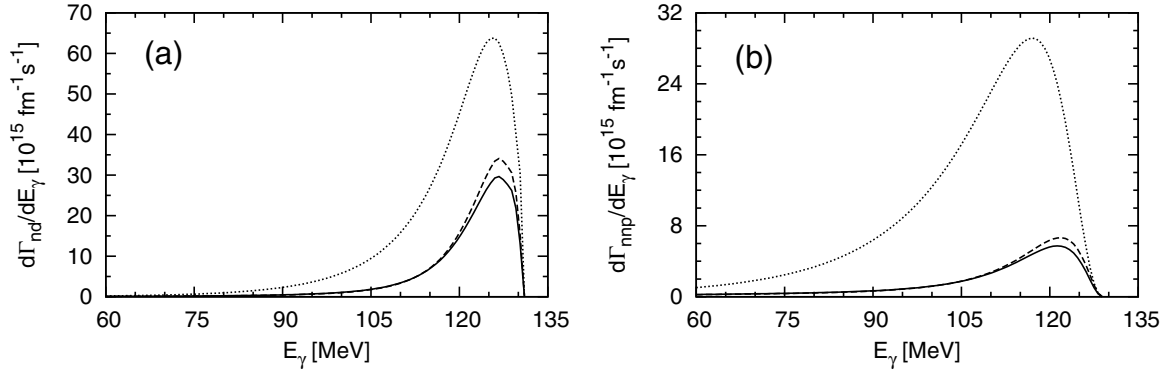
FIG. 8. The differential capture rate d\Gamma_{nd}/dE_\gamma for the \pi^- + {}^3\text{He} \rightarrow \gamma + n + d process (a) and the differential capture rate d\Gamma_{nnp}/dE_\gamma for the \pi^- + {}^3\text{He} \rightarrow \gamma + n + n + p reaction (b) as a function of the photon energy, calculated with the single-nucleon transition operator and with different treatment of 3N dynamics: taking the symmetrized plane wave (SPW) approximation (dotted line) and calculating the initial and final 3N states without (dashed curve) and with (solid line) 3N force. The calculations are based on the AV18 NN potential [70] and the Urbana IX 3N force [71].
