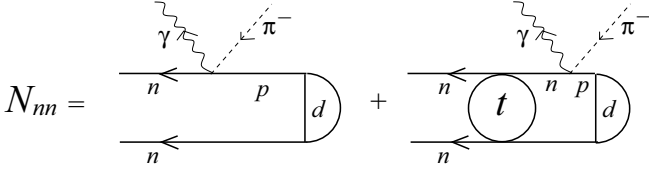
FIG. 12. Diagrammatic representation of the 2N matrix element for the radiative pion capture reaction, assuming a single-nucleon mechanism. The circular segment on the right stands for the initial deuteron. The left diagram corresponds to the plane wave (PW) part of N_{nn,\pm 1} , and the circle in the second diagram represents the rescattering described by the t matrix.
