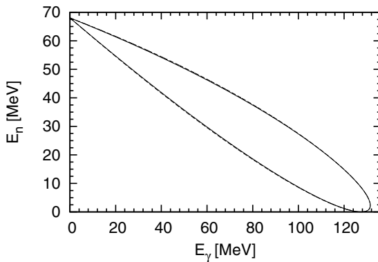
FIG. 1. The kinematically allowed region in the E_\gamma - E_n plane calculated relativistically (solid curve) and nonrelativistically (dashed curve) for the \pi^- + {}^2\text{H} \rightarrow \gamma + n + n capture process. The lines practically overlap.
