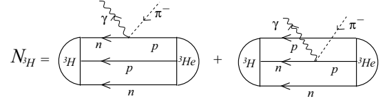
FIG. 13. Diagrammatic representation of the 3N matrix element for the \pi^- + {}^3\text{He} \rightarrow \gamma + {}^3\text{H} reaction, assuming that the pion is captured only by single protons. The circular segment on the right (left) stands for initial {}^3\text{He} (final {}^3\text{H} ).
