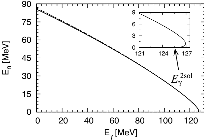
FIG. 10. The kinematically allowed region in the E_\gamma - E_n plane calculated relativistically (solid curve) and nonrelativistically (dashed curve) for the \pi^- + {}^3\text{H} \rightarrow \gamma + n + n + n capture process.
