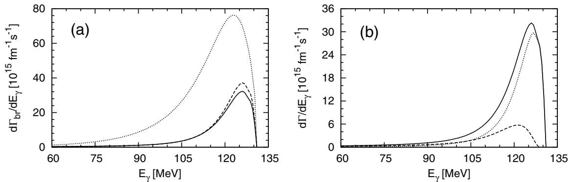
FIG. 9. As in Fig. 8 but for (a) the differential breakup capture rate d\Gamma_{br}/dE_\gamma = d\Gamma_{nd}/dE_\gamma + d\Gamma_{nnp}/dE_\gamma . In (b) the two-body d\Gamma_{nd}/dE_\gamma (dotted curve) and three-body d\Gamma_{nnp}/dE_\gamma (dashed curve) breakup contributions to the differential breakup radiative pion capture rate d\Gamma_{br}/dE_\gamma (solid curve) are displayed as a function of the photon energy. They are obtained with the single-nucleon transition operator and with full 3N dynamics (including 3N force in the initial and final nuclear states). As before, the calculations are based on the AV18 NN potential [70] and the Urbana IX 3N force [71].
