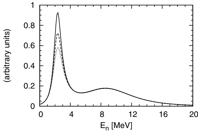
FIG. 4. The differential capture rate d^5\Gamma_{nn}/(d\mathbf{p}_\gamma d\mathbf{p}_1 dE_1) as a function of the neutron energy E_n \equiv E_1 calculated with the transition operator from Eq. (2.4) and with three versions of the AV18 potential [70] yielding different a_{nn} values: -21.8 fm (solid line), -18.8 fm (dashed line) and -16.5 fm (dotted line). All the results correspond to \theta_{\gamma 1} = 179^\circ .
