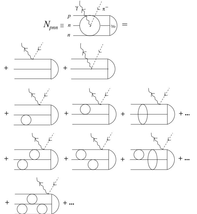
FIG. 14. The same as in Fig. 13 but for the \pi^- + {}^3\text{He} \rightarrow \gamma + p + n + n breakup reaction, assuming a single-nucleon pion capture mechanism and neglecting the 3N force. The open circles and ovals represent the two-nucleon t matrices acting in the three different subsystems. The subsequent rows show the symmetrized plane wave contributions (SPW) and selected diagrams representing rescattering of the first, second, and third order in the t matrix.
