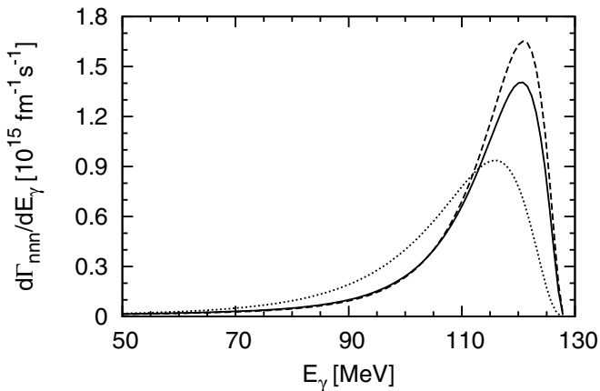
FIG. 11. The same as in the right panel of Fig. 8 but for the differential capture rate d\Gamma_{nnn}/dE_\gamma in the case of the \pi^- + {}^3\text{H} \rightarrow \gamma + n + n + n process.
