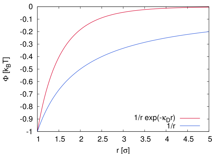
Figure 2. Electrostatic potential \Phi(r) between two differently charged species at distance r in presence of a finite salt density according to Equation (3) with \kappa_D^{-1} = \sigma (red line), and for unscreened Coulomb interactions with \Phi(r) \sim 1/r (blue line). The electrostatic potential at the hydrodynamic boundary of the object r_s = \sigma is arbitrarily chosen with \Phi_s = -k_B T .
