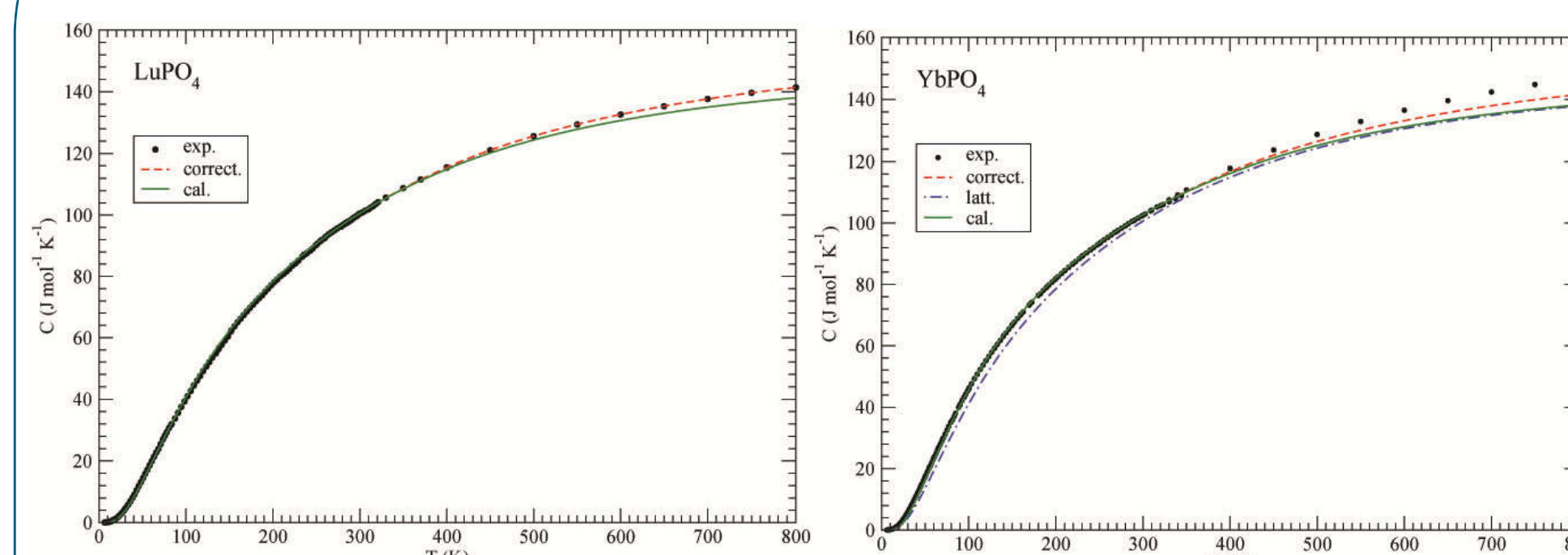
Fig. 6. The calculated and measured heat capacity of LuPO_4 and YbPO_4 [4].
