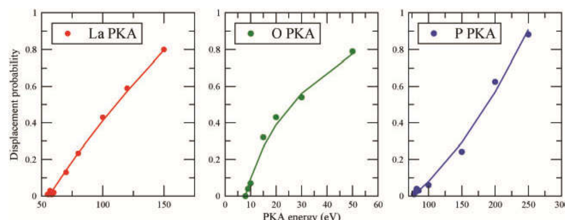
Fig. 2. The simulated atomic displacement probabilities of La, P, O PKA in LaPO_4 at T=300K [1]
