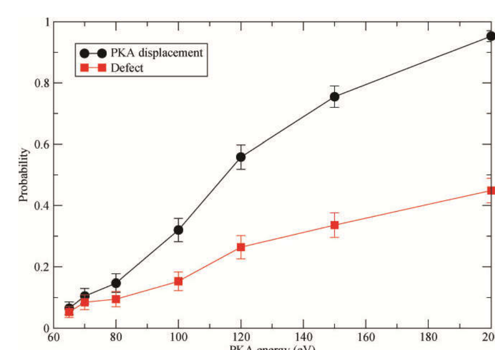
Fig. 4. The displacement probabilities (DP) and the defect formation probabilities (DFP) for the La PKA at 300 K.
