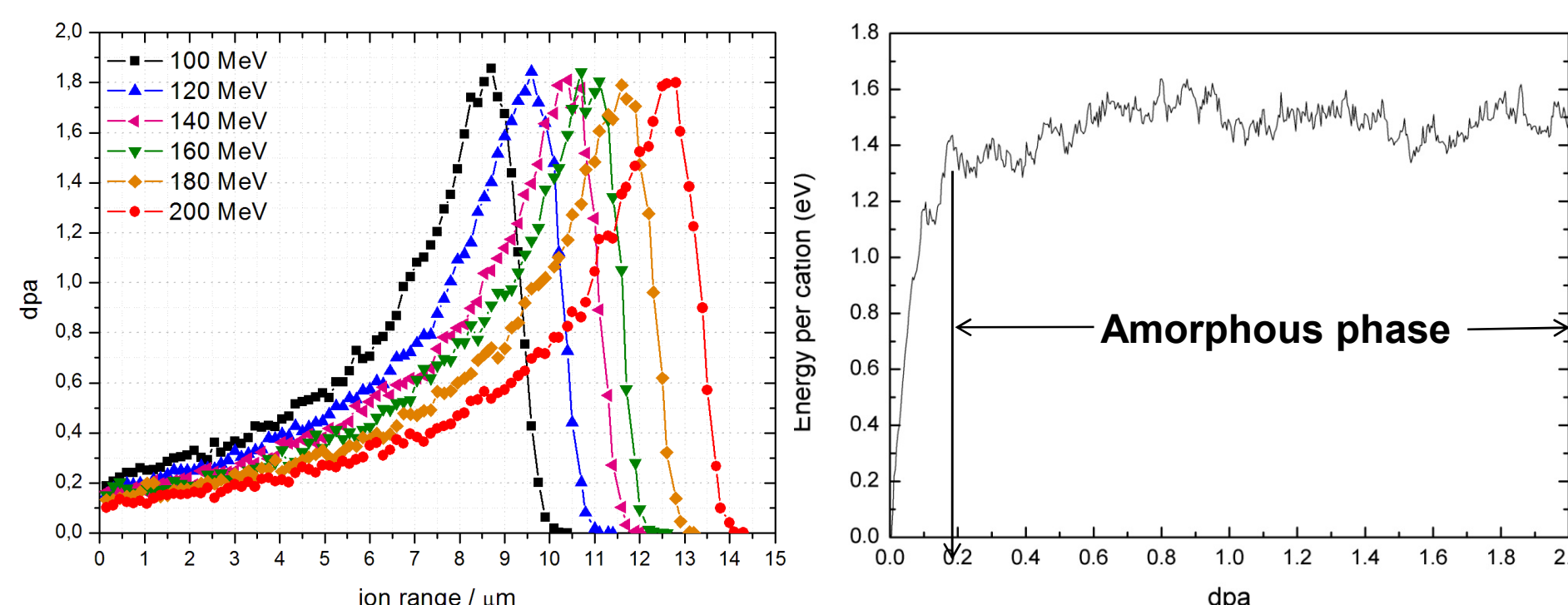
Fig. 5. Left: simulation of radiation damage: Au on LaPO_4 , simulated by Dr. Andre Filby, Dr. Ralf Kunz and Dr. Thomas Moeller (BRENK GmbH, Aachen) using E_d we calculated. Right: simulation of critical amorphization dose.
