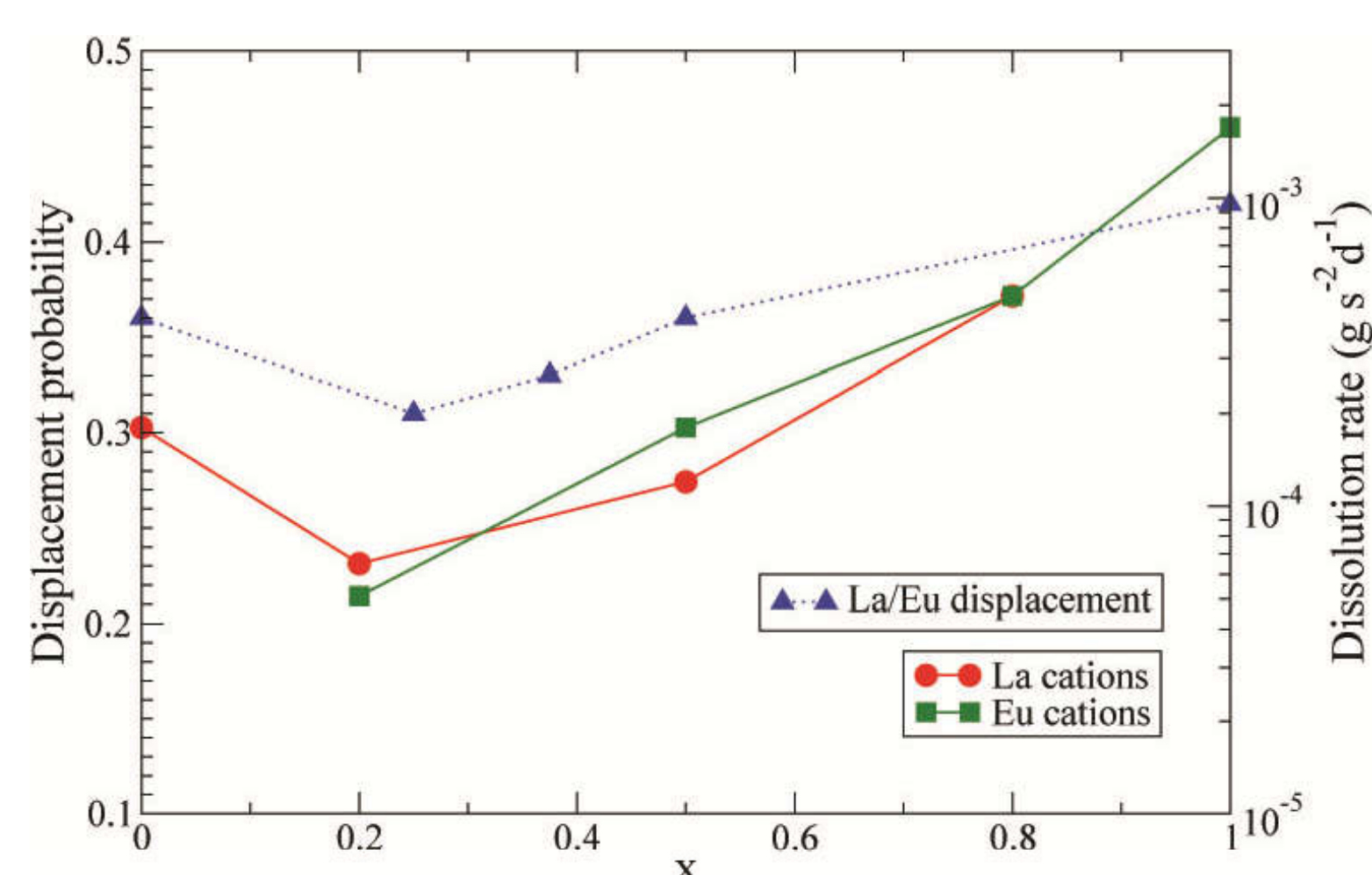
Fig. 3. The atomic displacement probability of La_{1-x}Eu_xPO_4 solid solution (left y-axis) [3] and the normalized steady-state dissolution rates measured for La_{1-x}Eu_xPO_4 solid solution and calculated from the released Eu and La concentrations [2] (right y-axis).
