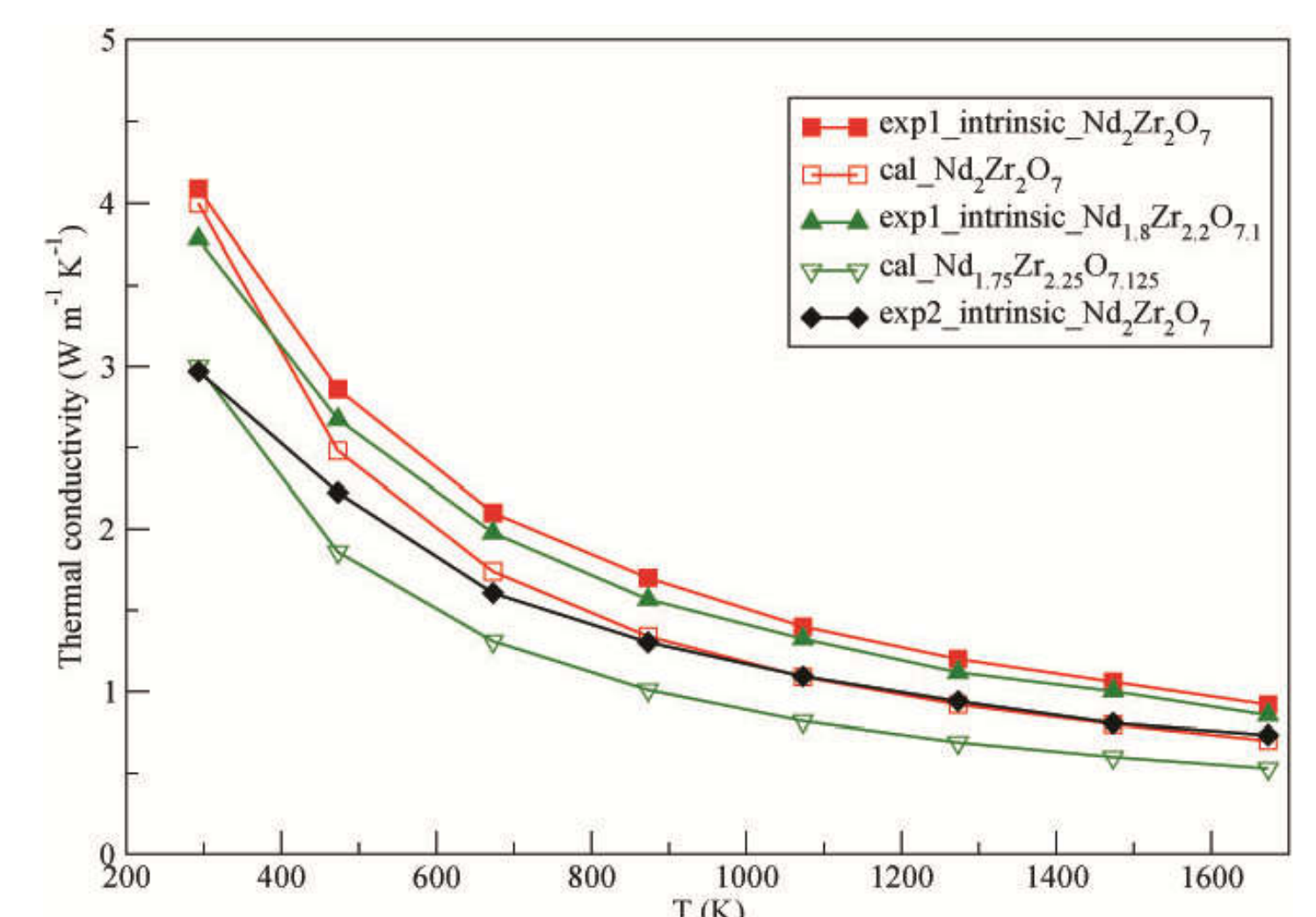
Fig. 7. The calculated and measured thermal conductivities of different Nd,Zr_{1-x}O_{2-x/2} [6,7].
