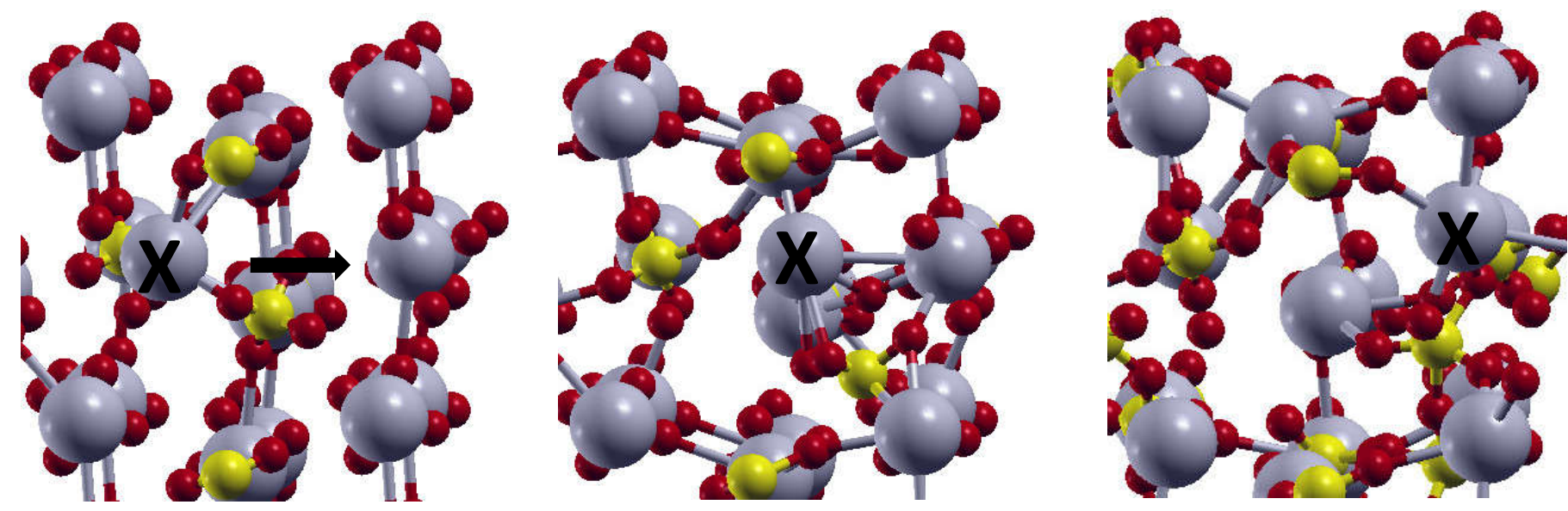
Fig. 1. Creation of the Ln -cation displacement in monazite by application of initial velocity (illustration of the simulation method).
