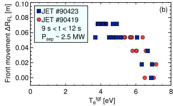
Fig. 6. Spectroscopic measurements of c_N and the amount of movement of the N II emission front away from the strike point are shown as a function of the strike point temperature from Langmuir probes for two JET L-mode plasma in (a) and (b), respectively. Scaling law predictions of c_N required for detachment are indicated in (b) by the dashed lines for two values of f_{GW, sep} .
