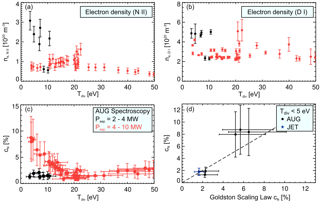
Fig. 4. The electron density calculated using the N II line ratio (averaged over results with T_{e, NII} = 3.5-4.0 eV) and using Stark broadening is shown in (a) and (b), respectively, as a function of T_{div} . Corresponding measurements of c_N from AUG H-mode plasma are shown in (c). The c_N measurements in AUG plasma with T_{div} \leq 5 eV are compared with scaling law predictions for detachment from Goldston et al. in (d). The data from JET at T_e^{igt} < 4 eV is shown by the blue symbol. (For interpretation of the references to colour in this figure legend, the reader is referred to the web version of this article.)
