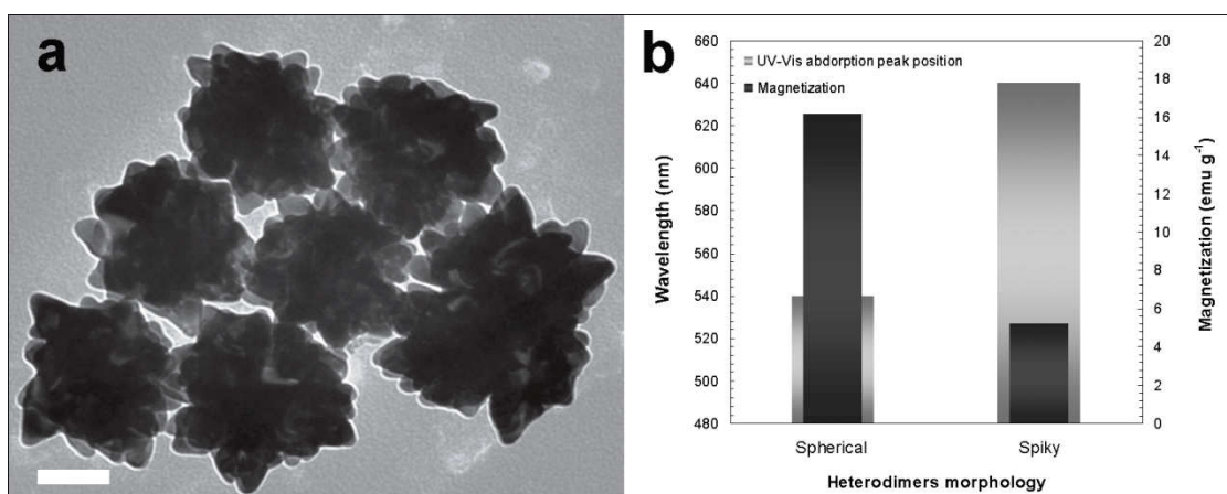
Figure 6. \text{Fe}_3\text{O}_4 -Au heterodimers. TEM image of spiky-shaped structure, scale bar: 100 nm (a) and Variation charts of magnetization and UV-Vis absorption peak position as a function of morphology (b). Adapted from reference [177].
