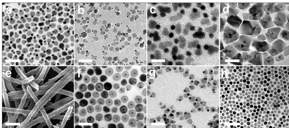
Figure 2. Microscopic images of different metallic-nonmetallic heterodimers. TEM image of \text{Fe}_3\text{O}_4 -Au heterodimers, scale bar: 40 nm, reproduced with permission from [110], copyright (2015) American Chemical Society (a), TEM image of \text{Fe}_3\text{O}_4 -Ag heterodimers, scale bar: 40 nm, with permission from [111], copyright (2017) Elsevier (b), TEM image of \text{Fe}_3\text{O}_4 -Pt heterodimers, scale bar: 30 nm, with permission from [112], copyright (2013) American Chemical Society (c), TEM image of \text{Fe}_3\text{O}_4 -Pd heterodimers, scale bar: 30 nm, with permission from [113], copyright (2011) Royal Society of Chemistry (d), SEM image of \text{CoFe}_2\text{O}_4 -Pd heterodimers, scale bar: 300 nm, with permission from [117], copyright (2016) Royal Society of Chemistry (e), TEM image of \text{MnO} -Au heterodimers, scale bar: 40 nm, with permission from [121], copyright (2014) American Chemical Society (f), TEM image of \text{FePt} -CdS heterodimers, scale bar: 40 nm, with permission from [123], copyright (2009) American Chemical Society (g), and TEM image of \text{CdO} - \text{FePt} heterodimers, scale bar: 100 nm, with permission from [73], copyright (2014) American Chemical Society (h).
