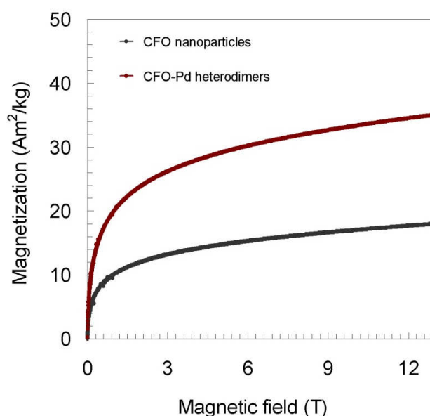
Figure 7. M-H curves of superparamagnetic \text{CoFe}_2\text{O}_4 nanoparticles (CFO, mean hydrodynamic size: 24 nm) and \text{CoFe}_2\text{O}_4 -Pd (CFO-Pd, mean particles size of Pd: 2 nm) heterodimers measured by vibrating sample magnetometer (VSM) magnetometry at 300 K.
