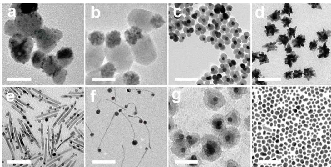
Figure 4. TEM images of heterodimers with different interfacial morphologies. Random-decorated \text{Fe}_2\text{O}_3 -Pd heterodimers, scale bar: 30 nm, reproduced with permission from [32], copyright (2015), Royal Society of Chemistry (a), Janus \text{Fe}_3\text{O}_4 -antibody dye heterodimers, scale bar: 100 nm, with permission from [143], copyright (2018) Elsevier (b), Flower-shaped \text{MnO} -Au heterodimers, scale bar: 50 nm, with permission from [121], copyright (2014) American Chemical Society (c), Star-shaped \text{FeO}_x -Au heterodimers, scale bar: 100 nm [107], published by The Royal Society of Chemistry (d), Rod-shaped \text{Fe}_2\text{O}_3 - \text{TiO}_2 heterodimers, scale bar: 200 nm, with permission from [144], copyright (2009) Royal Society of Chemistry (e), Dumbbell-shaped \text{FePt} -Au heterodimers, scale bar: 30 nm, with permission from [90], copyright (2011) Springer Nature (f), Mosaic \text{Fe}_3\text{O}_4 -Au(thiol)@ \text{SiO}_2 heterodimers, scale bar: 50 nm, with permission from [108], copyright (2015) Elsevier (g), and Core-shell \text{Fe}_3\text{O}_4 @Au heterodimers, scale bar: 50 nm, with permission from [145], copyright (2005) American Chemical Society (h).
