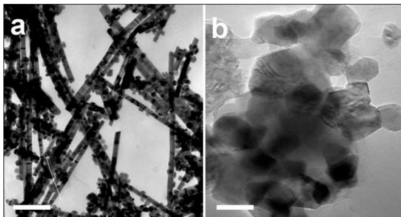
Figure 3. TEM images of different nonmetallic-nonmetallic heterodimers. \text{Fe}_2\text{O}_3 -CdS heterodimers, scale bar: 300 nm, reproduced with permission from [134], copyright (2009) American Chemical Society (a), and \text{CoFe}_2\text{O}_4 -ZnO heterodimers, scale bar: 50 nm, with permission from [137], copyright (2013), Elsevier (b).
