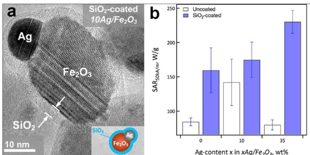
Figure 5. SiO 2 coated Fe 2 O 3 -Ag heterodimers. HRTEM image of heterodimer structure, with 10 wt% Ag (a) and specific absorption rate (SAR) values of uncoated and SiO 2 coated heterodimers with different Ag concentrations (b). Reproduced with permission from [17], copyright (2013) American Chemical Society.
