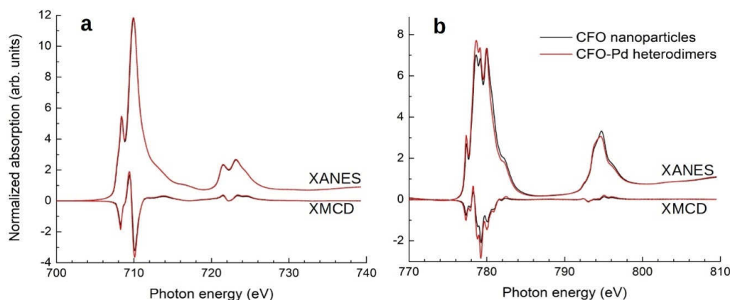
Figure 8. X-ray absorption near-edge structure (XANES) and magnetic circular dichroism (XMCD) of bare \text{CoFe}_2\text{O}_4 nanoparticles (CFO, black lines) and after Pd decoration (CFO-Pd, red lines). Measurements were performed at 5 K in a magnetic field of 6 T at the \text{Fe L}_{3,2} absorption edges (a) and \text{Co L}_{3,2} absorption edges (b).
