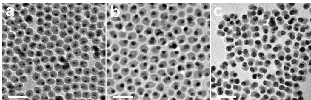
Figure 1. Transmission electron microscopy (TEM) images of Fe-Au heterodimers with different particles sizes. 15–4 nm Fe-Au heterodimers (a), 7–13 nm Fe-Au heterodimers (b), and 11–10 nm Fe-Au heterodimers (c), scale bars: 50 nm. Reproduced with permission from [81], copyright (2016) Royal Society of Chemistry.
