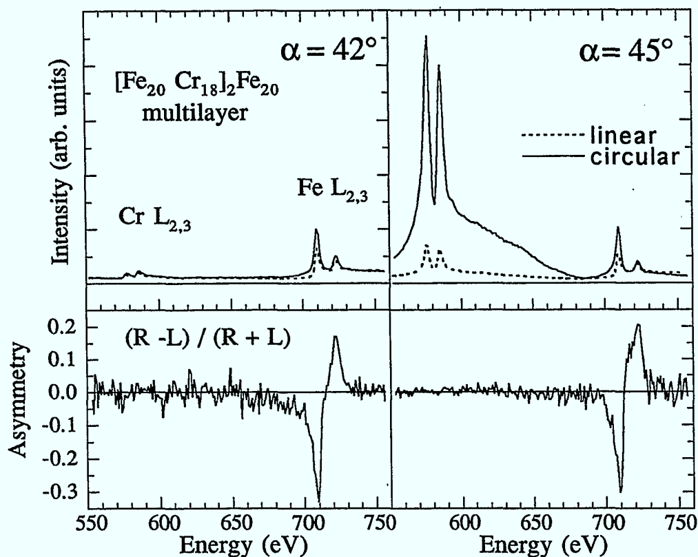
Fig. 6.9. 45^\circ reflection spectrum at the Cr and Fe L_{2,3} absorption edges of a [\text{Fe}_{20}\text{\AA} \text{Cr}_{18}\text{\AA}]_2 \text{Fe}_{20}\text{\AA} multilayer. left. not complete reflection \alpha = 42^\circ . right: reflection at \alpha = 45^\circ . solid line: circularly polarized light; dashed line: linearly (p-) polarized light.
