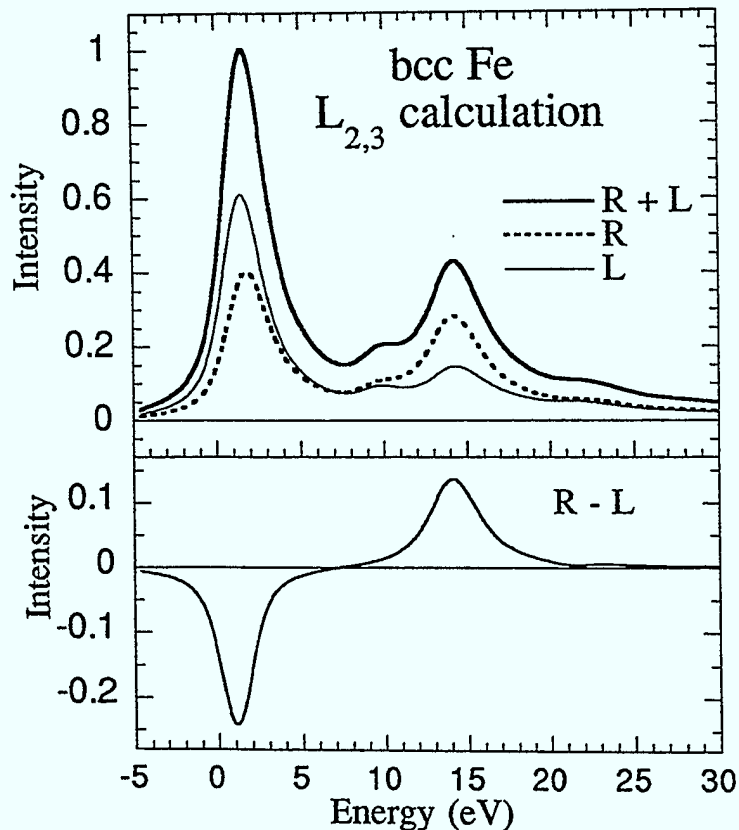
Fig. 3.2. Calculated Fe L_{2,3} absorption spectra for parallel (R) and antiparallel (L) coupling of the magnetization to the light helicity, as well as the sum ( R + L ) and the difference of both spectra ( R - L ).
