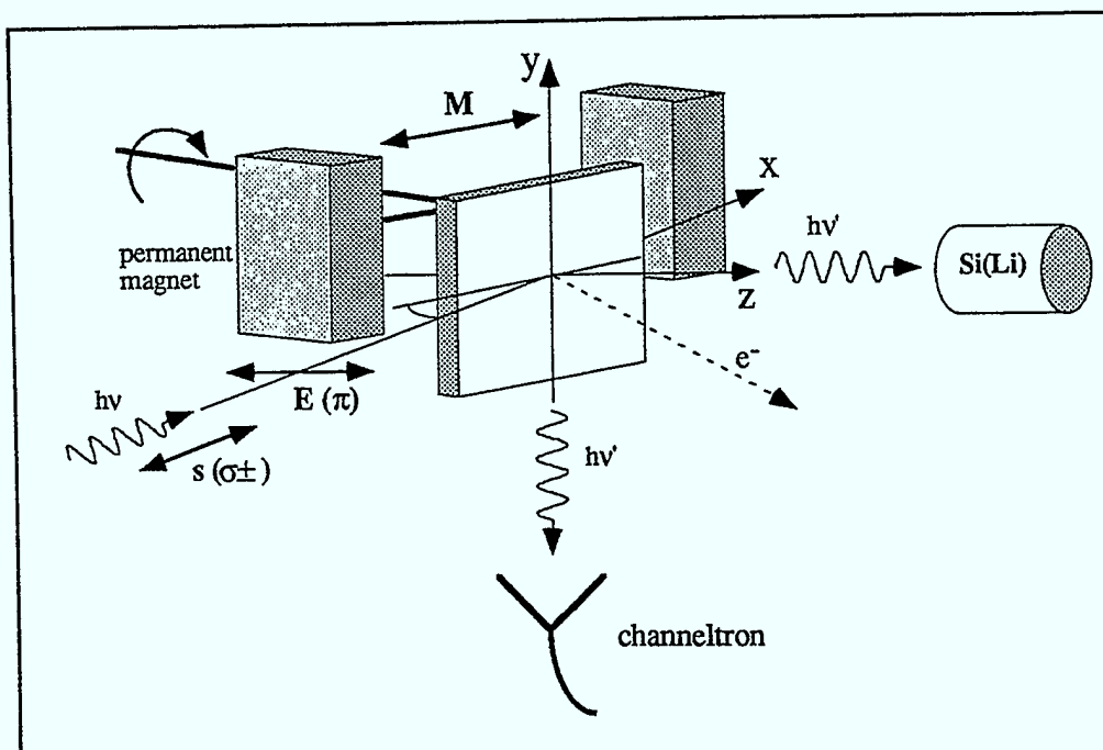
Fig. 4.3 Schematic setup of the experiment
