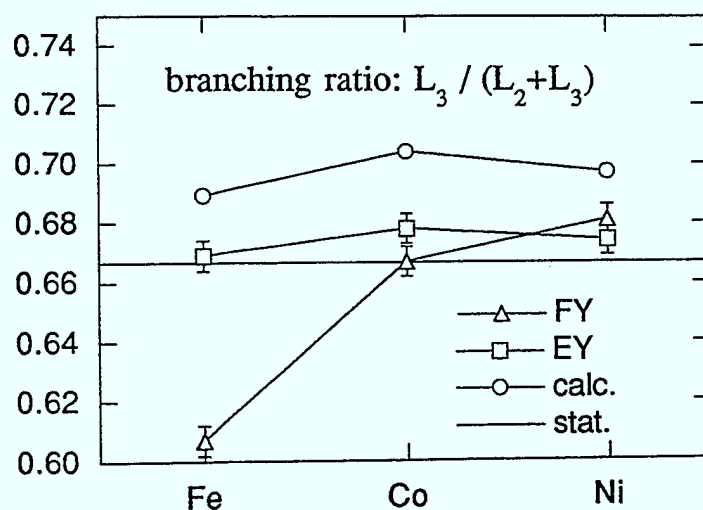
Fig 5.5. L_{2,3} branching ratio of the isotropic spectra for Fe, Co and Ni measured in FY and EY mode compared to first principle calculations.
