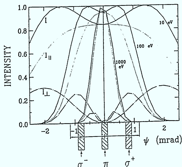
Fig.4.1. I_{\parallel} and I_{\perp} as a function of the off-plane angle \psi for three different photon energies at a BESSY dipole magnet [Petersen 93]; included are the SX700/3 acceptances for \psi = 0 and for \sigma^{\pm} - light. The total intensity I = I_{\parallel} + I_{\perp} is also given.
