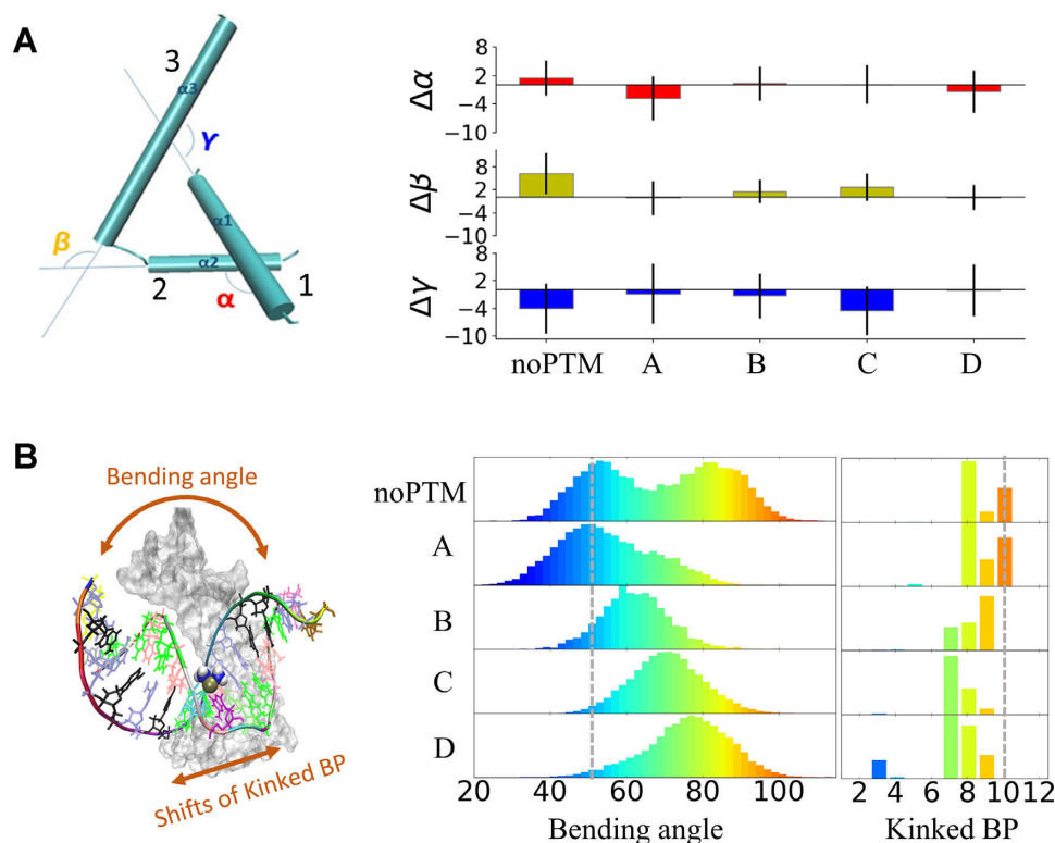
Figure 2. (A) Conformation of the helices in the box-region. Left: definition of the inter-helical spatial angles ( \alpha , \beta and \gamma ). Right: histogram showing deviations of \alpha , \beta and \gamma relative to the X-ray structure ( \alpha = 115^\circ , \beta = 114^\circ and \gamma = 117^\circ ); error bars indicate the standard deviations. (B) Distributions of bending angle and shifts of kinked base-pair (Kinked BP). Left: graphical representation of bending angle and shifts of Kinked BP. Right: distribution of bending angle and Kinked BP shifts of the platinated DNA. Distributions from lower to higher values are colored spanning from blue to red. Bending angle and Kinked BP of the X-ray structure are marked as grey dot lines.
