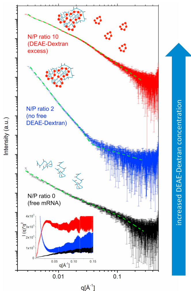
Fig. 4. SAXS data of DEAE-Dextran/mRNA polyplexes with an N/P ratio of 0 (black), 2 (blue) and 10 (red) in HBGx1 buffer (pH 7.2). Green dashed curves are fit models of the respective scattering curves obtained with SASfit using the unified exponential power law from Beaucage [38,39]. Data are shifted vertically for clarity. Kratky plot (bottom left inset plot) was obtained by plotting I(q) \cdot q^2 against q . (For interpretation of the references to colour in this figure legend, the reader is referred to the Web version of this article.)
