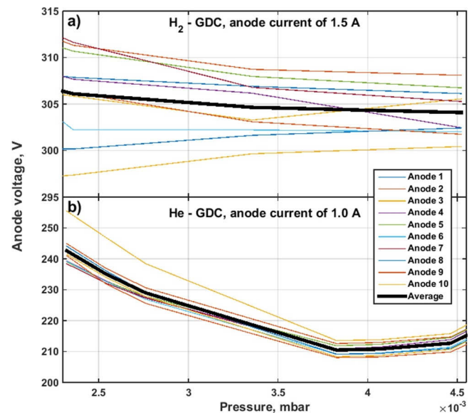
Fig. 2. (a) \text{H}_2 glow discharge anode voltage dependence on neutral gas pressure at anode current of 1.5 A. (b) He glow discharge anode voltage dependence on neutral gas pressure at anode current of 1 A.
