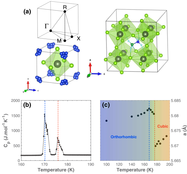
FIG. 1. (a) (Left) Crystallographic structure of MAPbCl 3 in the cubic phase. The Pb site is represented by the grey sphere, the Cl ions are shown in green, and the methylammonium molecules are represented in blue in their disordered state. The top figure shows the high symmetry points in the first Brillouin zone of a primitive cubic lattice. X , M , and R represent \mathbf{Q} = (\frac{1}{2}, 0, 0) , (\frac{1}{2}, \frac{1}{2}, 0) , and (\frac{1}{2}, \frac{1}{2}, \frac{1}{2}) , respectively. (Right) Crystallographic structure of MAPbCl 3 in the orthorhombic phase. In this ordered phase, the H, N, and C atoms forming methylammonium molecules are represented with light blue, dark blue, and dark green spheres, respectively. (b) Heat capacity as a function of temperature for MAPbCl 3 . (c) Temperature dependence of the cell parameter a , measured on BT4 (NIST). The dashed lines indicate the two structural transitions in MAPbCl 3 .
