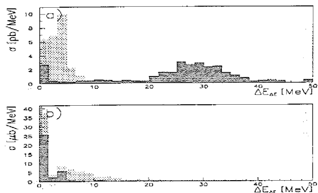
Fig. 3: a) \Delta E_{\Delta E} spectra for kaons and myons, b) \Delta E_{\Delta E} for the background events. The gate for K^+ detection is set to 14 \text{ MeV} \leq \Delta E_{\Delta E} \leq 40 \text{ MeV} .
