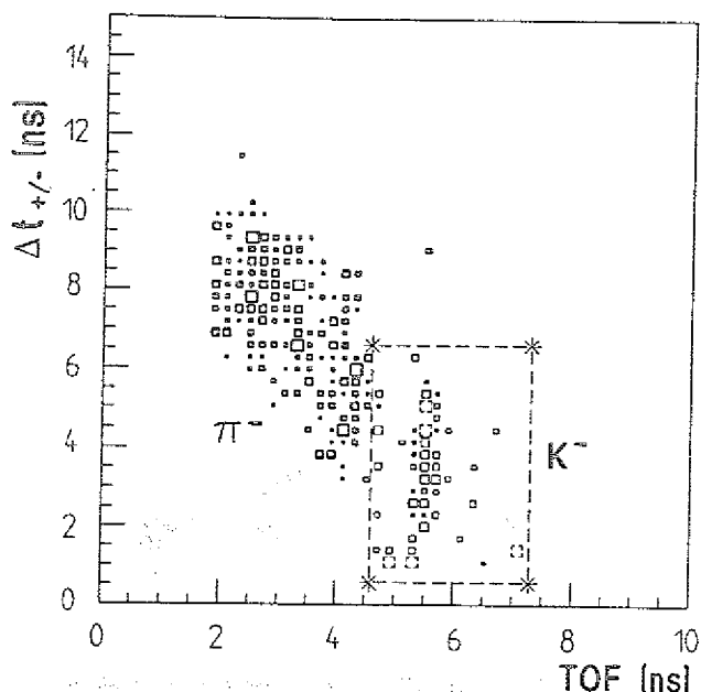
Fig. 2: Simulated TOF spectra of correlated K^+/K^- and K^+/\pi^- events summed over all counters.
