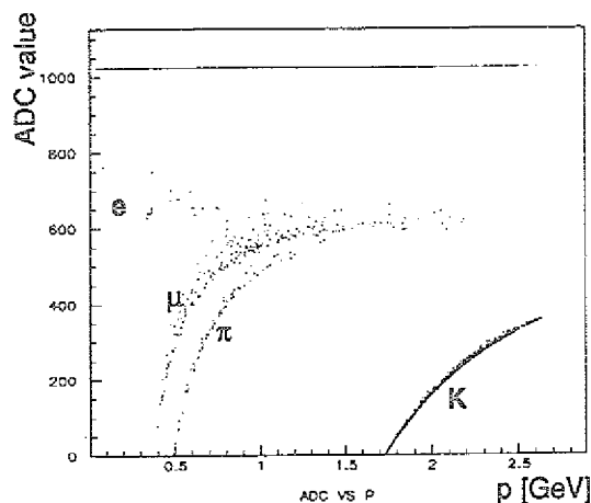
Figure 1: Simulated ADC values
