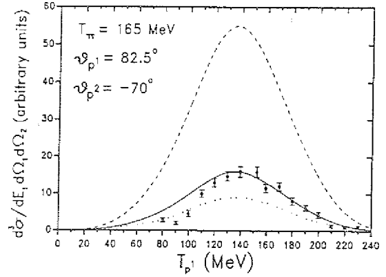
Fig. 2: Threefold differential cross section for the ^{12}\text{C}(\pi^+, pp)^{10}\text{B} reaction as function of the kinetic energy of the proton, which was measured at \theta_{p1} = 82.5^\circ . The angle of the second proton was fixed at \theta_{p2} = -70^\circ . The dashed curve shows the result of our calculation with V_{\Delta N, \Delta N} = 0 , the solid curve the result with V_{\Delta N, \Delta N} \neq 0 . The dotted curve represents the result with V_{\Delta N, \Delta N} \neq 0 and inclusion of distortion effects on the outgoing protons. Our calculation with inclusion of V_{\Delta N, \Delta N} (solid curve) was normalized to the counting rate from ref. [2].
