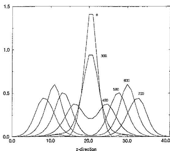
Fig. 2. Cut in the baryon number density along the separation axis for different time steps t
