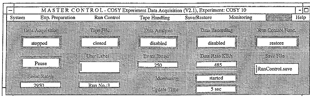
Fig. 1: Main OSF/Motif window of Master Control process
