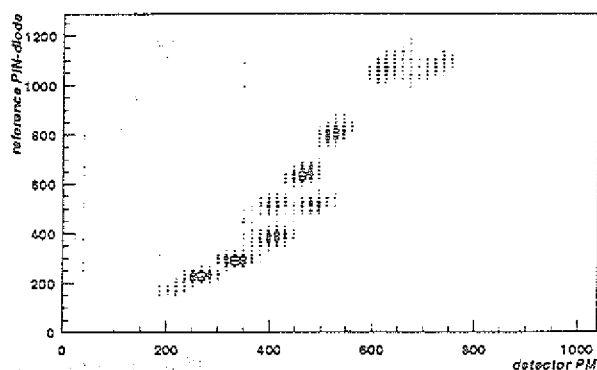
Fig. 3: Correlation plot of laser monitor pulse heights read from Pin 2 and one of the EDDA scintillators showing an irregularity in the ADC of the latter.
