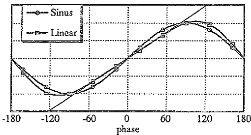
Fig. 1a: sinusoidal and "linearized" voltage
