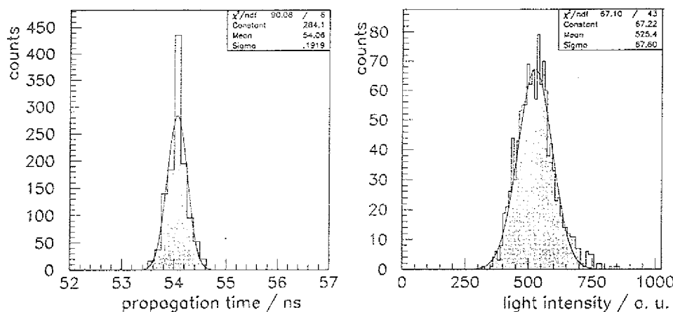
Figure 2: Typical TDC and QDC histograms of one channel. The time resolution is in the order of the intrinsic one of the photomultiplier XP2020.
