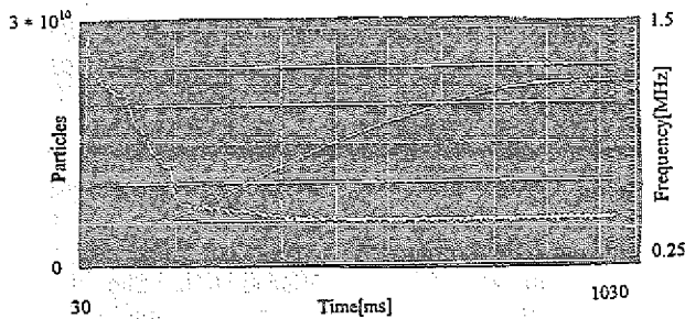
Fig. 1: Number (left scale 5 \cdot 10^9/\text{div} ) and revolution frequency (right scale 0.2 \text{ MHz}/\text{div} ) of the circulating protons dependent on time ( 0.1 \text{ s}/\text{div} ) after the start of the COSY cycle
