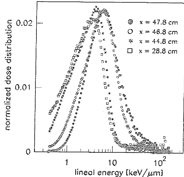
Fig. 1: Microdosimetric dose distributions as a function of depth in water
