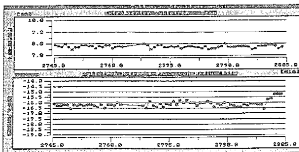
Fig. 2 Display of external beam current (upper trace) and phase (lower trace) over a period of 1 hour
