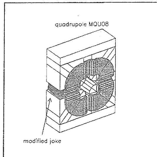
Fig. 1: Quadrupole MQU8 with machined wedge
