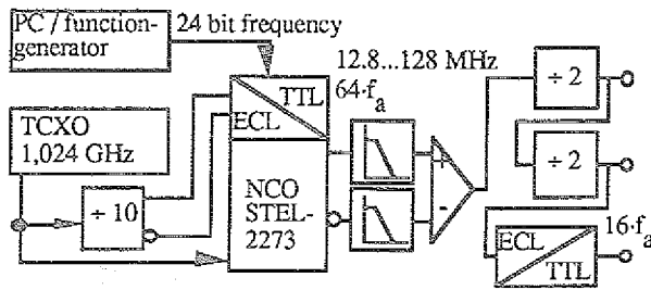
Fig. 4: clock generation with TCXO and NCO
