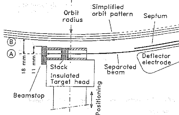
Fig. 1: Simplified representation of the orbit pattern and part of the extraction system. Target head with foil stack in irradiation position
