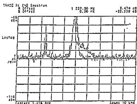
Fig. 4: Schottky scan around the revolution frequency after shaping with 6 kHz noise bandwidth around the 4th harmonic. The noise centre is shifted by +3 kHz.
