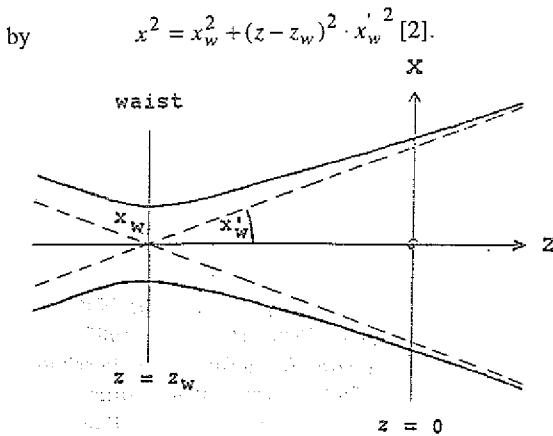
Fig. 1: Beam envelope near the waist. Illustration for the definitions of z_w , x_w , x'_w
