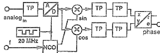
Fig. 3a: Schematic of one digital phase-detector
