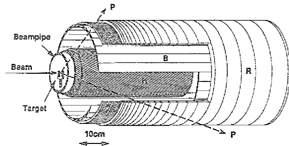
Fig. 1 The EDDA-Detector (not to scale): Target (CH 2 fiber suspended from fork, later polarized atomic beam), Beam pipe (2 mm Al in sensitive region), H Scintillating Fibers wound in opposing helicities, B Scintillator bars, F + R Scintillator semi-rings
