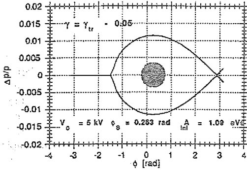
Fig. 2: Bunch and bucket before transition using a single harmonic rf-system.
