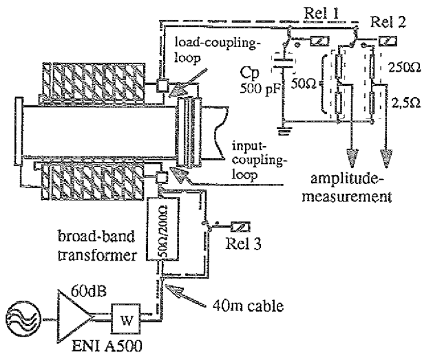
Fig. 4: RF-matching of one Kicker-structure
