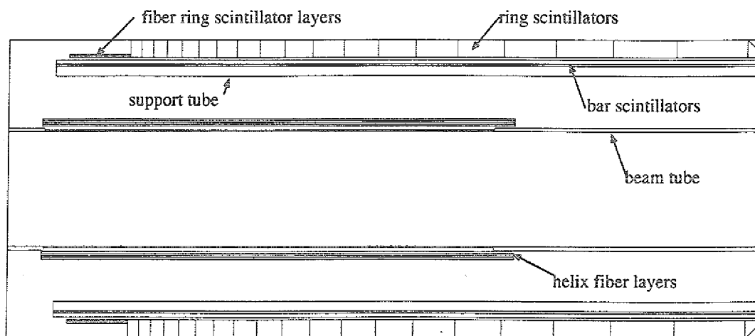
Fig.1 EDDA BSG z,x cross section
