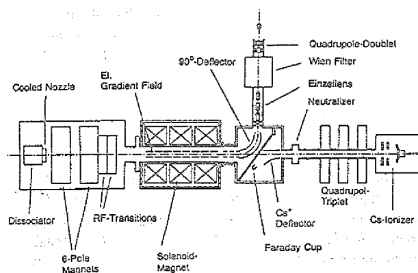
Fig. 1 Schematic of the polarized Source
