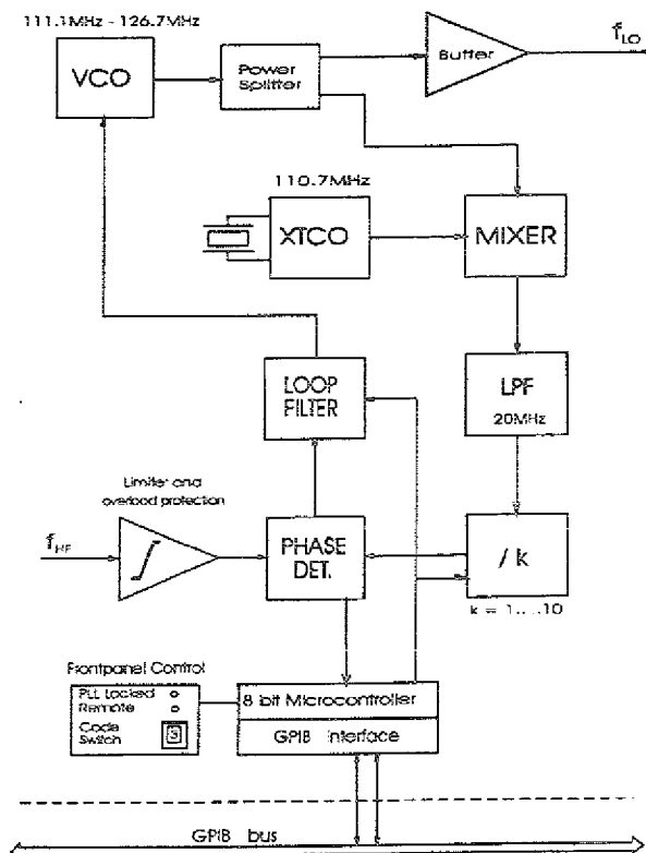
Fig. 1: Block diagram of the tracking LO-synthesizer
