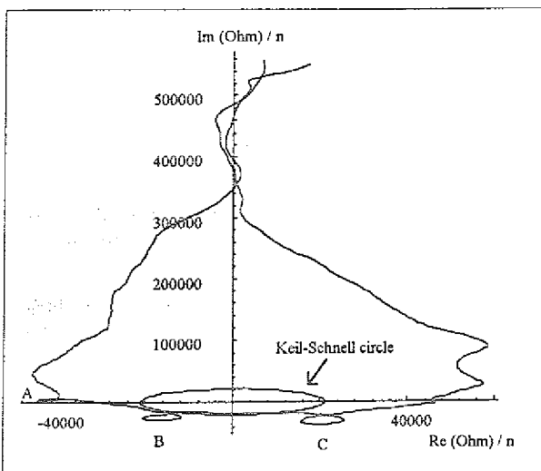
Figure 3: Longitudinal stability diagram of a beam with \approx 2 \cdot 10^{10} protons at 269 MeV/c at the 3rd harmonic, with (dp/p)_{FWHM} = 9 \cdot 10^{-4} . From the stability diagram follows that the coupling impedance is below the theoretical Keil-Schnell limit (ellipse). The loops (marked by "A", "B" and "C") come from tune resonances, as shown by transverse BTF measurements [8].
