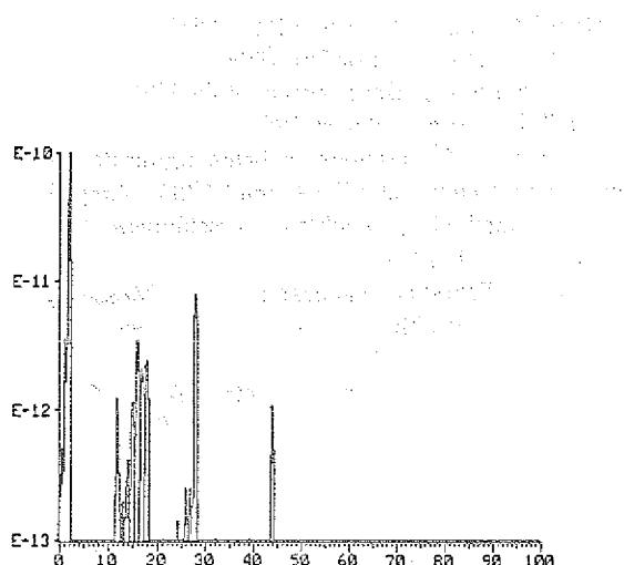
Fig. 1: Residual Gas Spectrum
