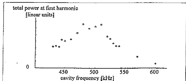
Figure 1: The total power of the beam signal at the first harmonic, measured for different cavity frequencies f_{RF} (revolution frequency f_0 = 451 \text{ kHz} ).
