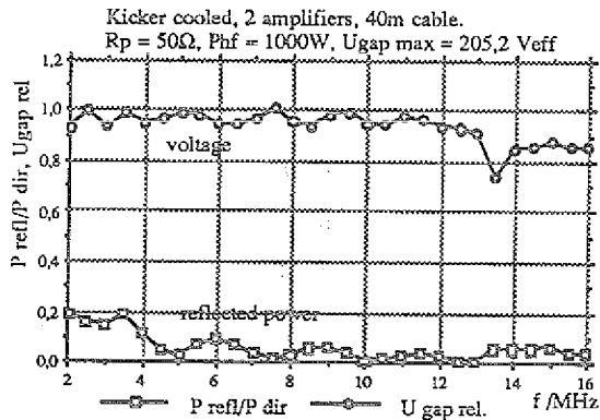
Fig. 5a: Kicker measured in broad-band mode
