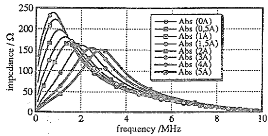
Fig. 7: gap-impedance of the VitroVac®-filled cavity
