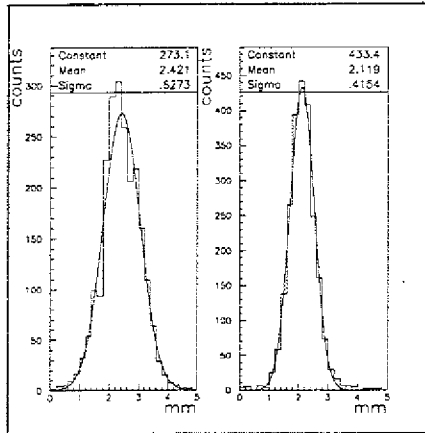
Figure 2: Beamprofile, left: horizontal, right: vertical.
