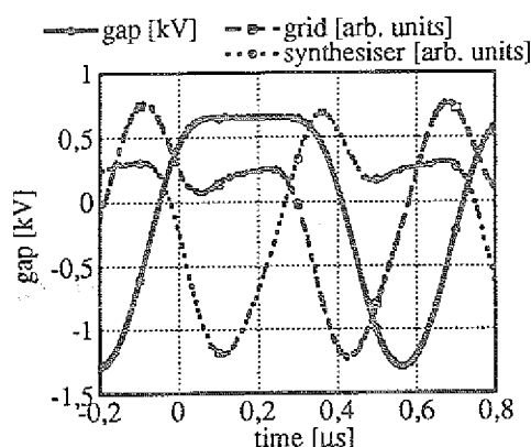
Fig. 9: synthesised voltages for transition
