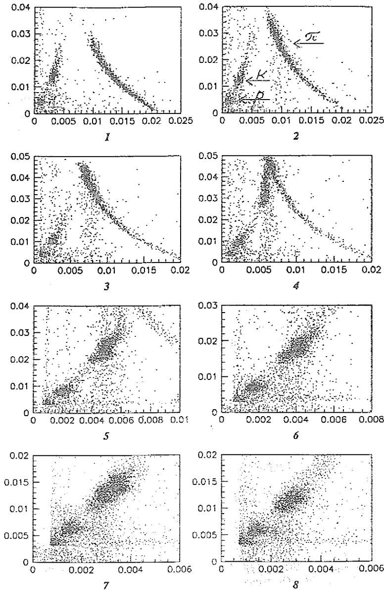
Fig. 3: GEANT simulated energy losses in the counters of the two hodoscope layers (abscissa: 5 mm thick counters of the first layer; ordinate: 20 mm thick counters of the second layer). The plots 1 to 8 correspond to the 8 counters hit by particles with momenta increasing from 250 MeV/c in the first to 600 MeV/c in the eighth counter.
