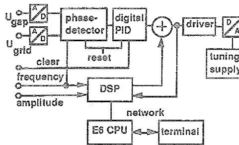
Fig. 2: Digital test system
