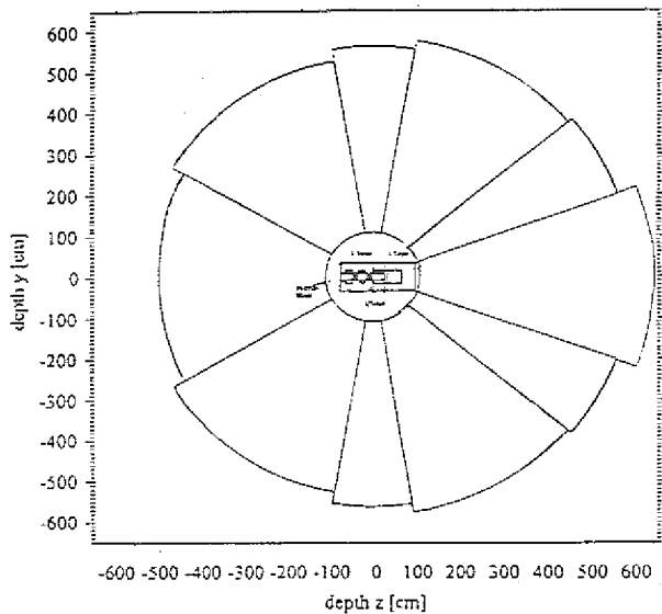
Fig. 6: Resulting shield thicknesses for different angular intervals to get dose rates less than 7.5 \mu\text{Sv/h} outside the shield
