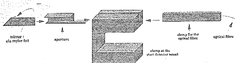
Figure 1: Schematic drawing of the reflector head
