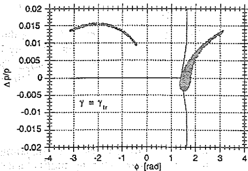
Fig. 3: Bunch and bucket at transition.
