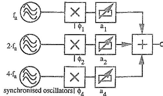
Fig. 2: principle of higher harmonic synthesis
