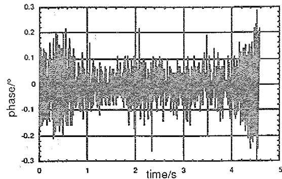
Fig. 5c: phase deviation, first ramp
