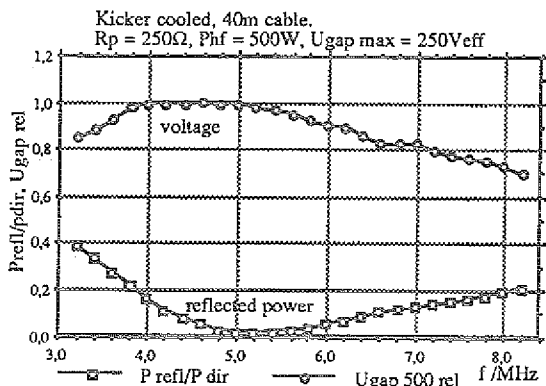
Fig. 5b: Kicker measured in narrow-band mode
