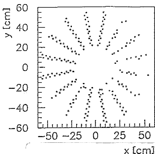
Fig. 3: Central projection of the overlap regions of the start ring on the stop detector from the target point
