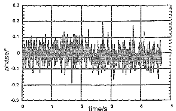
Fig. 5f: phase deviation, consecutive ramps
