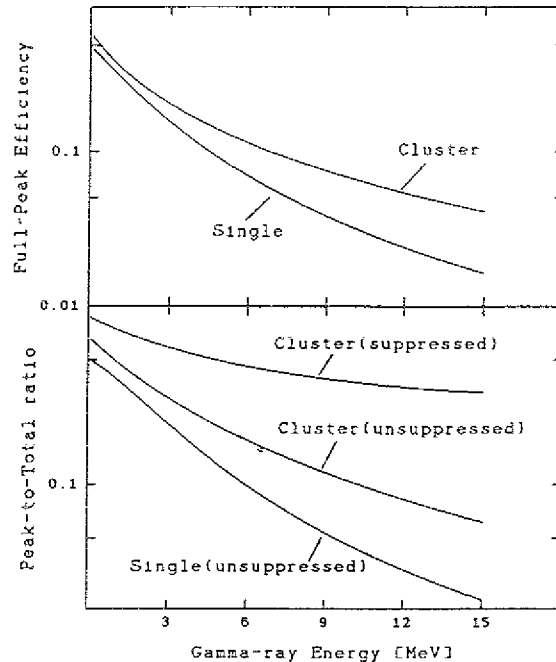
Fig. 1: Calculated full-peak efficiency and P/T ratio of a single semi-hexagonal tapered detector and the cluster of 7 such detectors plotted against the energy of the incident \gamma -rays.
