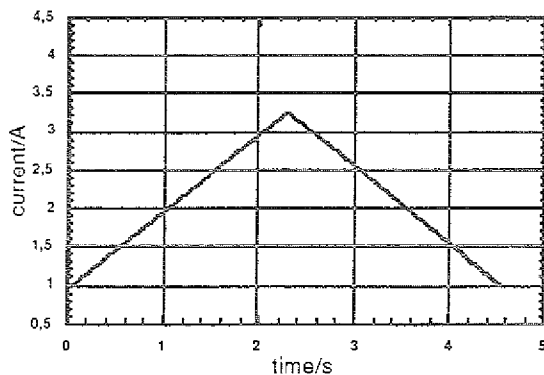
Fig. 5a: estimated current (DSP), first ramp
