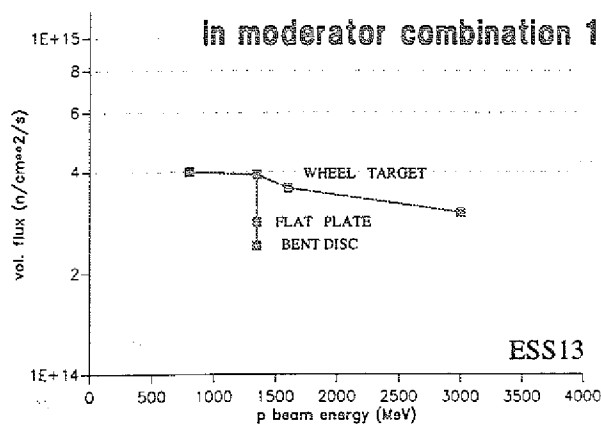
Fig. 4: Thermal neutron flux in a fast moderator for different target systems
