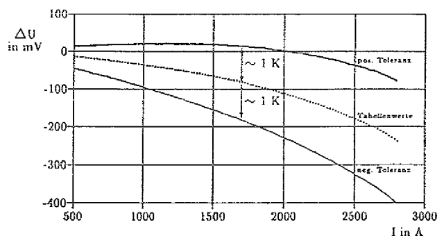
Fig. 3: Voltage deviations and threshold temperature versus current
