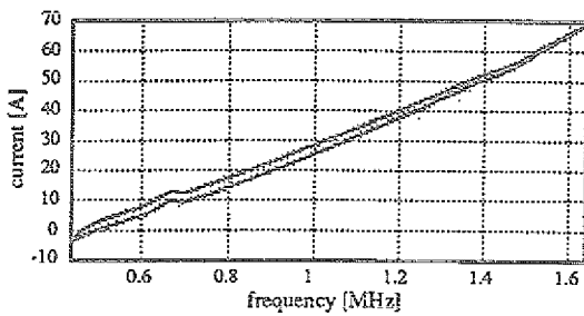
Fig. 1a: Tuning current vs. frequency, "normal" rf-amplitude (DAC-Voltage 4.0 V, COSY-GUI)
