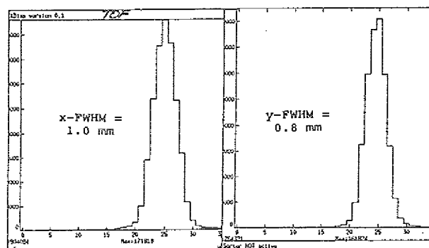
Fig. 2: Beam size on the Target in TOF as measured on a strip detector (Erlangen) with a resolution of 0.2 mm at p = 1.09 \text{ GeV}/c .
