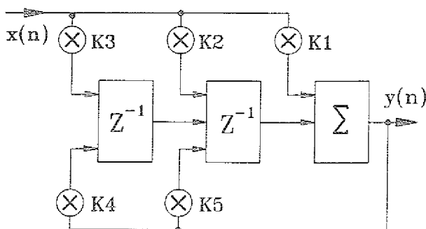
Fig. 1: Butterworth Filter in Z-notation
