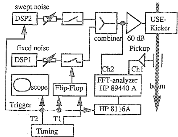
Fig. 6: experimental set-up for first experiments
