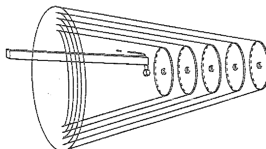
Figure 2: Target and decay spectrometer
