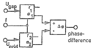
Fig. 3b: Combination of two digital phase-detectors
