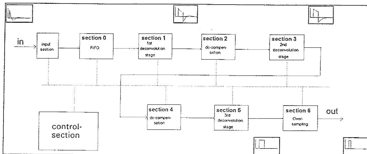
Figure 1: Block diagram of the ASDSP
