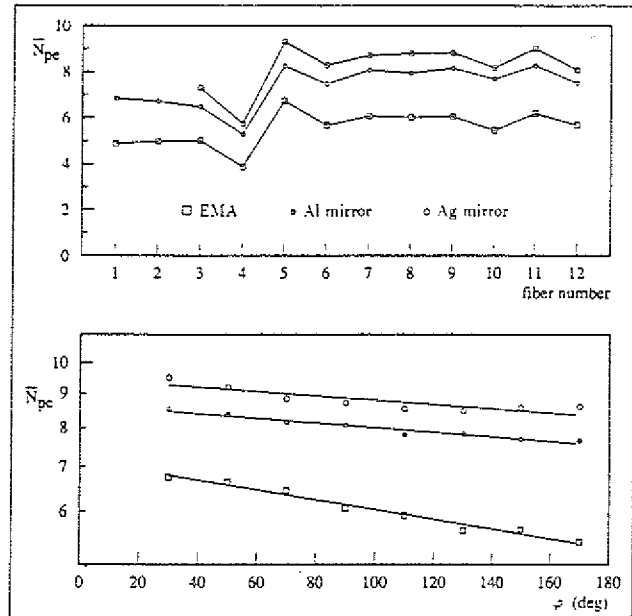
Fig. 2: Top: Average number \bar{N}_{pe} of photoelectrons vs. fiber number for different designs of the far fiber ends. Bottom: Attenuation of light along a fiber; \Delta\varphi = 90^\circ corresponds to \Delta s = 27 cm.
