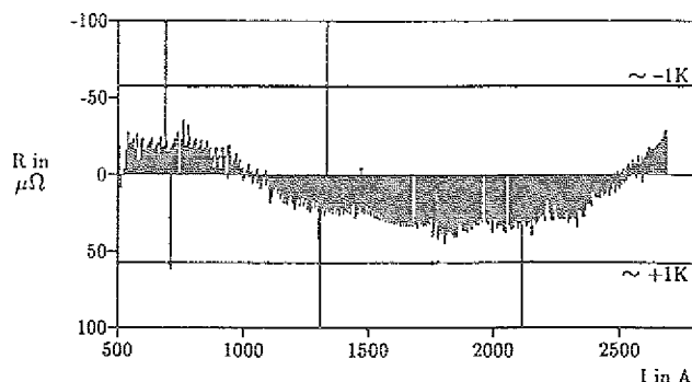
Fig. 2: Deviation between measured and calculated coil resistance
