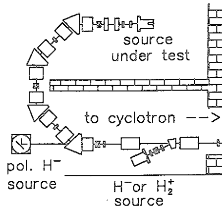
Fig. 1: New source locations at the cyclotron beamline
