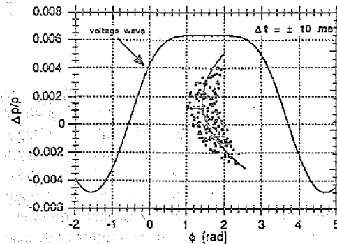
Fig. 6: At transition. The HHS is switched on for 20 ms.
