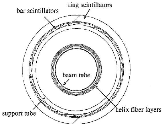
Fig.2 EDDA BSG -x,y cross section
