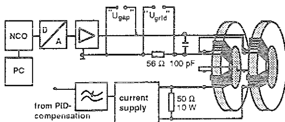
Fig. 4: Test system with simulated cavity
