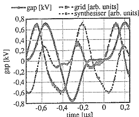
Fig. 10: synthesised voltages for stochastic cooling
