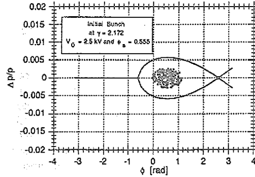
Fig. 5: Bunch and bucket before transition. HHS off.
