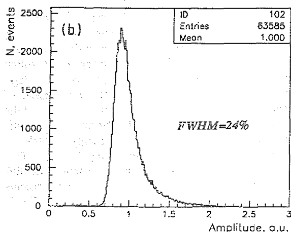
Fig. 2: Amplitude spectra measured with the hodoscope modules of 5 mm (a) and 20 mm thickness (b).
