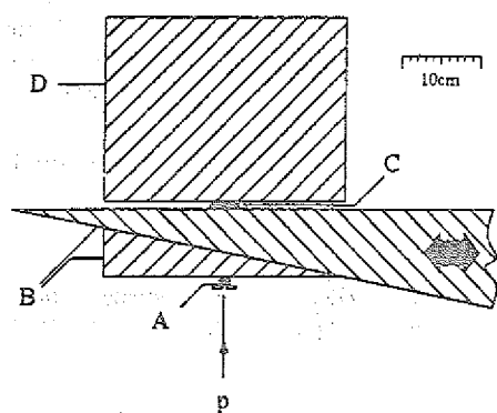
Fig.1: Basic experimental setup with a solid phantom wedge.
