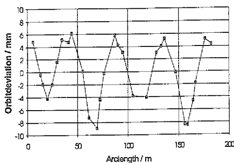
Orbit for magnetic fields raised by 0.05%
