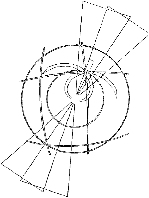
Fig.3: eventplot in theta-phi-projection, elastic scattering
