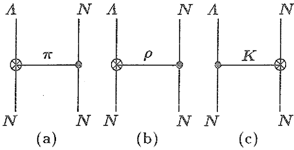
Fig. 1. (a) \pi exchange contribution to the reaction NN \rightarrow \Lambda N . (b) \rho exchange contribution. (c) K exchange contribution. The \otimes indicates the weak vertex.
