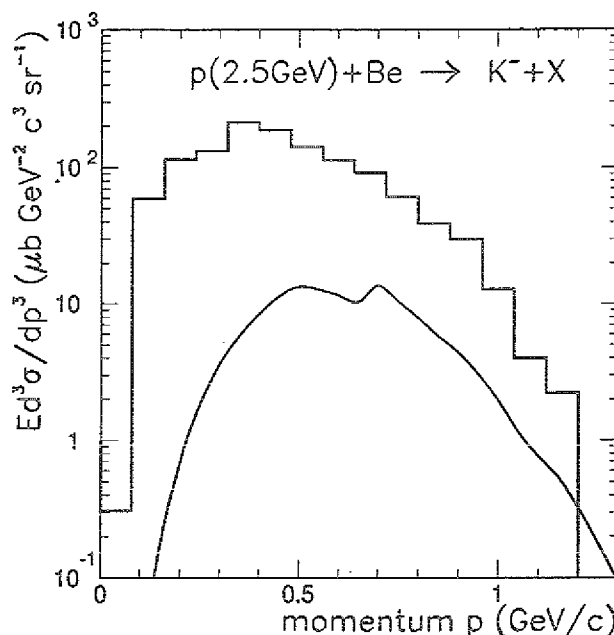
Fig. 1: Folding-model (curve) and ROC-model (histogram) predictions for the K^- -momentum spectra produced in p+Be collisions at T_p = 2.5 GeV, integrated over kaon-emission angles \theta \leq 10^\circ .
