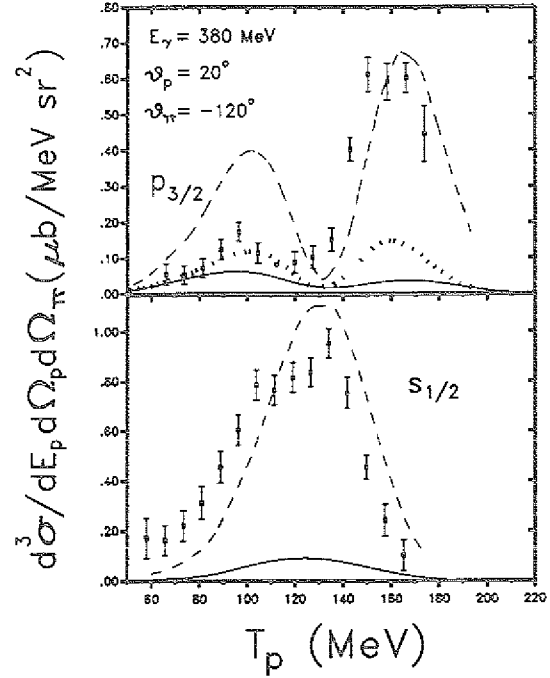
Fig. 1: Threefold differential cross section for the ^{12}\text{C}(\gamma, p\pi^-)^{11}\text{C} reaction as function of the kinetic energy of the outgoing proton. The data are taken from ref. [5]. The upper part of the figure shows the photon absorption on a p_{3/2} neutron, the lower part the absorption on a s_{1/2} neutron. The solid curves show the results of our calculations, the dashed curves the results of ref. [3] including \Delta contributions and Born terms. The dotted curve represents the result of [3] with \Delta contribution alone.
