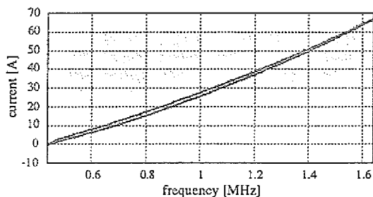
Fig. 7b: DAC: 9.0 V, with filter
