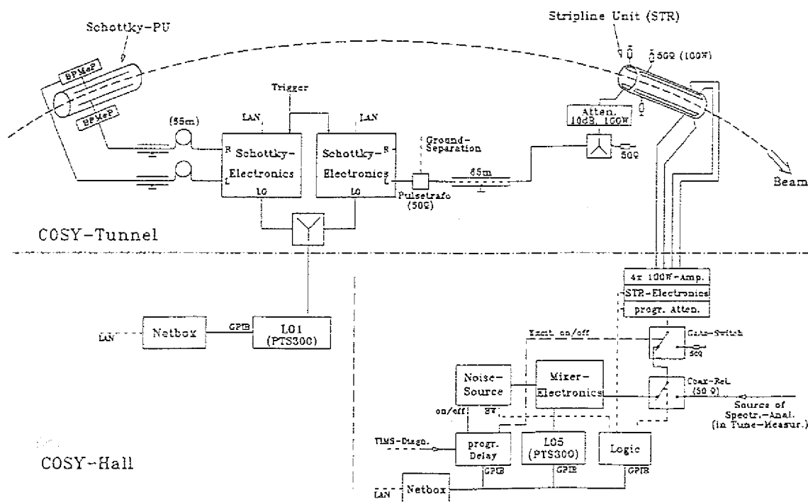
Fig. 1: Blockdiagram of the BTF-measurement system
