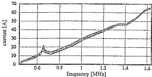
Fig. 1b: "maximum" rf-amplitude (DAC: 9.9 V)
