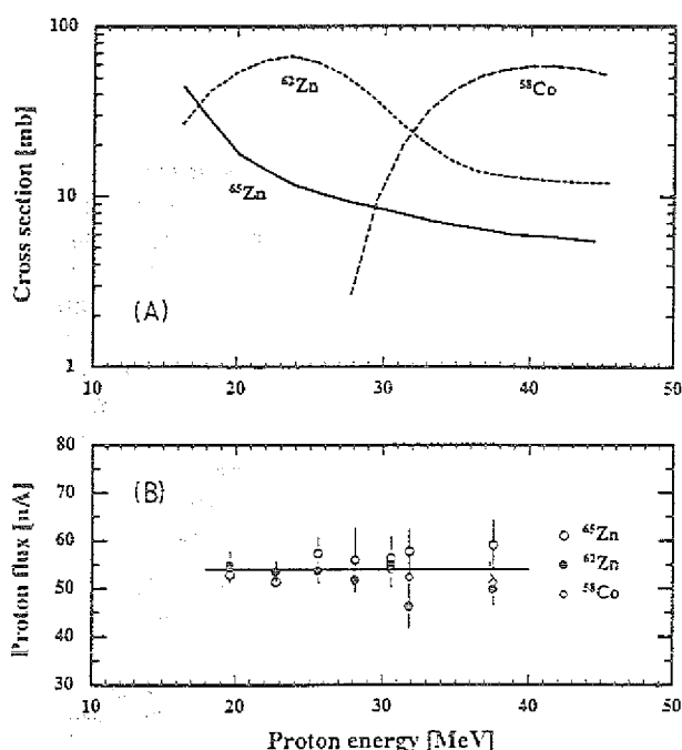
Fig. 4: (A) Excitation functions for the formation of ^{65}\text{Zn} , ^{62}\text{Zn} and ^{58}\text{Co} in proton irradiation of ^{nat}\text{Cu} , used for beam monitoring in the energy range of 16 to 45 MeV. (B) Proton current values determined via the three monitor reactions at different projectile energies.
