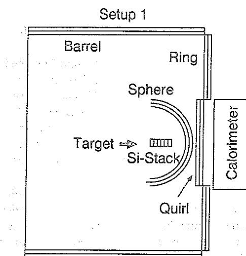
Fig. 1: Experiment setup 1 with scintillator calorimeter
