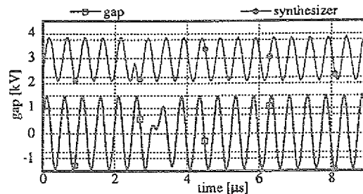
Fig. 8a: phase jump 180° with VitroVac-cavity
