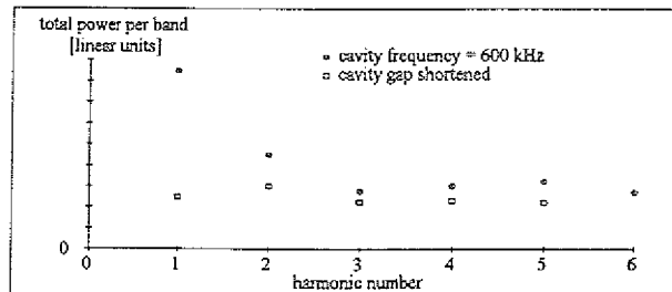
Figure 2: The total power of the Schottky bands at lower harmonic numbers ( f_{RF} = 600 \text{ kHz} , f_0 = 451 \text{ kHz} ).
