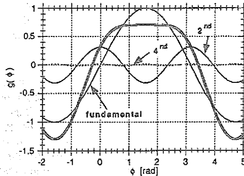
Fig. 1: Single rf-wave forms in comparison to the resultant sum wave form of the three octave rf-system, eq. 1.
