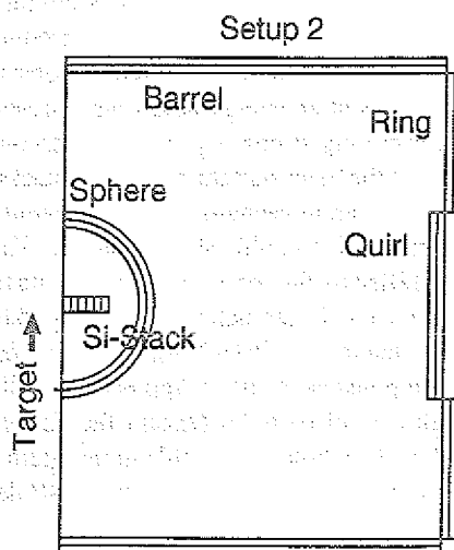
Fig. 2: Experiment setup 2 (time-of-flight setup)
