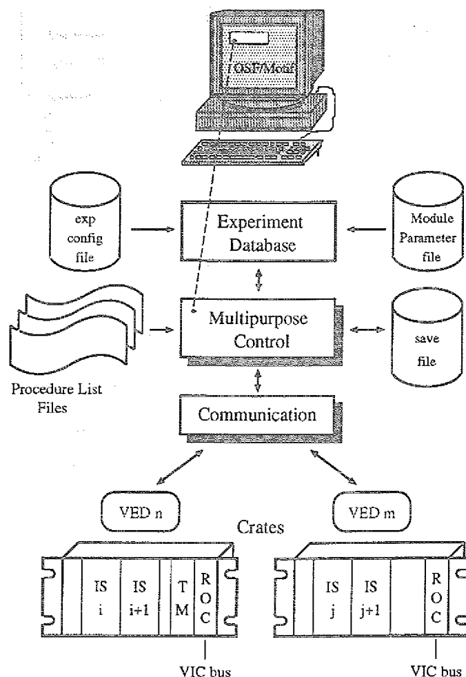
Fig. 2: Structure of the Multipurpose Control process
