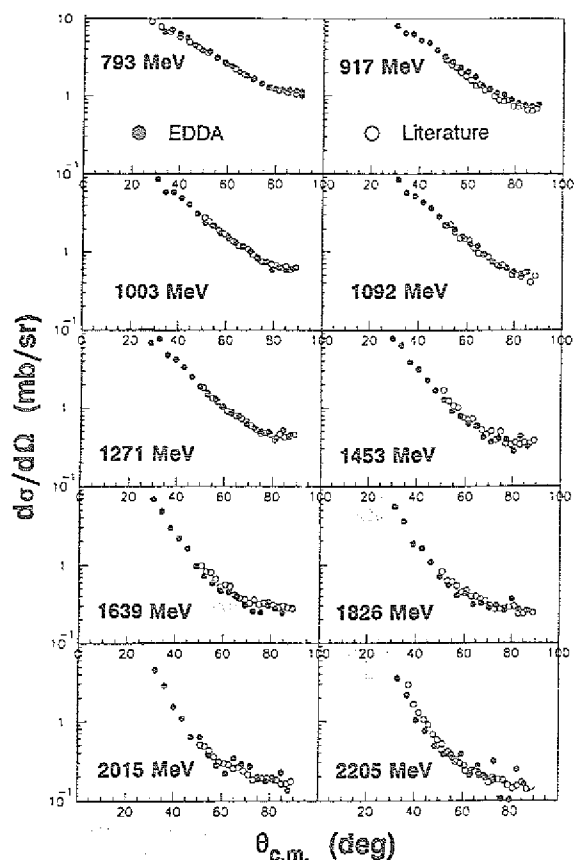
Fig. 3 Angular distributions of elastic proton-proton scattering events as obtained (preliminary, analysis uncomplete) by EDDA and as available from the literature for the bombarding energies (lab) indicated. The EDDA data were normalized as a function of bombarding energy using the \delta -electrons recorded in PIN diodes as luminosity signal.
