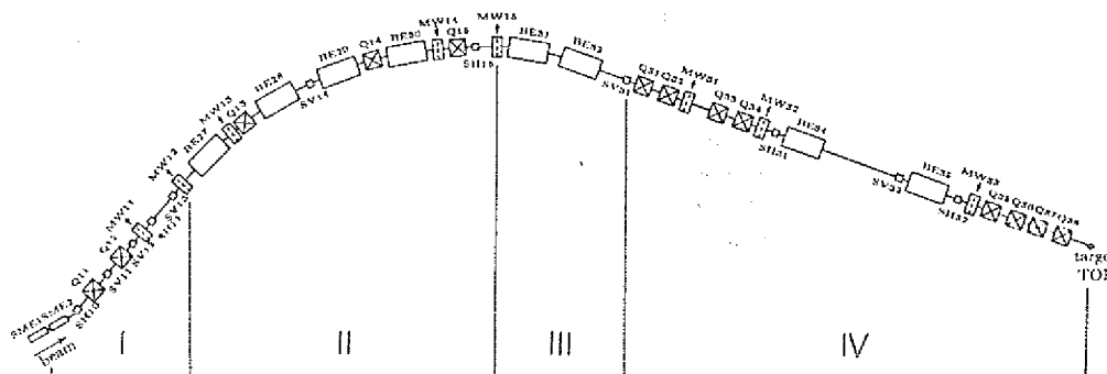
Fig. 1: The four sections in the extraction beam line from COSY to the TOF experiment with dipoles (BE), quadrupoles (Q), steerers (S) and multiwire chambers (MW).
