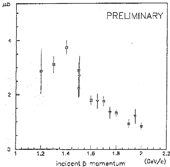
Figure 3: Excitation curve for the reaction \bar{p}p \rightarrow \phi\phi from a broad scan over the mass range accessible at LEAR. These data are corrected for the unseen decay modes of the \phi .
