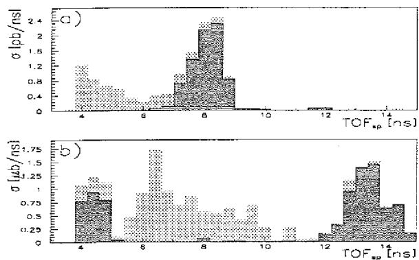
Fig. 2: a) TOF spectra for kaons and myons, b) TOF spectra for the background events. The gate for K^+ detection is set to 7.1 \text{ ns} \leq \text{TOF}_{\text{sp}} \leq 9.0 \text{ ns} .
