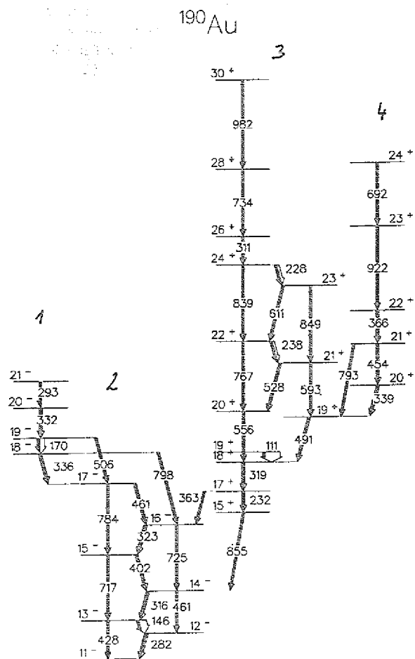
Figure 1: Partial level scheme of ^{190}\text{Au}
