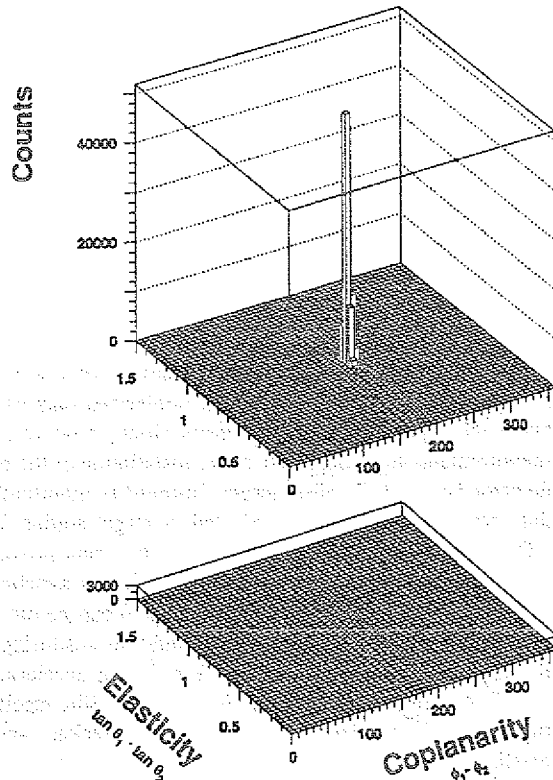
Fig. 2 Kinematic distribution of EDDA events as obtained with a CH 2 (upper part) and with a carbon (lower part) fiber target ( T_p = 793 MeV)
