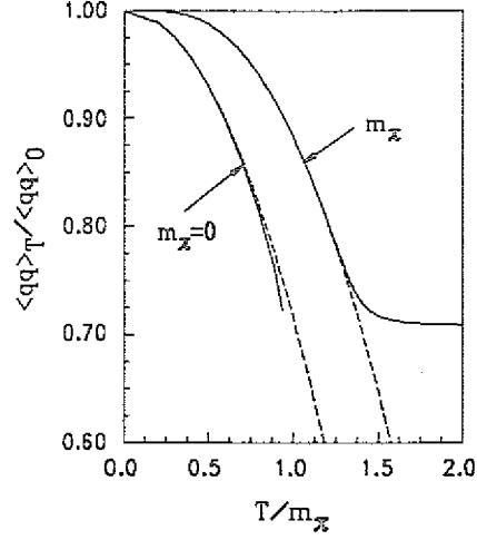
Fig. 1: Temperature dependence of the chiral condensate from an interacting pion gas. The full lines denote the results with \lambda = f_\pi^{-2}/4 both for the physical pion mass and in the chiral limit. The dashed lines give the corresponding results with \lambda/4 .
