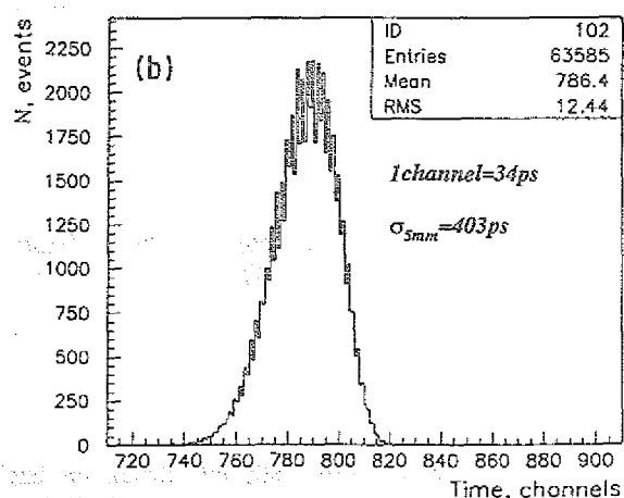
Fig. 1: Time spectra measured for coincidences between the hodoscope modules: a) Spectrum for 20 mm thick start module and 20 mm thick stop module; b) Spectrum for 5 mm thick start and 20 mm thick stop module. Single counter RMS values are given.
