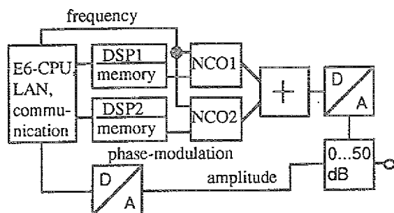
Fig. 1: Layout of the noise generator
