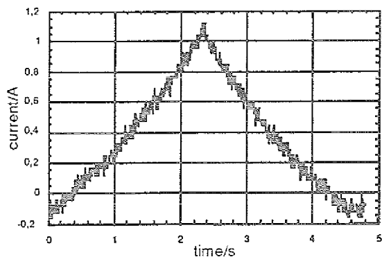
Fig. 5b: output signal PID-compensation, first ramp
