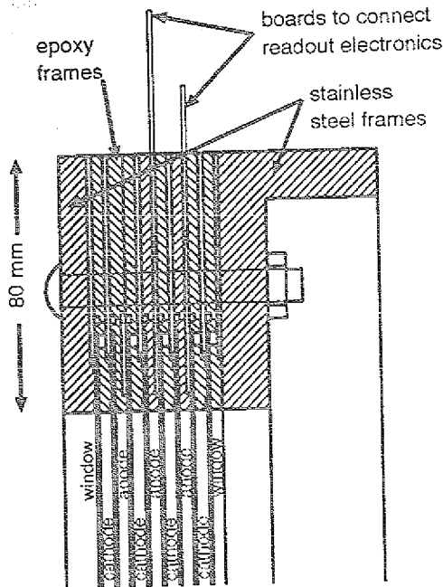
Fig. 1: Drawing of the design of the multiwire chamber MWC1. A cut through the upper part of the frame is shown.
