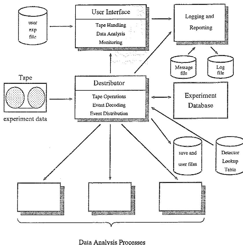
Fig. 3: Structure of the Offline Eventdistributor
