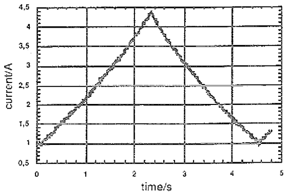
Fig. 5d: estimated current (DSP), consecutive ramps
