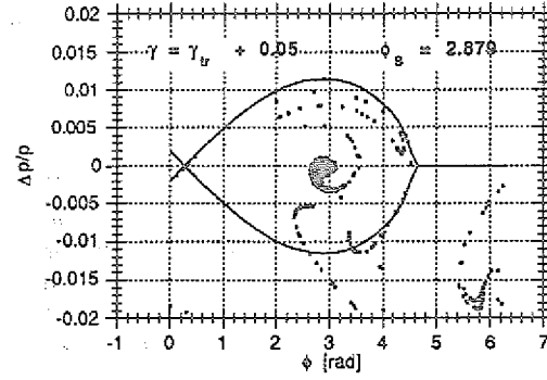
Fig. 4: Bunch and bucket after transition crossing.
