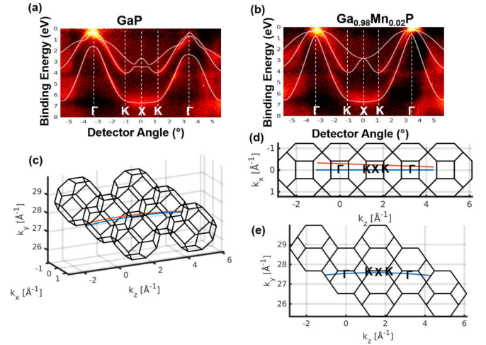
FIG. 7. (a, b) Curves that are the results of the free-electron final-state calculations are superposed on the corrected experimental HARPES data for GaP and \text{Ga}_{0.98}\text{Mn}_{0.02}\text{P} , respectively. (c–e) HARPES paths in k -space for the optimized experimental geometries determined from the FEFS calculations: GaP, red line; \text{Ga}_{0.98}\text{Mn}_{0.02}\text{P} , blue line. The paths are shown in three different perspectives. \text{Ga}_{0.98}\text{Mn}_{0.02}\text{P} is very close to the ideal geometry of Fig. 5. The red and blue lines overlap in (e).
