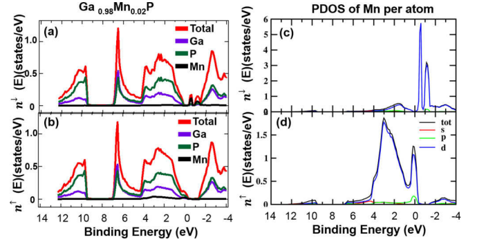
FIG. 9. Calculated spin-resolved element- and orbital-projected DOS for \text{Ga}_{0.98}\text{Mn}_{0.02}\text{P} , with Ga (purple), P (green), and Mn (black) contributions indicated: (a) spin-down; (b) spin-up. Calculated spin-resolved projected DOS for Mn alone in \text{Ga}_{0.98}\text{Mn}_{0.02}\text{P} , with s , p , and d contributions indicated: (c) spin-down; (d) spin-up.
