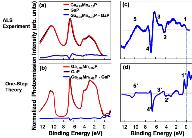
FIG. 8. (a) Experimental angle-integrated valence-band spectra for GaP and \text{Ga}_{0.98}\text{Mn}_{0.02}\text{P} , including their difference curve. (b) Theoretical spectra obtained using one-step theory calculations and their difference. (c, d) Intensity difference spectra between \text{Ga}_{0.98}\text{Mn}_{0.02}\text{P} and GaP for the experimental data (c) and the one-step theory results (d).
