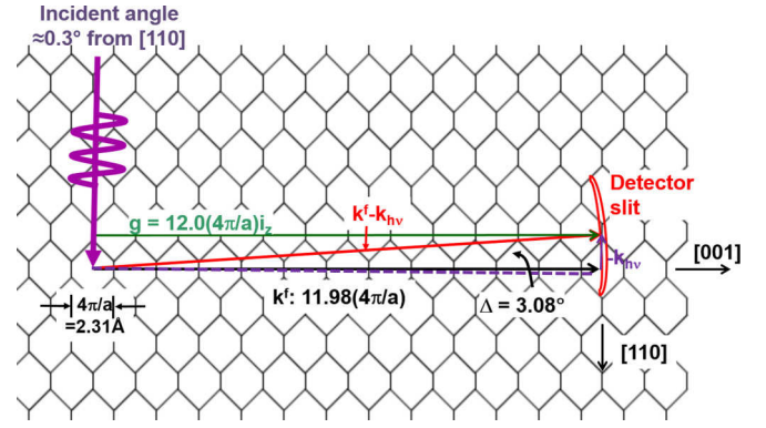
FIG. 5. The experimental geometry of the HARPES measurement in an extended zone picture, with various key vectors and angles shown.
