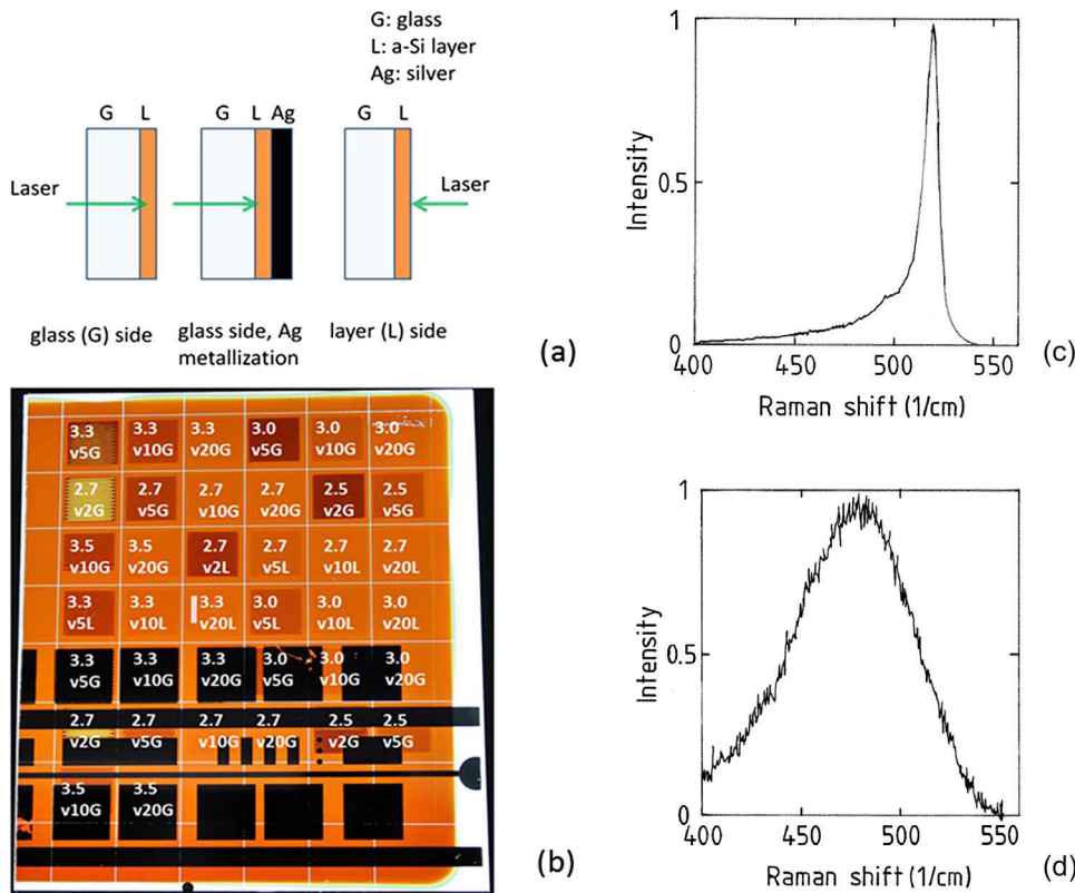
FIG. 1. Schematic setup for laser treatment of the a-Si:H layer on glass (a), transmitted light image of glass plate L24 coated with 0.3 μm a-Si:H and 0.05 μm a-Si:D, scanned at various laser power and scan speed values (see text) (b), Raman scattering spectrum of crystallized silicon (in field 3.3/v5G) (c) and of amorphous silicon (in field 3.3/v10G) (d).
