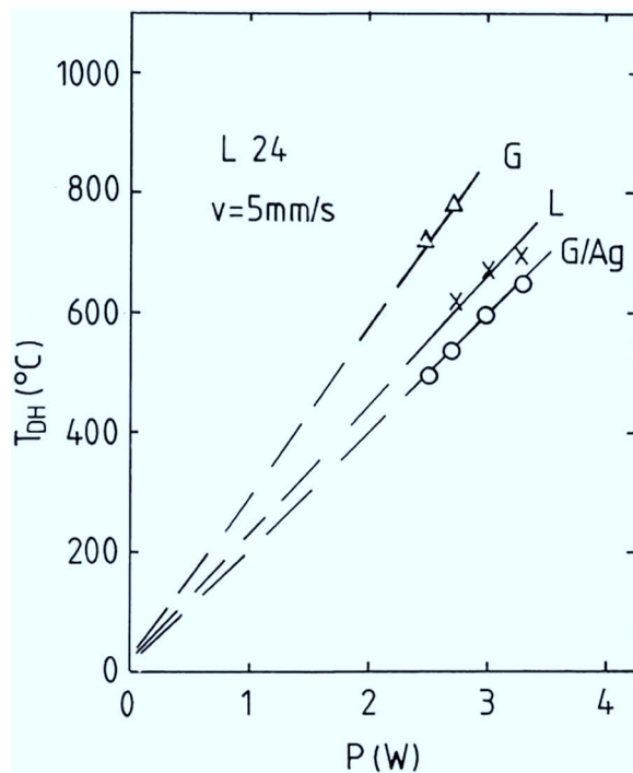
FIG. 9. Temperature T_{DH} in the laser spot as a function of (nominal) laser power P at a scan speed v = 5 \text{ mm/s} for sample L24 at treatment from the a-Si:H layer (L) and glass (G) sides, and at glass side treatment of an a-Si:H film underneath 0.7 \mu\text{m} silver metallization (G/Ag).
