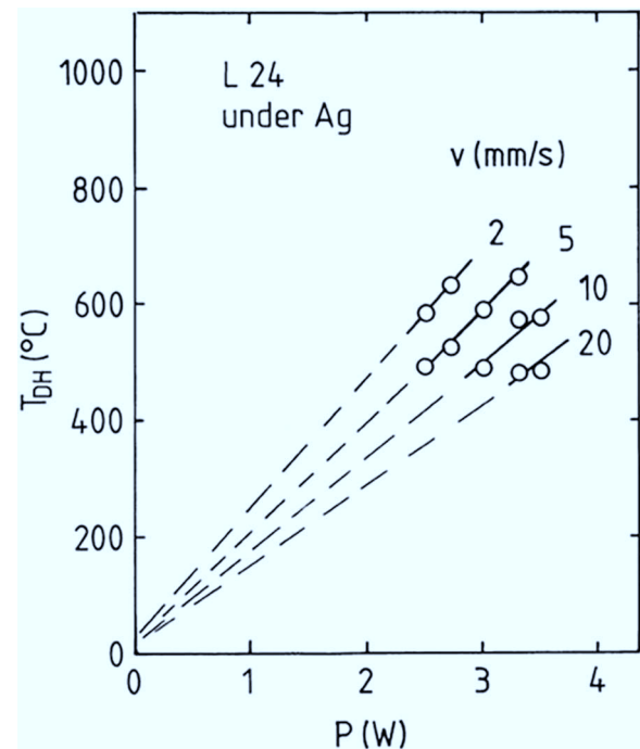
FIG. 10. Temperature T_{DH} in the laser spot underneath a 0.7 \mu\text{m} silver contact film as a function of laser power P (sample L24) for various scan speeds v . Dashed lines indicate extrapolation to T = 20 °C for P = 0 \text{ W} .
