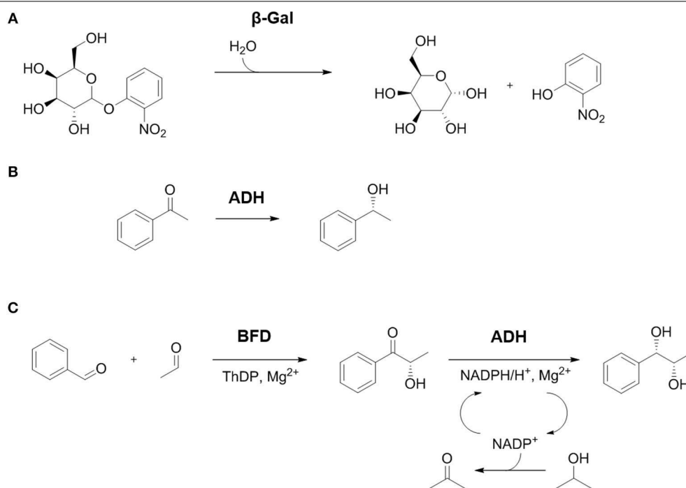
FIGURE 1 | Overview of the studied reactions. (A) Hydrolysis of o-Nitrophenyl-β-D-galactopyranoside (ONPG) by β-Gal yields the monosaccharides galactose and o-nitrophenol. (B) Activity of ADH can be determined by enantioselective reduction of acetophenone to (R)-phenylethanol. (C) The combination of BFD and ADH in a 2-step cascade reaction. Carboligation of the educts benzaldehyde and acetaldehyde catalyzed by BFD yields the intermediate (S)-2-hydroxy-1-phenyl-propanone ((S)-HPP), which can be further reduced to the product (1S,2S)-1-phenylpropane-1,2-diol ((S,S)-PPD) by ADH. The redox equivalents are delivered by the cofactor NADPH that is oxidized to NADP + . For in situ regeneration of NADPH 2-propanol was added in excess which is oxidized to acetone by the same ADH.
