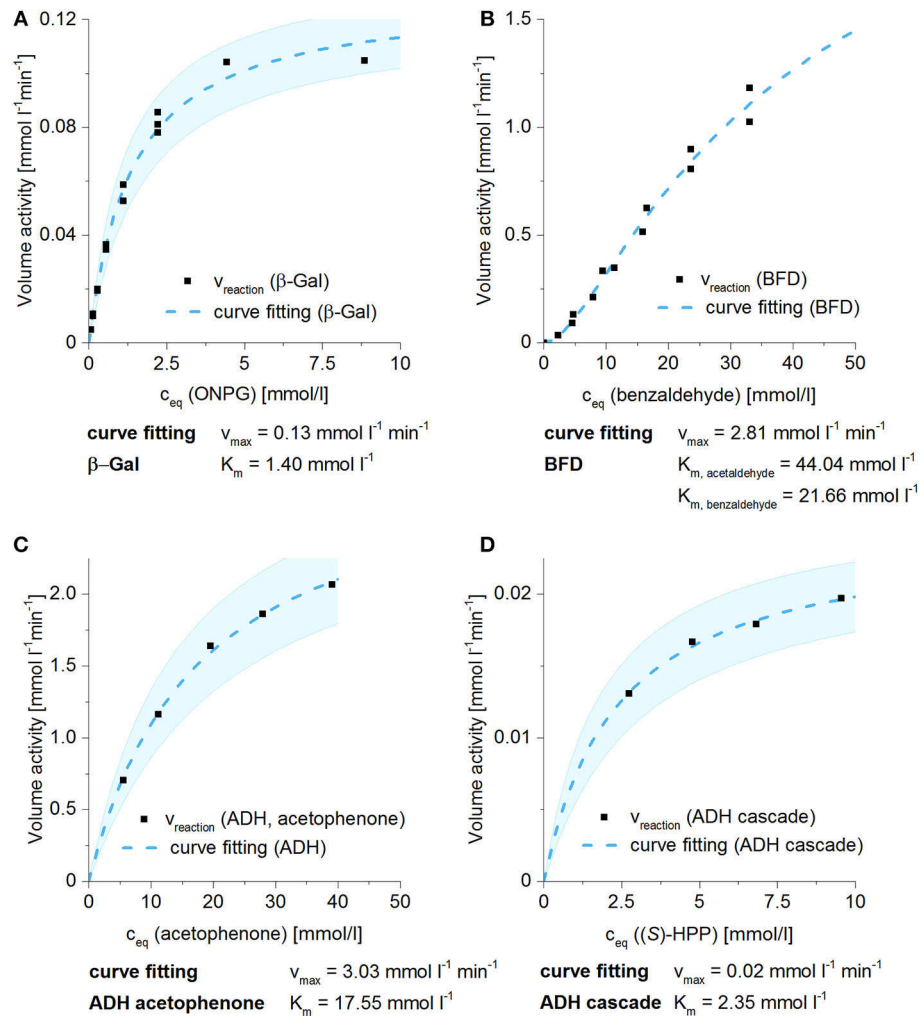
FIGURE 3 | Michaelis–Menten kinetics of the investigated biocatalytic reactions with freely dissolved enzymes. Kinetic parameters v_{\max} and K_m were calculated by fitting the data to the Michaelis–Menten function, which is shown including 95% confidence bounds. In the whole figure, each data point represents one sample. (A) \beta -Gal kinetics for the cleavage of ONPG at pH 4.6 ( n = 3 separate runs). (B) BFD kinetics for the carbonylation of benzaldehyde and a respective 2.5-fold excess of acetaldehyde ( n = 2 separate runs). Estimation of the confidence bounds was omitted because of limited data for substrate excess. (C) ADH kinetics for the reduction of acetophenone. (D) ADH kinetics for the reduction of (S)-HPP, which was previously synthesized by BFD. For ADH kinetics, data points were generated in one batch due to shortage of the enzyme.
