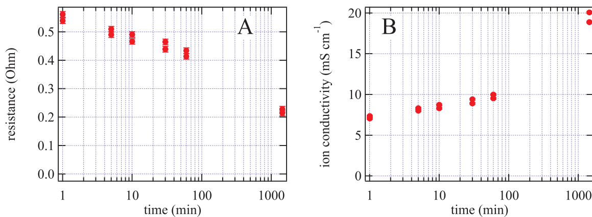
Fig. 8. Online-checked resistance of the membrane plotted against doping time (A) and the resulting membrane conductivity, based on ex-situ measured thickness data (B); the first data point was obtained after 1 min.
