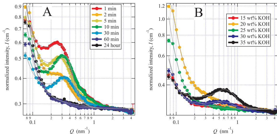
Fig. 3. SANS scattering data for the PBI membrane, the colored lines are to guide the eye, and the grey lines are the fits to the data using Eq. (2) (color available online). Graph A. SANS data as a function of doping time using a 25 wt% KOH doping solution. The diffraction peak in the 30 min data corresponds to 16 nm structures and the peak for 1 min corresponds to 20 nm structures. The PGAA data for the samples shown in this graph are given in Fig. 2 A. Graph B. SANS data as a function of KOH doping solution concentration (doping time: 24 h). The strong correlation peak in the 30 wt% and 35 wt% occurs for a nano-structure size of about 11 nm. The 25 wt% and 20 wt% KOH doped samples show an increased forward scattering presumably due to the formation of larger domains with increased D 2 O uptake/swelling. The PGAA data for the samples shown in this graph are given in Fig. 2B.
