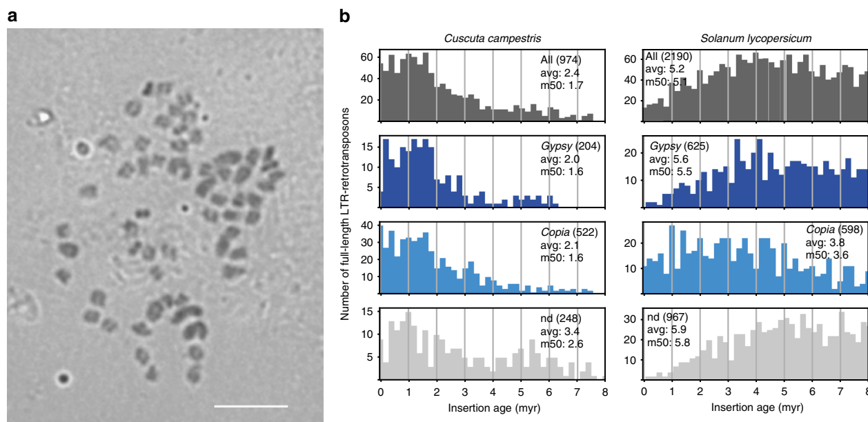
Fig. 2 Genome features. a Feulgen-stained metaphase chromosomes of C. campestris ( 2n = 56 ). The scale bar represents 10 μm. b Insertion age distribution of C. campestris full-length LTR retrotransposons in comparison to tomato ( Solanum lycopersicum ) as another Solanales representative. Insertion events of long terminal repeat (LTR) retrotransposons were dated by comparing the divergence between the 5' and 3' long terminal repeats 61 . A random mutation rate of 7 \times 10^{-9} was used to convert the sequence divergence into age 62 (in million years)
