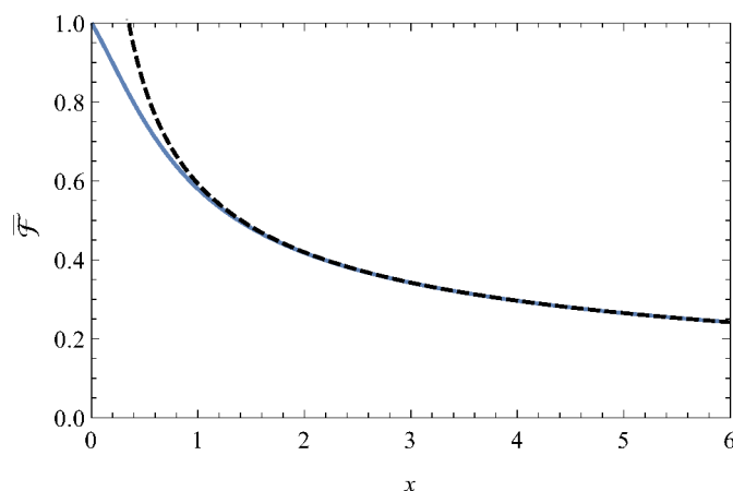
Figure 5: Solid line: \tilde{\mathcal{F}} = (\mathcal{F}_0 + \mathcal{F}_\infty)/2 as obtained from numerical solutions to Eqs. (31) and (32); on this scale, the approximate formula in Eq. (33) is indistinguishable from the numerics. Dashed line: the asymptotic formula 0.5927/\sqrt{x} , as obtained from Eq. (33) at large x , is a good approximation for x > 1 .
