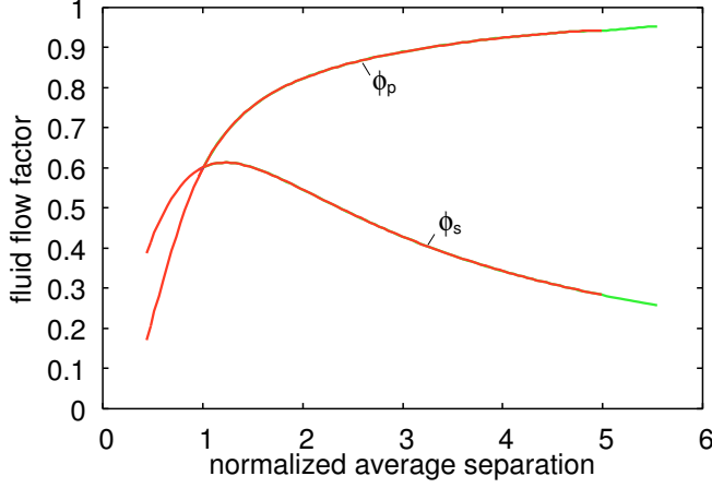
Figure 4. Fluid pressure flow factor \phi_p and shear stress flow factor \phi_s as functions of average separation normalized by h_{rms} . (The green tails to be removed! or put the both curves in black.)
