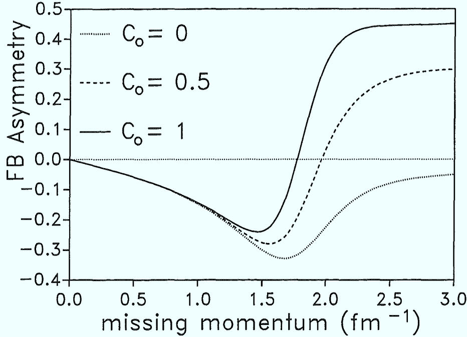
Figure 5.12: The forward-backward asymmetry A_{FB}(p_m) as defined in (5.35) is shown for hard core correlations, C_o = 1 , (solid line), soft core correlations, C_o = 0.5 , (dashed line), and no correlations at all, C_o = 0 , (dotted line). The other ground state parameters are R_o = 1.29\text{fm} and r_c = 0.5\text{fm} .
