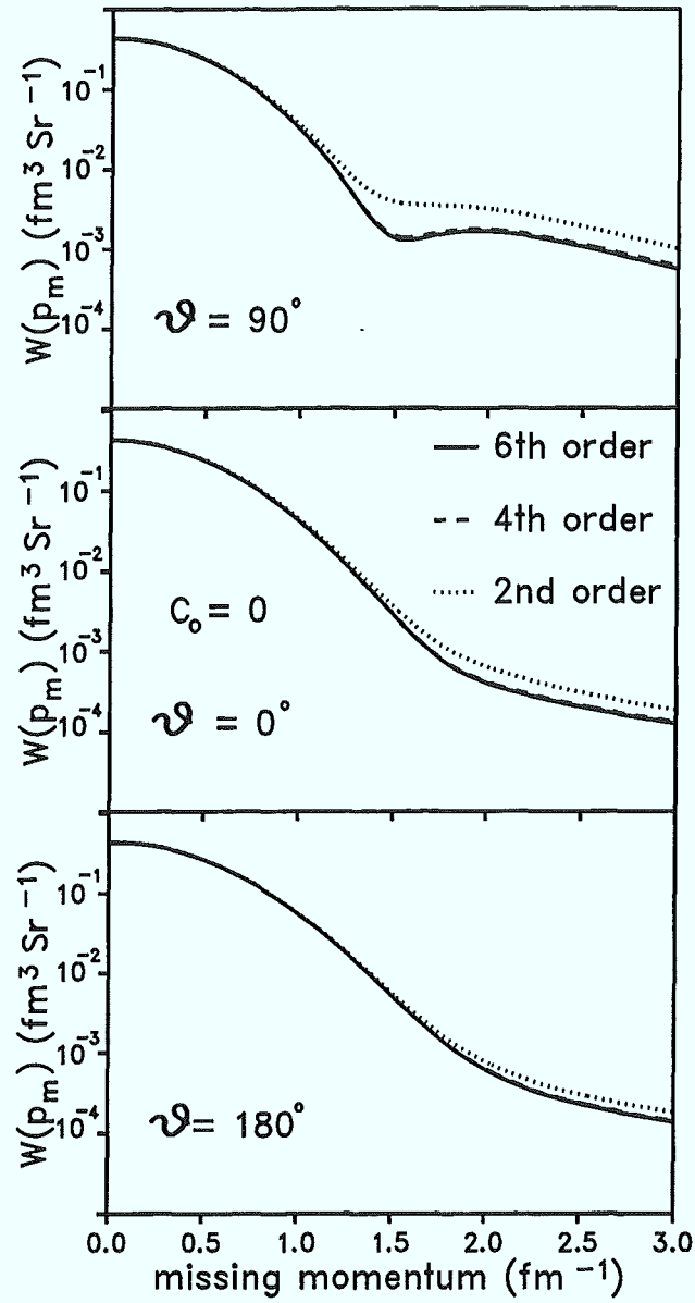
Figure 5.13: The convergence behaviour of the missing momentum distribution W(\vec{p}_m) without any correlations, i.e. C_o = 0 , for different angles \theta . The dotted line shows all the terms up to second order, the dashed line represents all terms up to fourth order, and the full line shows the complete result, i.e. all terms up to sixth order. The upper panel shows the results for \theta = 90^\circ , \theta = 0^\circ is shown in the middle panel and \theta = 180^\circ is shown in the lower panel. The other parameters are R_o = 1.29 \text{ fm} and r_c = 0.5 \text{ fm} .
