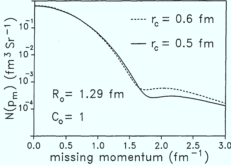
Figure 5.3: The single particle momentum distribution (SPMD) for different values of the correlation radius r_c . The solid curve shows r_c = 0.5\text{ fm} and the dashed curve shows r_c = 0.6\text{ fm} . The other parameters are R_o = 1.29\text{ fm} and C_o = 1 .
