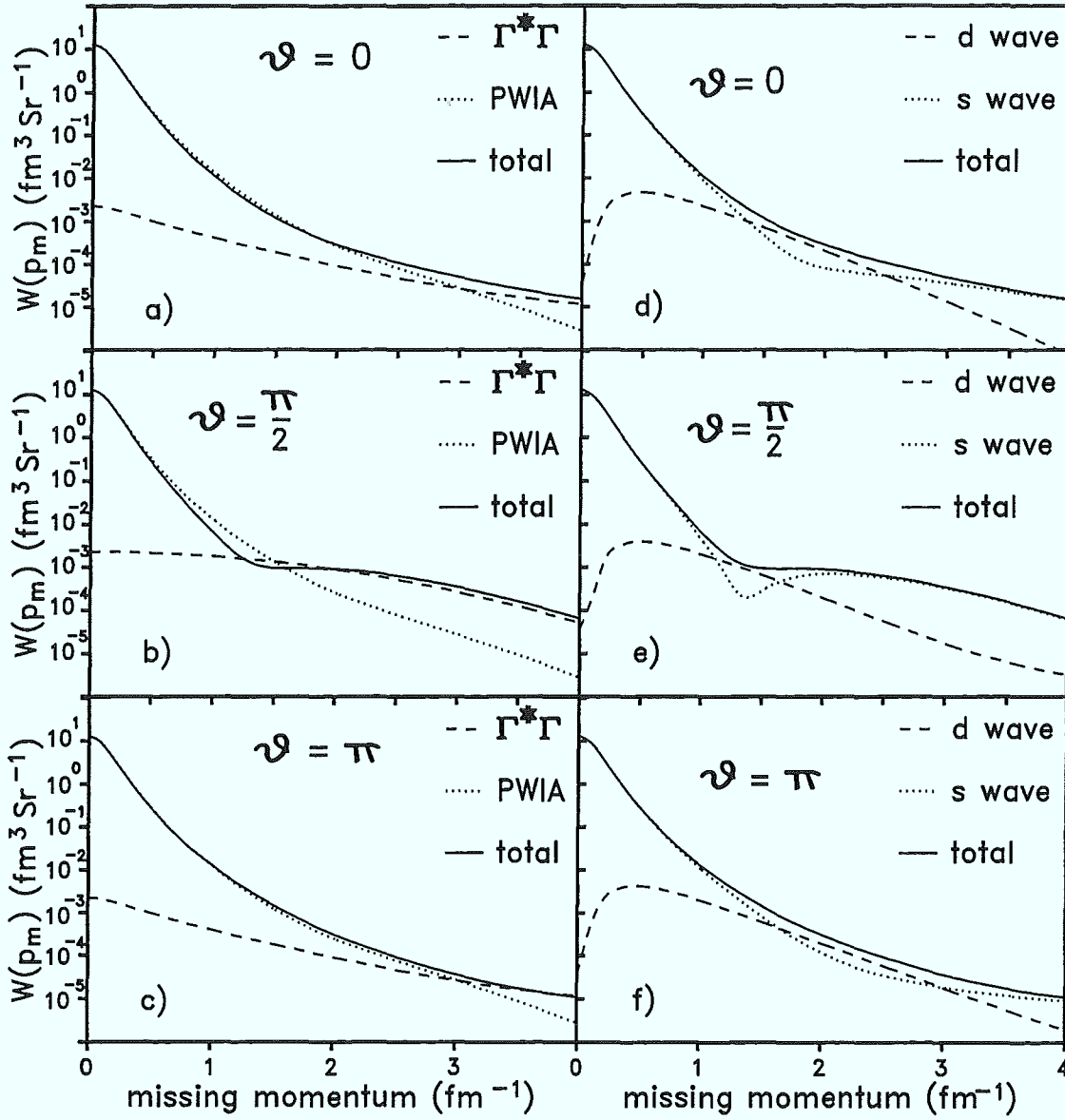
Figure 3.4: The missing momentum distribution W(\vec{p}_m) vs. p_m and its decomposition into (a-c) the PWIA and the rescattering contributions \propto \Gamma^* \Gamma and into (d-f) the S- and D-wave contributions at (a,d) \theta = 0^\circ , (b,e) \theta = 90^\circ and (c,f) \theta = 180^\circ . In panels (a-c) the full distribution W(\vec{p}_m) (solid curve) includes also the contribution \propto (\Gamma^* + \Gamma) from the interference of the PWIA and FSI amplitudes, which is not shown separately.
