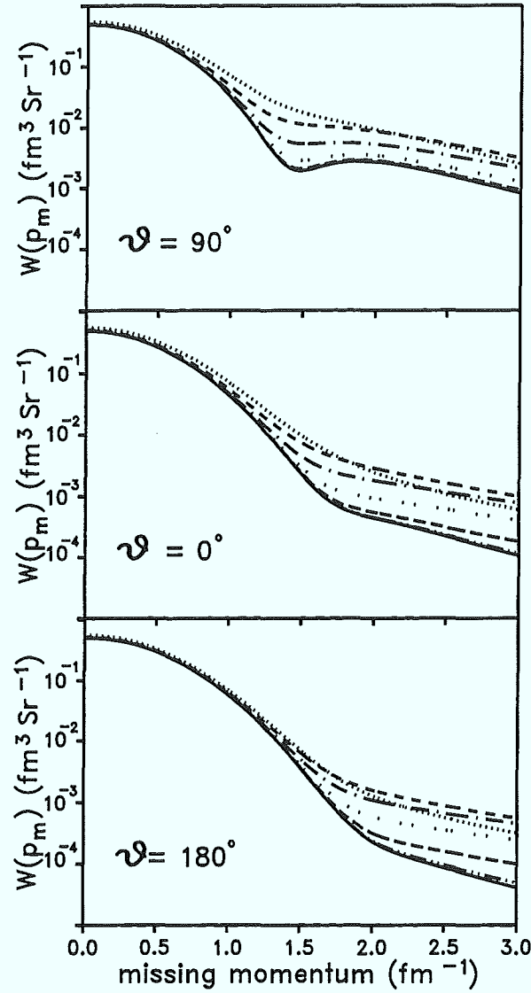
Figure 5.14: The convergence behaviour of the missing momentum distribution W(\vec{p}_m) with hard core correlations, i.e. C_o = 1 , for different angles \theta . The dotted line shows all the terms up to second order, the dashed line represents all terms up to fourth order, the dash-dotted line shows all terms up to sixth order, the double-dotted line includes all terms up to eighth order, the long-dashed line shows the calculation up to the tenth order, the dash-double-dotted line represents all terms up to twelfth order, and the full line shows the complete result, i.e. all terms up to 18th order. The upper panel shows the results for \theta = 90^\circ , \theta = 0^\circ is shown in the middle panel and \theta = 180^\circ is shown in the lower panel. The other parameters are R_o = 1.29\text{fm} and r_c = 0.5\text{fm} .
