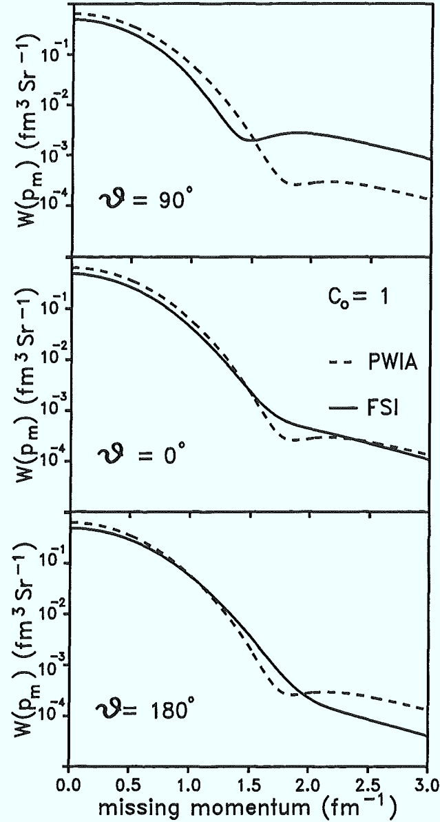
Figure 5.8: The missing momentum distribution W(\vec{p}_m) (full line) and the single particle momentum distribution N(p_m) (dashed line) for \theta = 90^\circ (upper panel), \theta = 0^\circ (middle panel), and for \theta = 180^\circ (lower panel). The parameters for the nuclear ground state are R_o = 1.29 \text{ fm} , r_c = 0.5 \text{ fm} and C_o = 1 .
