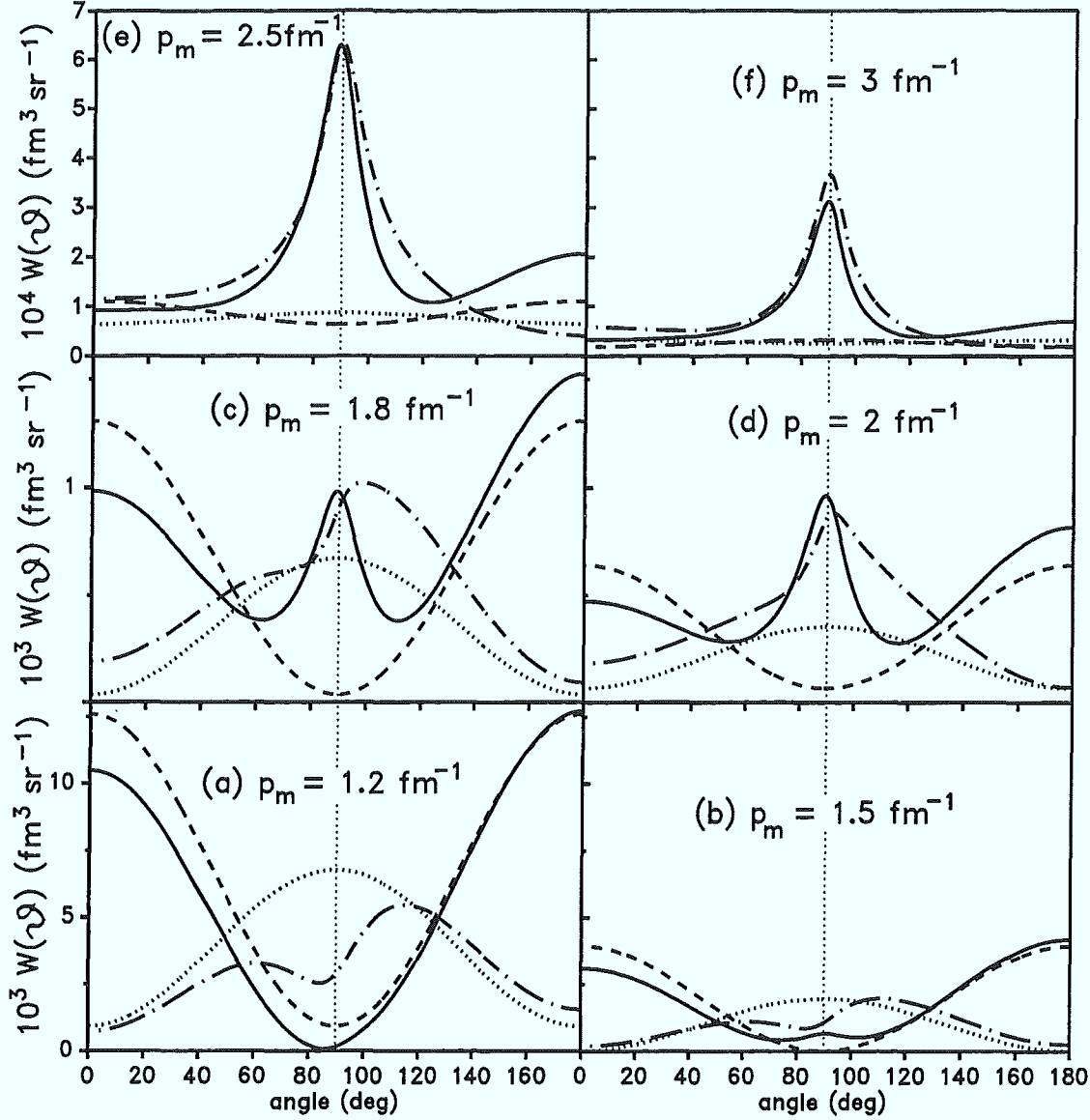
Figure 4.3: The angular dependence of the missing momentum distributions N_0 (dashed line), N_+ (dotted line), W_0 (solid line) and W_+ (dash-dotted line) for different values of the missing momentum p_m .
