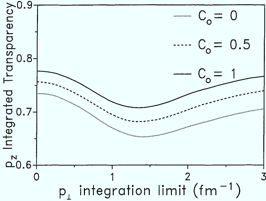
Figure 5.17: The fully integrated transparency T_{int} as function of the integration limit p_{\perp, max} as defined in (5.39) are shown for hard core correlations, C_o = 1 , (solid line), soft core correlations, C_o = 0.5 , (dashed line) and no correlations at all, C_o = 0 , (dotted line). The other ground state parameters are R_o = 1.29 fm and r_c = 0.5 fm .
