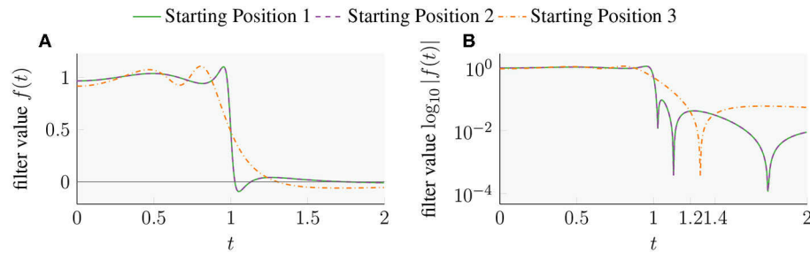
FIGURE 5 | (A) Three SLiSe filters obtained from gradient descent with different starting positions. (B) Semi-log plot with absolute value of the filter functions. The poles and residuals of the functions are listed in Table 1 .
