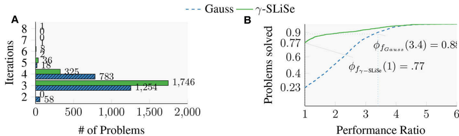
FIGURE 2 | Comparisons of the Gauss filter with our replacement candidate, \gamma -SLiSe, with p = 1.5m on a test set of 2116 benchmark problems obtained from the “Si2” matrix. Both filters have 16 poles and are plotted in Figure 3 . (A) Number of FEAST iterations required by \gamma -SLiSe and the Gauss filter. (B) Performance profiles of convergence rates for \gamma -SLiSe and Gauss filters.
