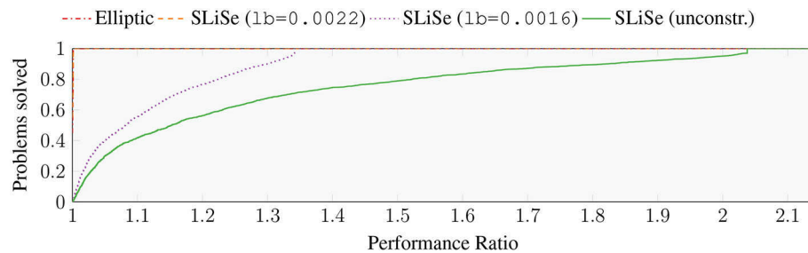
FIGURE 8 | Performance profile comparing the worst condition number for the linear systems arising from filter application to 2116 problems obtained from the “SI2” matrix. The performance ratio for the Elliptic and SLiSe ( 1b=0.0022 ) filters are one over the entire abscissa range.
