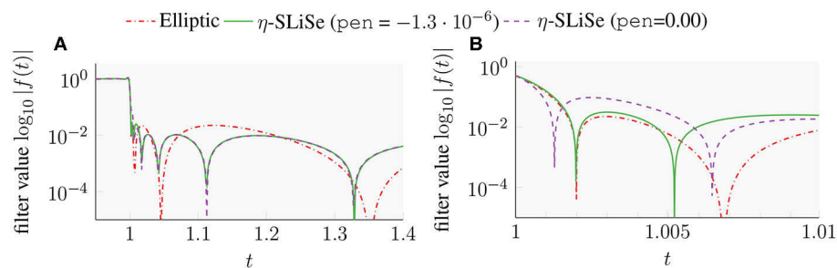
FIGURE 9 | Plots of the Elliptic filter, \eta -SLiSe, and the \eta -SLiSe filter without penalty term. All filters have 16 poles and coefficients. (A) Semi-log plot. (B) Semi-log plot. Abscissa limited to [1, 1.01] .
