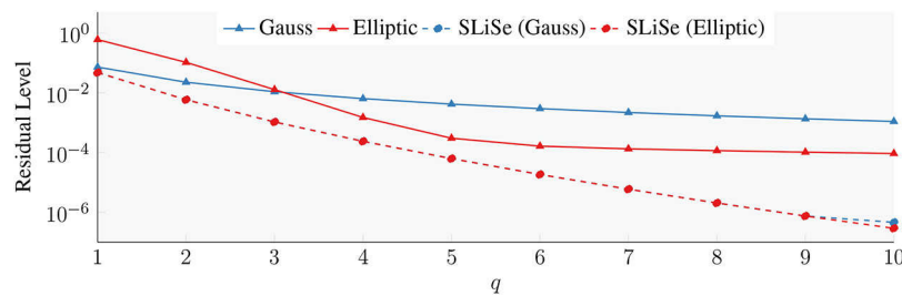
FIGURE 6 | Residual levels of Gauss and Elliptic filters, as well as, SLiSe filters obtained from Gauss and Elliptic filters as starting positions.
