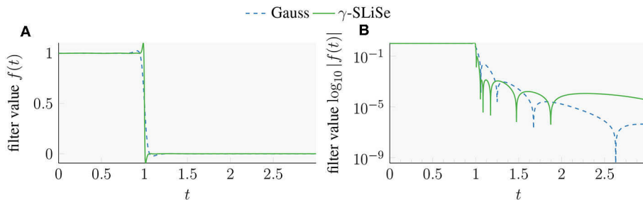
FIGURE 3 | Plots of the Gauss filter and our replacement candidate, \gamma -SLiSe. Both filters have 16 poles and coefficients. (A) Linear-scale plot. (B) Semi-log plot.
