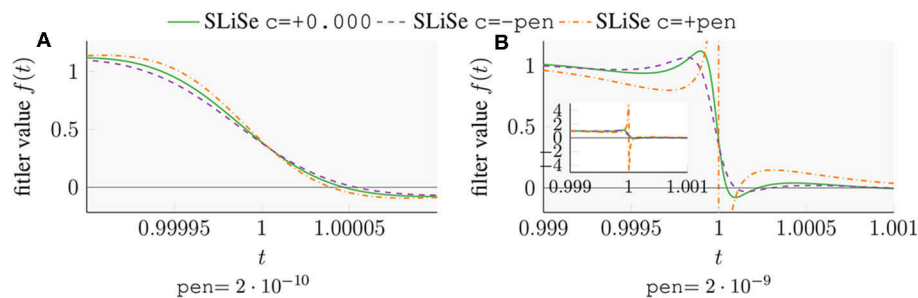
FIGURE 7 | Examples of filters obtained via penalty terms. (A) An appropriately sized penalty parameter yields filters of different steepness. (B) Too large a (positive) penalty parameter results in a pole on the real axis.
