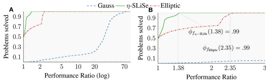
FIGURE 4 | Semi-log performance profile of the convergence ratio for the Gauss, \eta -SLiSe, and Elliptic filters. \eta -SLiSe is meant to replace the Elliptic filter. All filters have 16 poles and p = m . (A) Semi-log performance profile of the convergence rate. (B) The same performance profile zoomed into [1, 3] with a linear axis.
