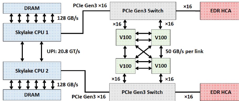
(b) JUWELS Cluster compute node (GPU partition).
