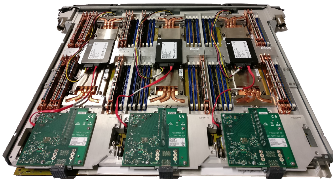
Figure 2: Example of a BullSequana compute blade encompassing three compute nodes. Please note that the shown local storage devices are not built into the JUWELS compute nodes. Copyright: Atos.
