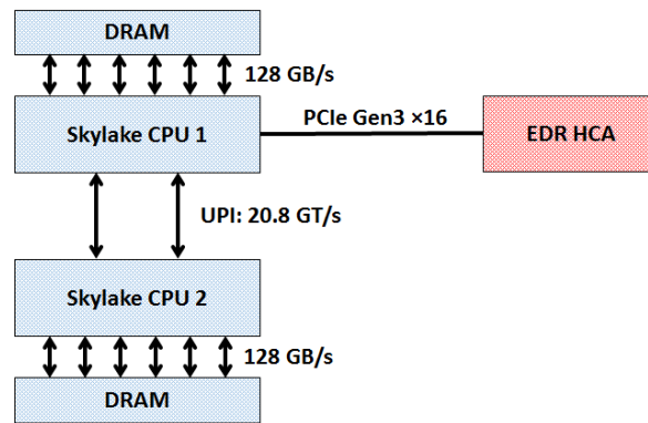
(a) JUWELS Cluster compute node (CPU partition).
