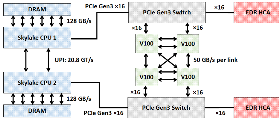
(b) JUWELS Cluster compute node (GPU partition).
