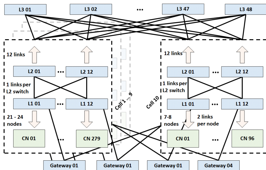
Figure 4: Schematic of the JUWELS InfiniBand network topology. Please note that the 10th cell is only half populated in the current deployment. Each cell is connected to each gateway switch with at least one link. Various service nodes that are connected to free ports in the level one switches are not shown.
