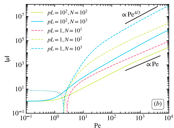
FIG. 2. Modulus of the stretching coefficient \mu = 2\nu/(3p) as a function of Péclet number. (a) Variation of \mu with the bending stiffness ( pL ) for L/l = N = 10^2 . (b) Variation of \mu with N for pL = 10^2 (solid lines) and pL = 1 (dashed lines). The dotted lines indicate the negative part of \mu for the respective pL , which appears for pL \lesssim \pi . With increasing \text{Pe} , \mu crosses zero, which leads to a rapid change of |\mu| . The black solid lines indicate power-law dependencies.
