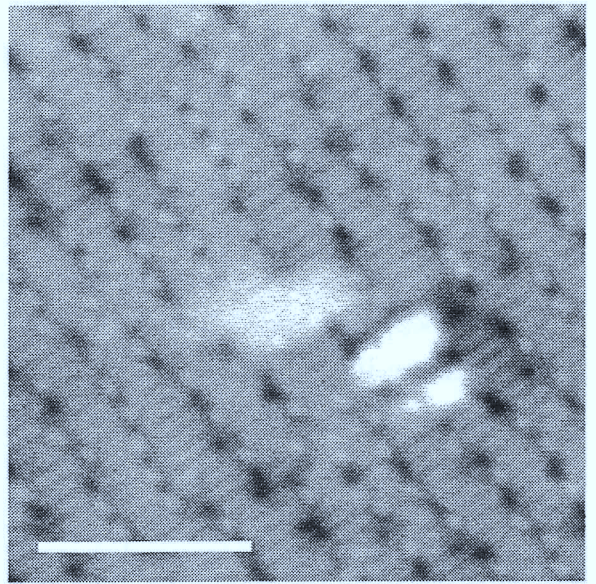
d) 0,2 ML \text{Co}/\text{Si}(100) , T_{\text{Si}} = 500^\circ\text{C}
