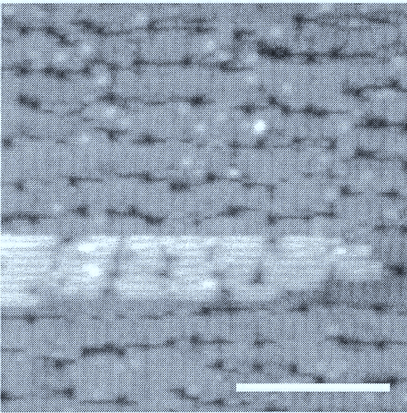
c) 0,1 ML \text{Co}/\text{Si}(100) , T_{\text{Si}} = 500^\circ\text{C}
