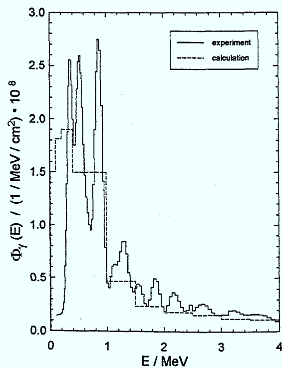
d) photon spectrum up to 4 \text{ MeV}
