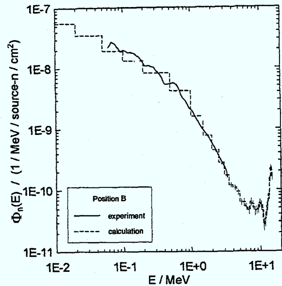
Fig. 4 Measured neutron spectrum in position B compared to calculation (FENDL-1 data)
