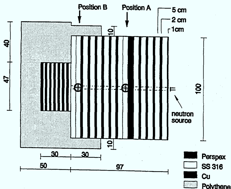
Fig. 1 Bulk shield assembly and positions for neutron energy spectra measurements
