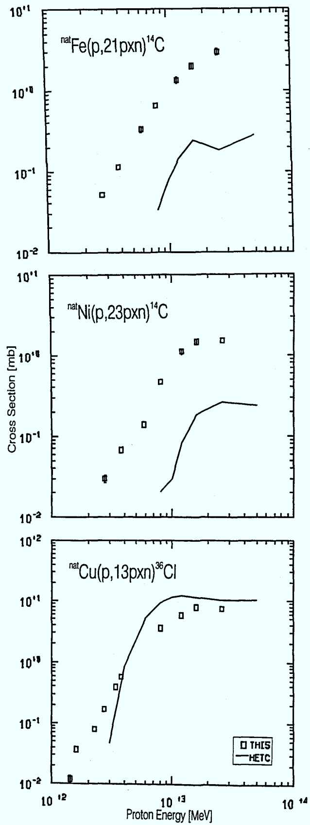
Fig. 3. Experimental and calculated excitation functions for the production of ^{14}\text{C} from iron and nickel and of ^{36}\text{Cl} from copper.
