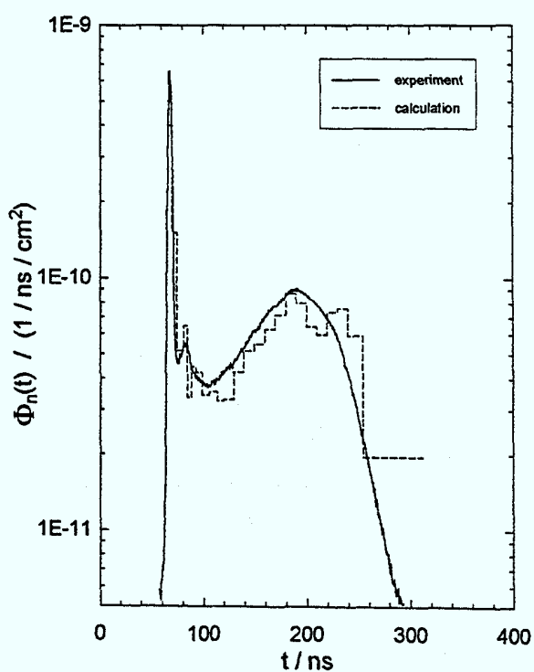
c) neutron time-of-arrival spectrum
