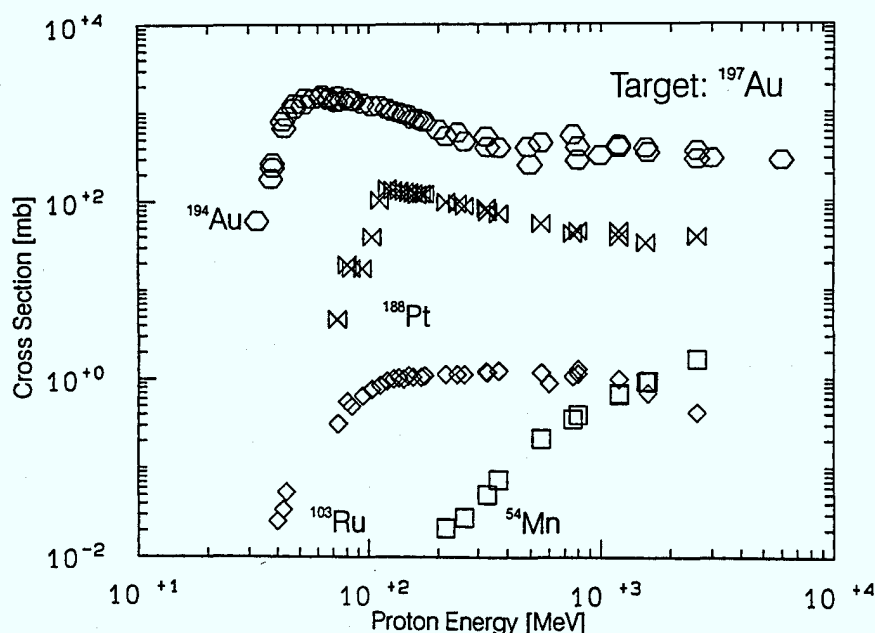
Fig. 1. Experimental excitation functions for the production of ^{54}\text{Mn} , ^{103}\text{Ru} , ^{188}\text{Pt} and ^{194}\text{Au} by proton-induced reactions on gold. The data are exclusively from this work.
