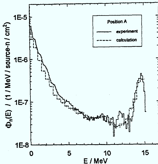
Fig. 3 Measured neutron spectrum in position A compared to calculation (FENDL-1 data)
