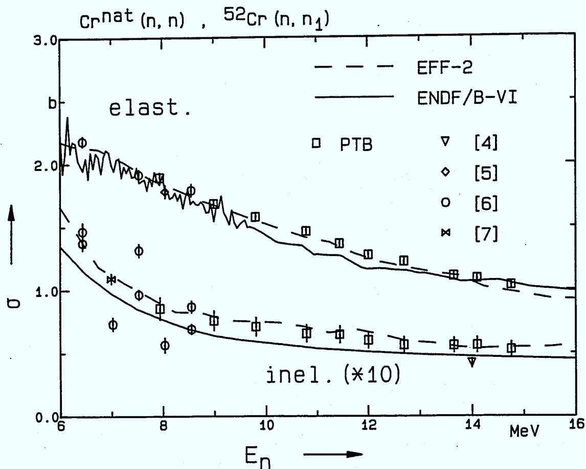
Fig. 1 Angle-integrated elastic cross sections from natural chromium and inelastic cross sections to the first excited state in the ^{52}\text{Cr} isotope (note the scale expansion factor of 10); data from the literature [4-7] are included, the EFF-2 and ENDF/B-VI evaluations presented here have been made for the main isotope ^{52}\text{Cr} .
