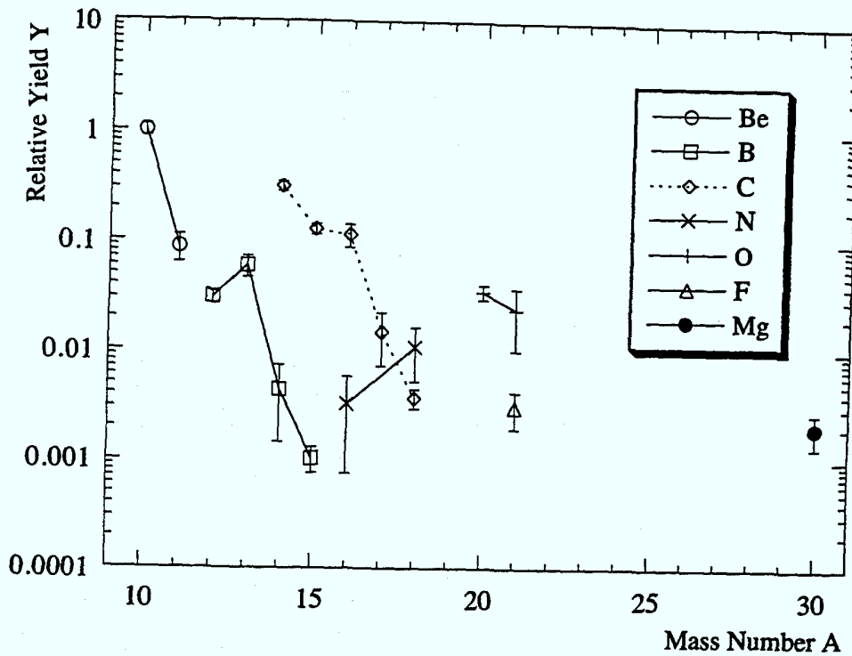
Fig. 2 Yields of ternary particles relative to ^{10}\text{Be}=1 obtained as discussed in the text. The absolute yield of ^{10}\text{Be} amounts to (4 \pm 1) \cdot 10^{-3} \%
