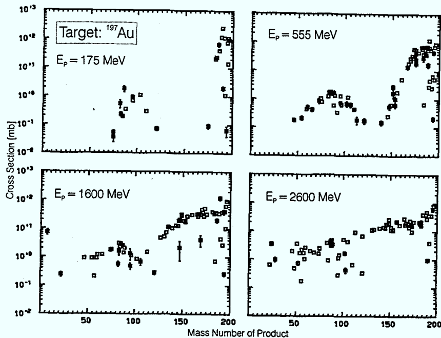
Fig. 2 Experimental cross sections for residual nuclide production by p-induced reactions on gold as function of product mass number. The data are exclusively from this work.
