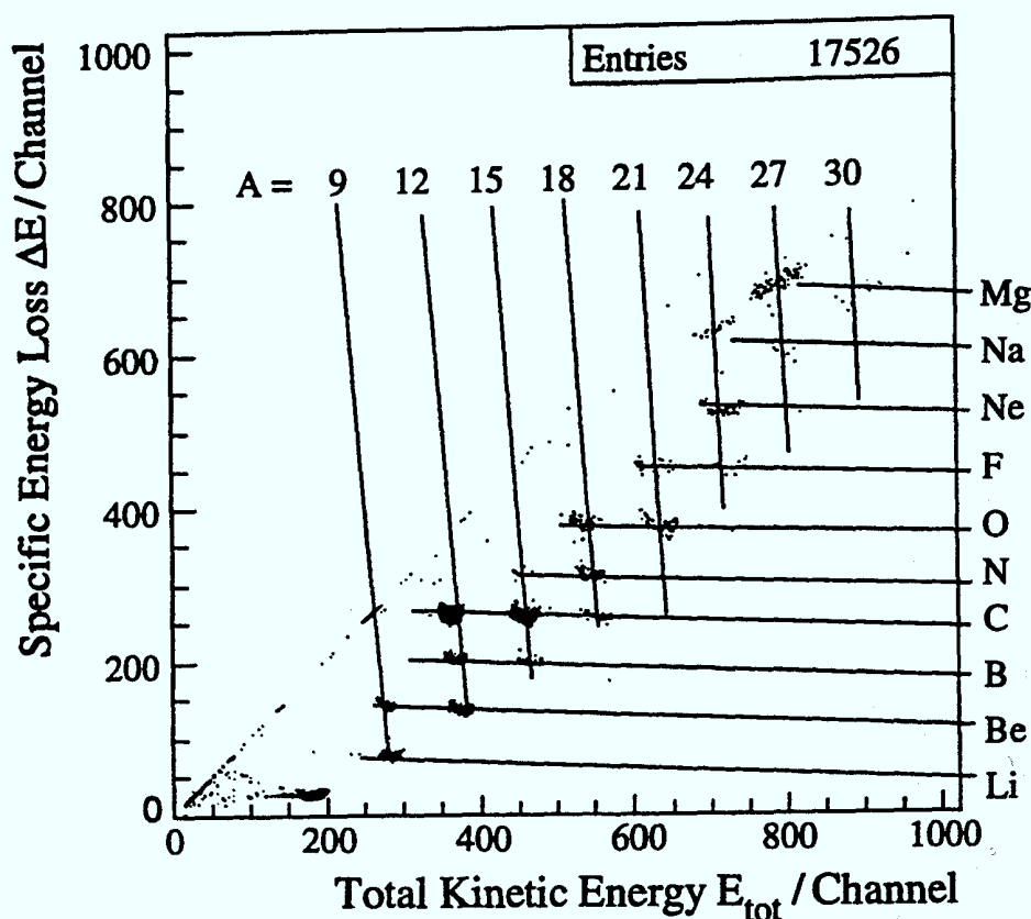
Fig. 1 "Scatter plot" of events registered in the ionization chamber with split anode (at a Lohengrin setting A/q=3 and E/q=3.6 [MeV]). The specific energy loss ( \Delta E ) is plotted versus the total kinetic energy ( E_{tot} ) of the fragments. Relative intensities are obtained by integrating the events registered in an appropriate area of the matrix.
