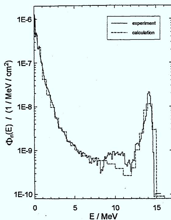
b) high-energy part of the neutron spectrum
