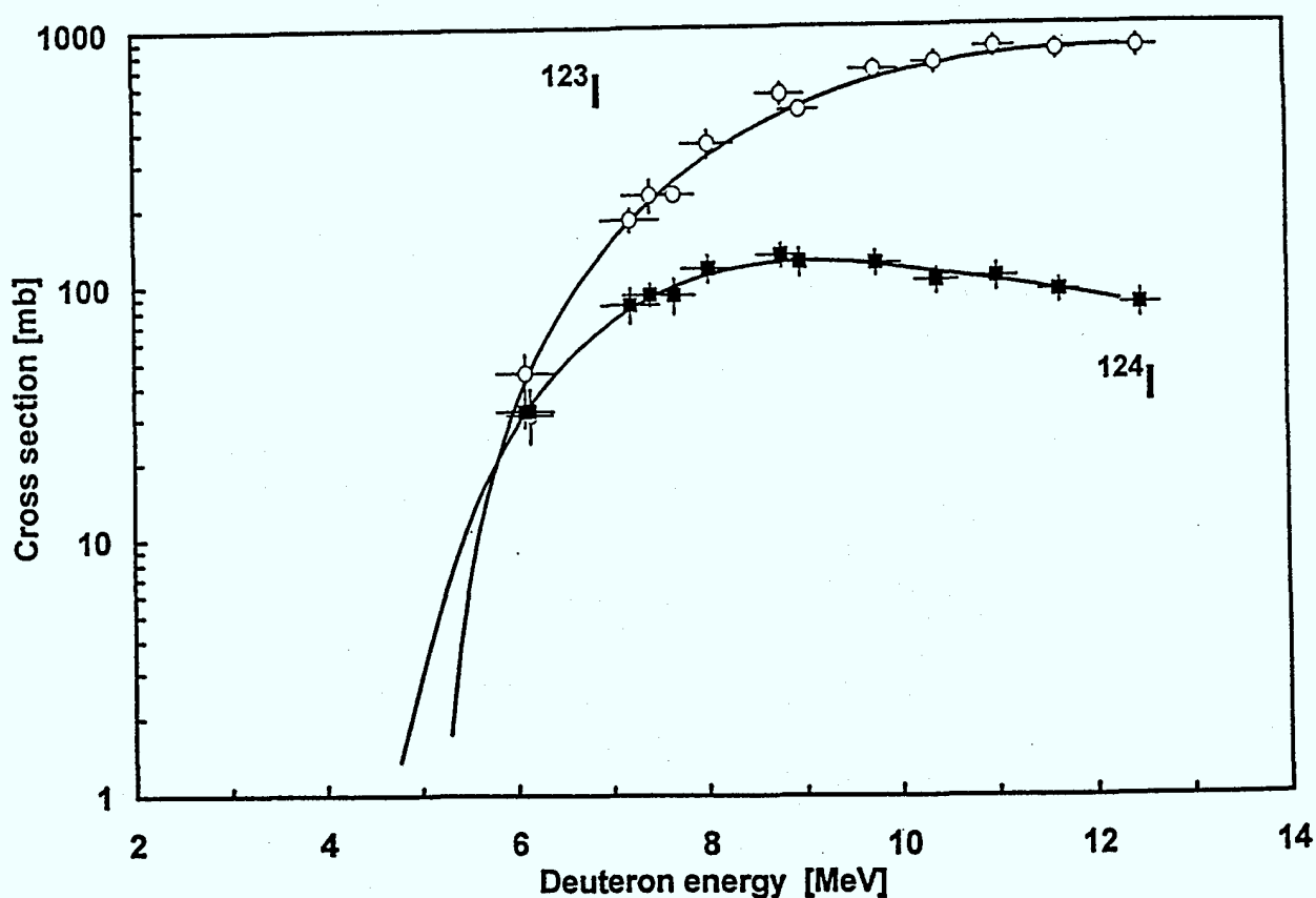
Fig. 3 Excitation functions of ^{123}\text{Te}(\text{d},\text{n})^{124}\text{I} and ^{123}\text{Te}(\text{d},2\text{n})^{123}\text{I} reactions. The solid lines give spline fits to the experimental data (for details cf. Ref. [10]).
