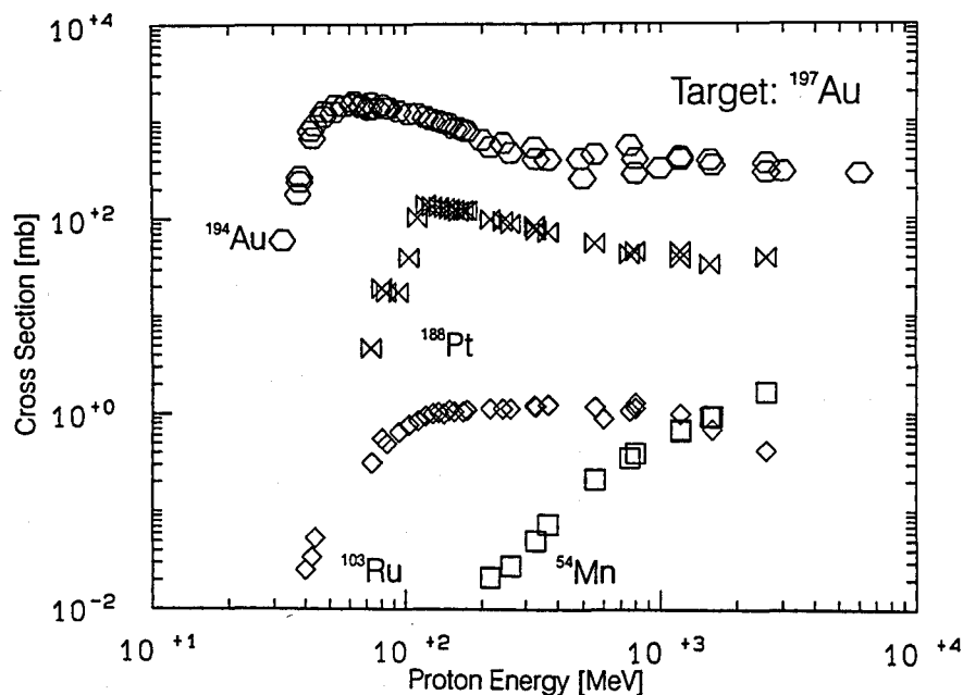
Fig. 1. Experimental excitation functions for the production of ^{54}\text{Mn} , ^{103}\text{Ru} , ^{188}\text{Pt} and ^{194}\text{Au} by proton-induced reactions on gold. The data are exclusively from this work.
