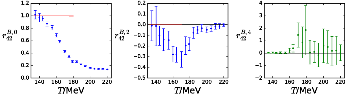
Figure 6. Taylor expansion coefficients for \kappa_B \sigma_B^2 = \frac{\chi_4^B(T, \hat{\mu}_B)}{\chi_2^B(T, \hat{\mu}_B)} as functions of the temperature: r_{42}^{B,0} (left panel) r_{42}^{B,2} (middle panel), r_{42}^{B,4} (right panel). The latter is not obtained independently, but by means of the prior ansatz (see text): for this reason, we plot it in green.
