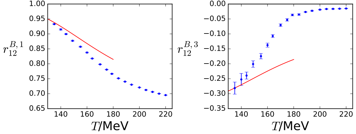
Figure 4. Taylor expansion coefficients for \frac{M_B}{\sigma_B} = \frac{\chi_1^B(T, \hat{\mu}_B)}{\chi_2^B(T, \hat{\mu}_B)} as functions of the temperature: r_{12}^{B,1} (left panel) and r_{12}^{B,3} (right panel).
