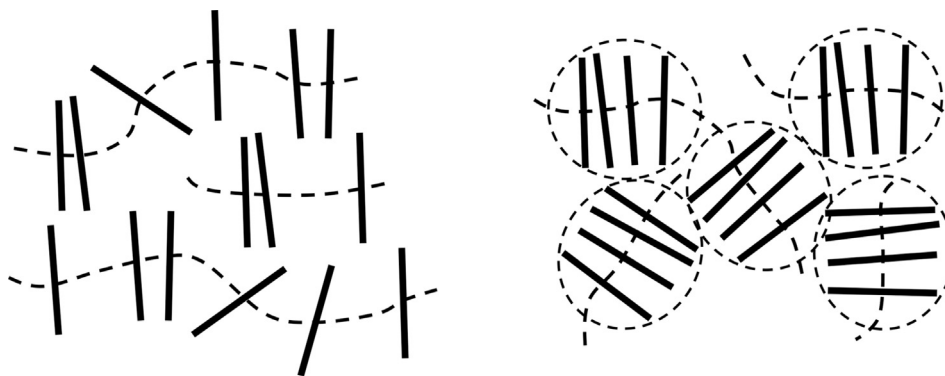
Fig. 4. Sketches for the meaning of the locally columnar model that connects a scattering model with a thermodynamic model.
