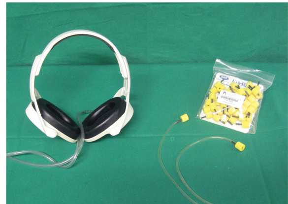
Fig. 1 Left: standard pneumatic headphone (Siemens), right: earphones (3M) connected to the pneumatic audio system of the MR
