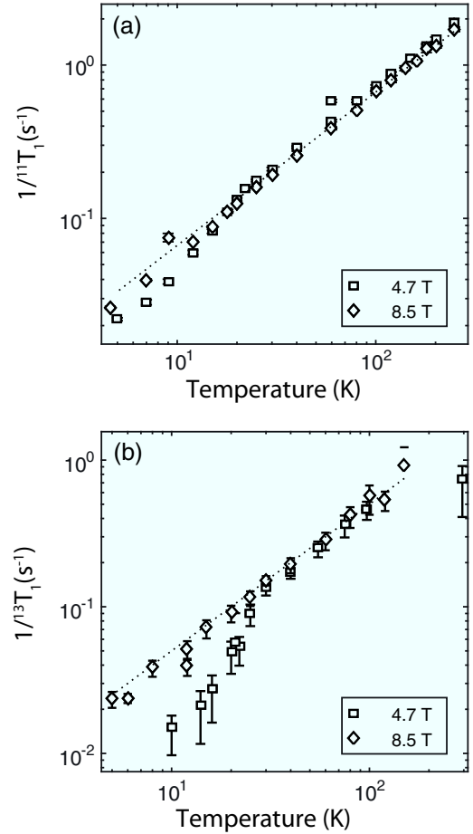
FIG. 5. Spin-lattice relaxation rate of \text{MgB}_{1.95}\text{C}_{0.05} . (a) ^{11}\text{B} NMR. (b) ^{13}\text{C} NMR. The black dotted line is the Korringa product. Values are 155 and 200 s K for boron and carbon, respectively.
