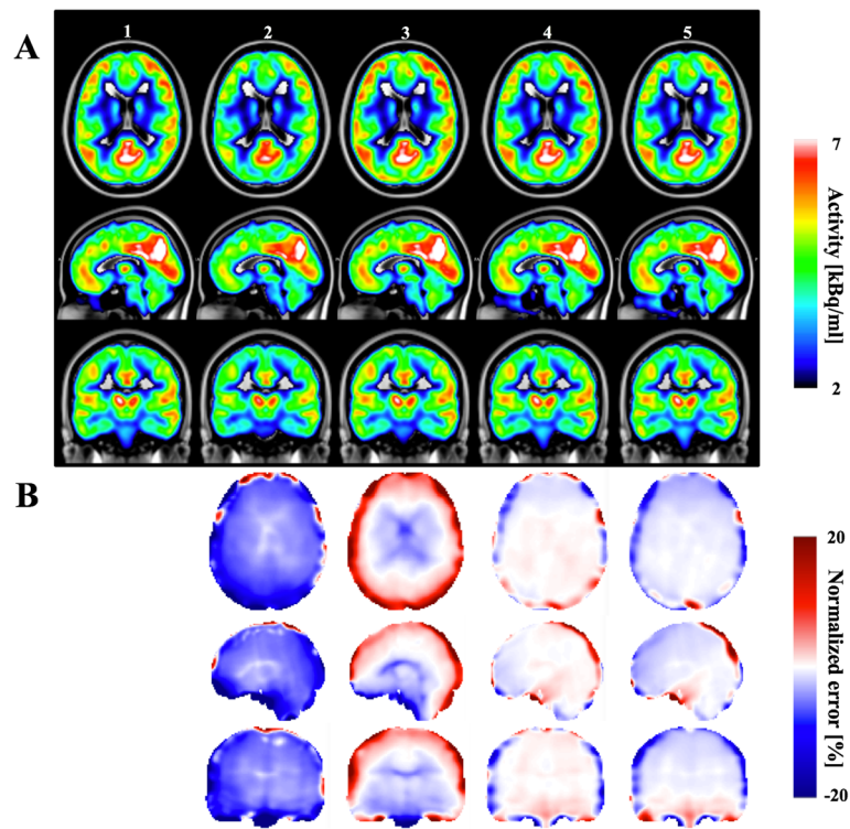
Fig. 5 Comparison of PET images for the Test participant. Comparison of PET images for the Test participant (panel a ) reconstructed with five different attenuation maps: PET_{ref} (column 1), PET_{UTE} (column 2), PET_{UCL} (column 3), PET_{sUTEcont} (column 4) and PET_{sUTEfix} (column 5). Comparison of corresponding normalized error (panel b ) for the reconstructed PET data is depicted
