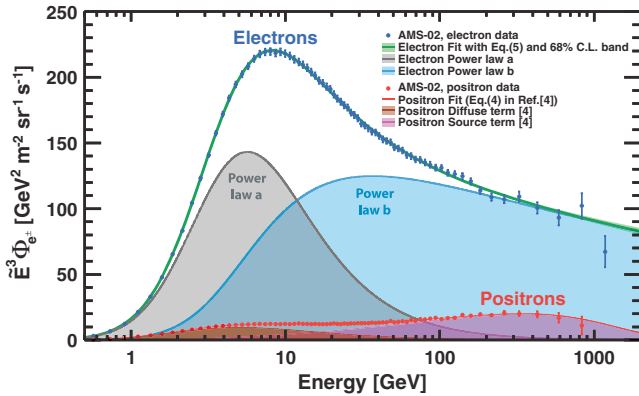
FIG. 4. The two power law fit of Eq. (5) to the electron flux data in the energy range [0.5–1400] GeV with 68% C.L. (green band). The two power law components a and b of Eq. (5) are represented by the gray and blue areas, respectively. Also shown are the positron spectrum together with the fit of Eq. (4) of Ref. [4] including the positron diffuse (i.e., interstellar secondary production) term (the brown area) and positron source term (the magenta area) contributions.
