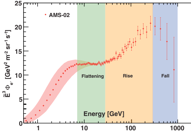
FIG. 1. For display purposes, the positron flux, \Phi_{e^+} is traditionally presented scaled by \tilde{E}^3 . The resulting AMS positron spectrum, \tilde{E}^3\Phi_{e^+} , (red data points) is shown as a function of energy \tilde{E} . The time variation of the flux at low energies due to solar modulation [3] is indicated by the red band. To guide the eye, the vertical color bands indicate the energy ranges corresponding to changing behavior of the spectrum: flattening, rising, and falling spectrum (see text).
