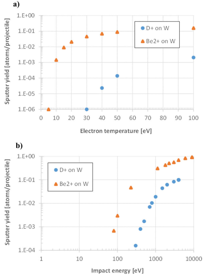
Fig. 4. Sputter yields based on SDTrimSP calculations for D + and Be 2+ ions impinging on tungsten: (a) inter-ELM and (b) intra-ELM conditions.
