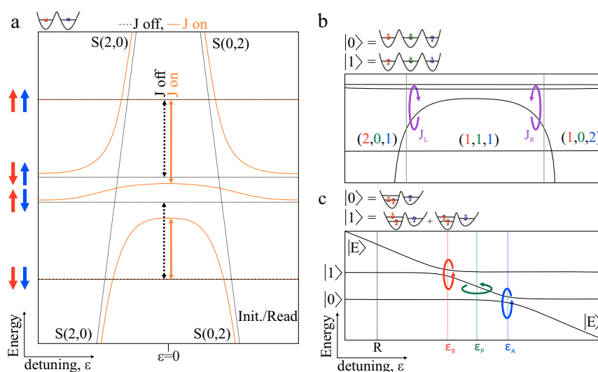
Fig. 2 Energy level diagram of spin states in quantum dots. a Low-energy spectrum of two uncoupled spins (black dotted line) and coupled spins (orange solid line) in two quantum dots as a function of the detuning energy \epsilon , the relative energy difference between the left and right dot levels, which is controlled by the corresponding dot gate voltages. The exchange interaction provided by the charge states with double occupancies ( S(2, 0) and S(0, 2) ) can be used for two-qubit operations between single spin qubits as the exchange interaction J modifies the qubit resonance frequencies. While in the uncoupled situation the transition |\downarrow\downarrow\rangle to |\uparrow\uparrow\rangle has the same energy as the |\downarrow\uparrow\rangle to |\uparrow\downarrow\rangle transition, these become different when exchange is on, allowing to drive rotations of one spin conditional on the state of the other. 75 Alternatively, when briefly turning on the exchange, the two spin states will exchange over time, which also constitutes a two-qubit gate. While many experimental works exploit the detuning to control the exchange amplitude, directly controlling the tunnel coupling allows to operate the system at the so-called symmetry point, where the exchange energy is less sensitive to charge noise, dramatically improving the gate fidelity. 104, 105 The joint state of two coupled spins, for instance the spin singlet and one of the triplet states, can also be used as a single qubit. 65 The advantage of such a qubit is that one qubit axis is electrically controlled and two qubits can be coupled capacitively. 23 For universal control, a magnetic field gradient is required, for instance induced by a nearby nanomagnet. All electrical control is possible using more advanced combinations of spins, for example, b the so-called exchange-only qubit and c hybrid qubit. b The encoding in the exchange-only qubit is based on three spins in three adjacent quantum dots and control is provided via the exchange between the outer quantum dots and the central dot, J_L and J_R . 46, 77, 78 c The hybrid qubit is based on three spins as well, but requires only two quantum dots. 48 Universal qubit control makes use of the anti-crossings between the lowest three energy states to induce rotations about different axes. While these qubit representations are clearly more involved compared to the single-spin qubit, their operation may offer advantages for scaling toward large arrays where not the number of dots per qubit but the number and type of control lines per dot will likely form the largest challenge
