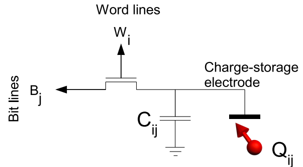
Fig. 3 Charge-storage capacitors for biasing quantum dots, in analogy to DRAM. Individual qubit communication can be achieved via a pair of word lines and bit lines. A voltage can be applied to qubit gate Q_{ij} via B_j by setting W_i high and stored on capacitance C_{ij} by subsequently setting W_i low. Depending on the pitch and dimensions of transistors and quantum dots, more complex circuits can be constructed based on this method
