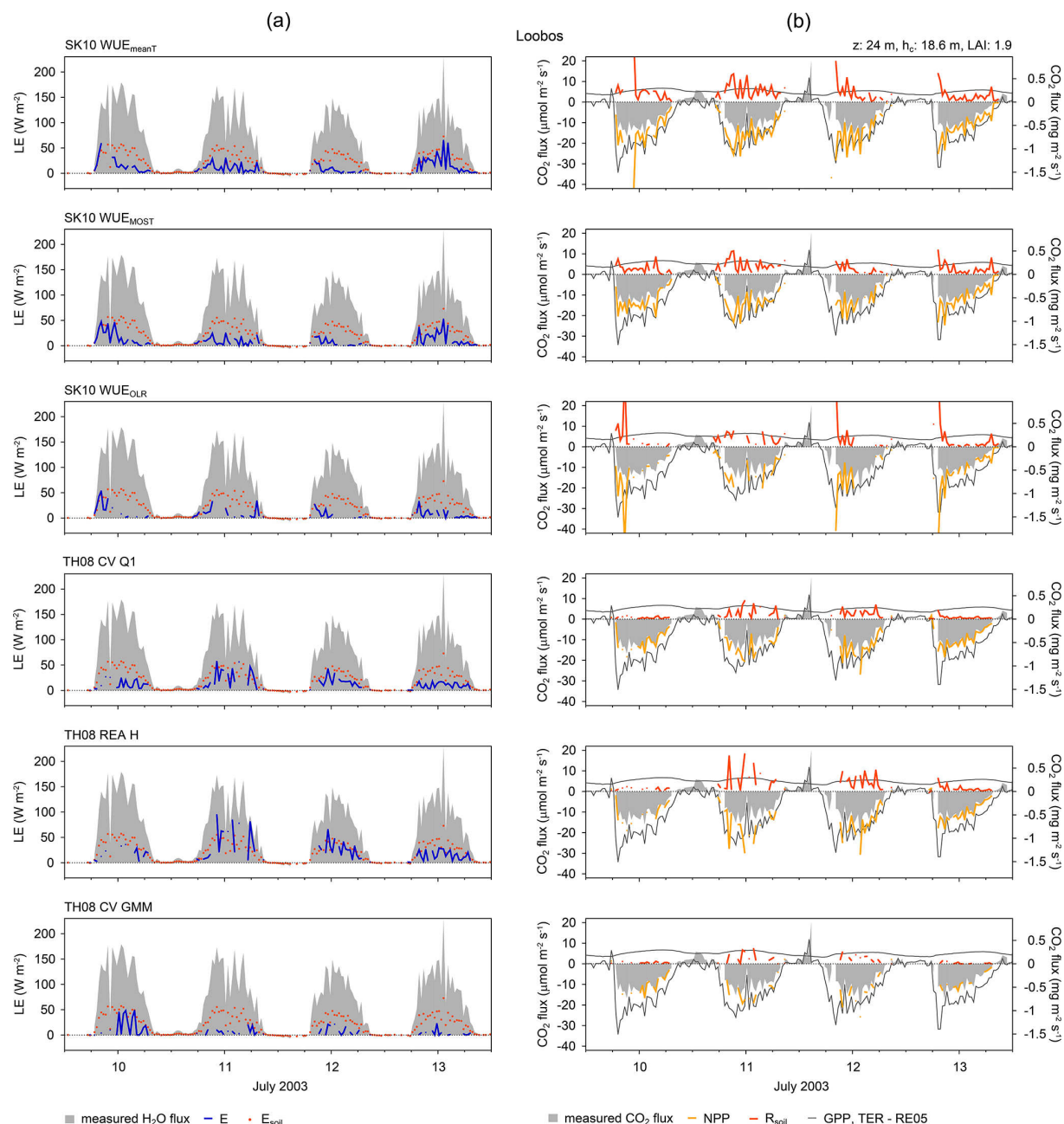
Figure 2. Source partitioning results for (a) H 2 O and (b) CO 2 fluxes in half-hourly time steps for the Loobos study site (forest) in the Netherlands. The figure shows 4 days of the considered time period and selected method versions (see text for description). Results for all days and for every method version are shown in the Supplement. Grey areas show the measured water and CO 2 fluxes. Soil evaporation estimates derived based on Beer's law and CO 2 flux estimates by Reichstein et al. (2005; RE05) are also included (LE: latent heat flux; E : evaporation; E_{\text{soil}} : estimated soil evaporation; GPP: gross primary production; NPP: net primary production; TER: total ecosystem respiration; R_{\text{soil}} : soil respiration; z : measurement height; h_c : canopy height; LAI: leaf area index).
