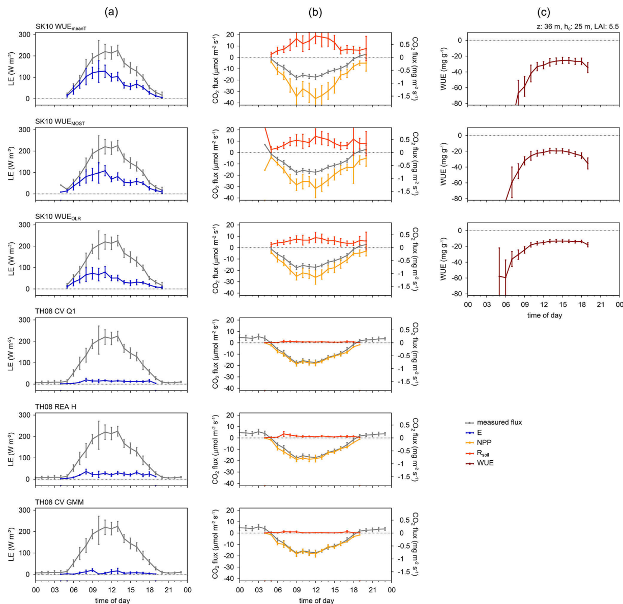
Figure 3. Diurnal dynamics of source partitioning results for (a) H 2 O and (b) CO 2 fluxes and (c) water use efficiency (WUE) for the Waldstein study site (forest) in Germany for 4–10 July 2016 and for selected method versions (see text for description; LE: latent heat flux; E : evaporation; NPP: net primary production; R soil : soil respiration; z : measurement height; h c : canopy height; LAI: leaf area index). Error bars indicate the 95 % confidence intervals of the mean values.
