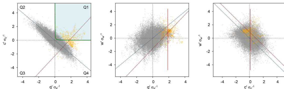
Figure 1. Exemplary scatterplots of w' , q' , and c' from the Wüstebach study site (forest), 18 May 2015, 12:00–12:30 LT (local time), including results of the cluster analysis by Gaussian mixture model (orange data points) for the conditional sampling. Also shown are the hyperbolic threshold ( H = 0.25 , green line) after Thomas et al. (2008), the averages of q and c only considering data points of the respiration–evaporation “cloud” (red lines), and reduced major axis regression lines after Webster (1997) for all data points (blue dashed lines) and only cloud data points (red dashed lines). In this example, calculating the covariance for w and c considering the CO 2 average of the cloud yielded a negative soil flux (negative correlation). Thus, only cloud data points within quadrant 1 in the original q' – c' plane were considered for flux calculation using averages of all data points.
