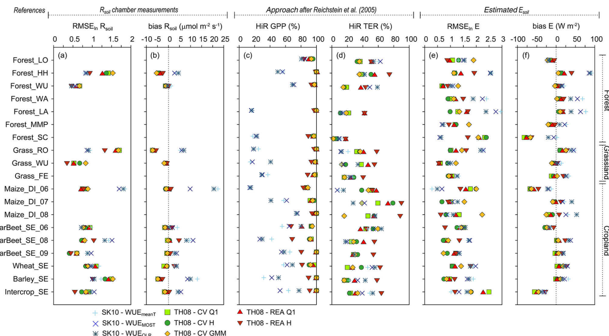
Figure 6. Error metrics for source partitioning results for each study site and method version (see text for description). (a–b) Root mean square error in log-transformed data ( RMSE_{\ln} ) and bias considering soil respiration ( R_{\text{soil}} ) chamber measurements, (c–d) percent fraction of time steps with partitioning results in the range (HiR) of estimated gross primary production (GPP) and total ecosystem respiration (TER) by the approach after Reichstein et al. (2005), and (e–f) RMSE_{\ln} and bias considering soil evaporation ( E_{\text{soil}} ) estimated based on Beer's law.
