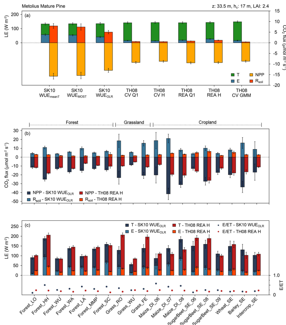
Figure 5. Averages of source partitioning results for the following: (a) H 2 O and CO 2 fluxes for the Metolius Mature Pine study site (forest) in the US and for all method versions; (b) CO 2 fluxes for all study sites and for the approaches after Scanlon and Kustas (2010; SK10) with WUE OLR and after Thomas et al. (2008; TH08) with REA H; and (c) H 2 O fluxes and the partitioning fraction E / ET for all study sites and for the approaches SK10 WUE OLR and TH08 REA H (see text for description; LE: latent heat flux; E : evaporation; NPP: net primary production; R_{soil} : soil respiration; z : measurement height; h_c : canopy height; LAI: leaf area index). Error bars indicate the 95 % confidence intervals of the mean values. For each study site, net fluxes (evapotranspiration and net ecosystem exchange) differ between method versions because each method version found a different number of partitioning solutions, and thus the averages were taken from different subsets of the original data.
