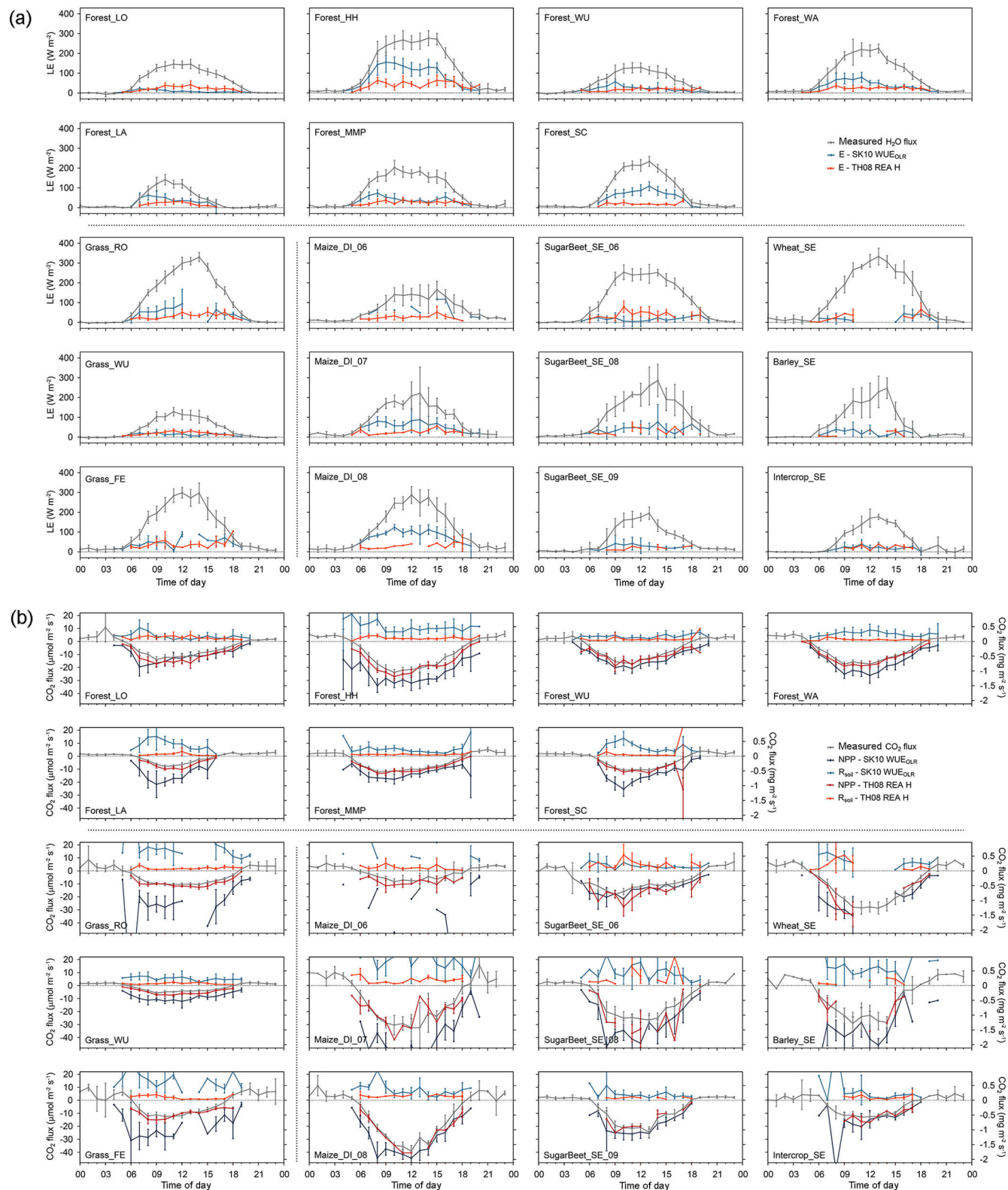
Figure 4. Diurnal dynamics of source partitioning results for (a) H 2 O and (b) CO 2 fluxes for all study sites and for the approach after Scanlon and Kustas (2010; SK10) with WUE OLR and after Thomas et al. (2008; TH08) with REA H (see text for description; LE: latent heat flux; E: evaporation; NPP: net primary production; R soil : soil respiration). Error bars indicate the 95 % confidence intervals of the mean values.
