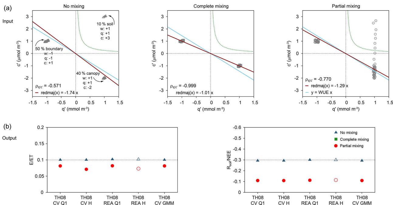
Figure 7. (a) Setup of the conceptual model for synthetic fluctuations ( q' and c' ) originating from the soil, canopy, or boundary layer with differing degrees of mixing (no, complete, or partial mixing between soil and canopy sink–source) including water use efficiency ( \text{WUE} = -1.444 \mu\text{mol mmol}^{-1} = -3.53 \text{ mg g}^{-1} ; blue line), reduced major axis regression (red line) after Webster (1997), hyperbolic threshold criterion after Thomas et al. (2008; TH08) ( H = 0.25 ; green dashed line), and correlation coefficient between q' and c' ( \rho_{q'c'} ). (b) True known partitioning ratios (dashed line) and source partitioning results from all TH08 method versions (see text for description) for each degree of mixing.
