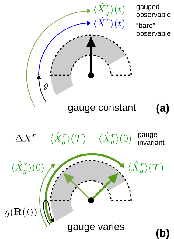
FIG. 1. (a) Global gauge transformation \hat{X}^r \rightarrow \hat{X}_g^r = \hat{X}^r + g\mathbb{1} leaving both currents I_{X^r} and transported observable \Delta X^r invariant. The gray scale bar is translated by fixed amount g relative to the ungauged one ( g = 0 , dashed outline). The needle corresponds to the quantum state that from the observable \hat{X}_g^r the measurement expectation value \langle \hat{X}_g^r \rangle = \langle \hat{X}^r \rangle + g indicated. (b) Local gauge transformation \hat{X}^r \rightarrow \hat{X}_g^r = \hat{X}^r + g[\mathbf{R}]\mathbb{1} , changing the currents to I_{X_g^r} but leaving the transported observable \Delta X^r invariant. Since the meter scale is gauged in a continuous way as function of the parameters \mathbf{R} , it returns to its original position every period: g(\mathbf{R}(\mathcal{T})) = g(\mathbf{R}(0)) .
