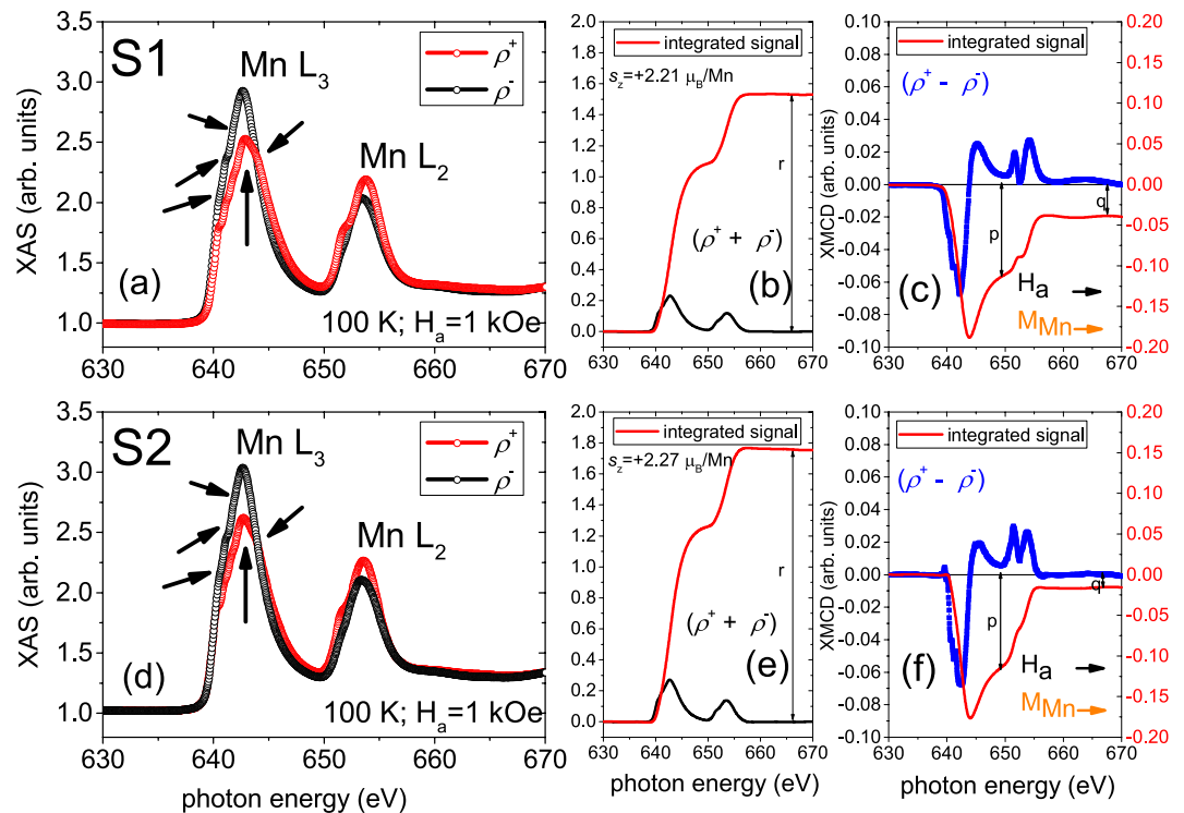
Figure 6. Mn L edge XAS, XMCD spectra and sum rules for s_z of specimens S1 and S2. TEY XAS signals of the Mn L_{3,2} edges with two different photon helicities ( \rho^+ and \rho^- ) from the (a) S1 and (d) S2 MLs measured at 100 K and 1 kOe (saturation). XAS (summation) and XMCD (difference) signals corresponding to the XAS signals for S1 (b,c) and S2 (e,f) after baseline correction that takes into account of the linear increase of the background. The p, q and r values are indicated inside. The red lines are the integrated area of each signal. The arrows (black and orange) indicate the Mn magnetic moments direction with respect to the H_a direction.
