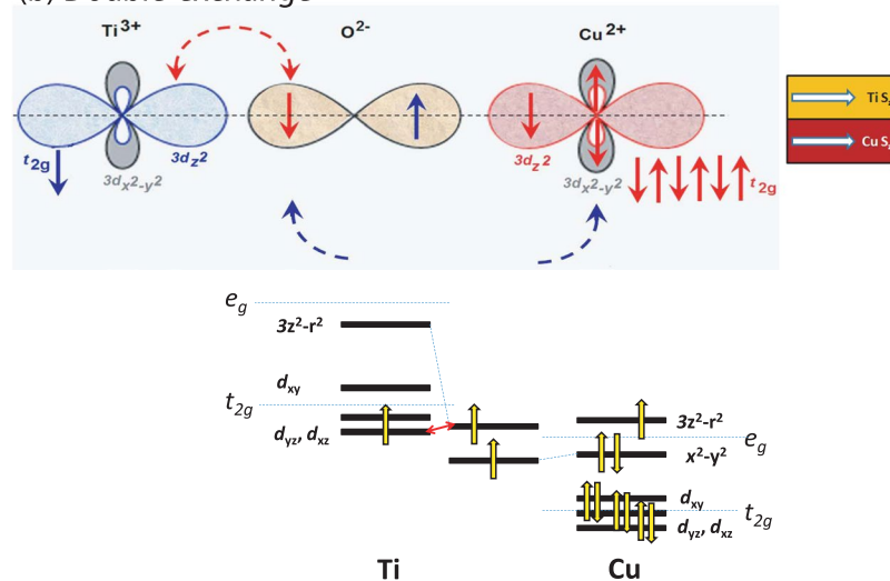
Figure 10. SE and DE coupling mechanisms. Schematic diagram of (a) Superexchange interaction between Mn 3d-O 2p-Ti 3d ( \text{Mn}^{3+} - \text{Ti}^{3+} ) and (b) Double-exchange coupling between Ti 3d-O 2p-Cu 3d ( \text{Ti}^{3+} - \text{Cu}^{2+} ) orbitals in the hybridization process. In one case 3d(3z^2 - r^2) orbital is occupied (LSMO), whereas in the other case the 3d(3z^2 - r^2) orbital with higher energy and 3d(x^2 - y^2) orbital with lower energy are occupied.
