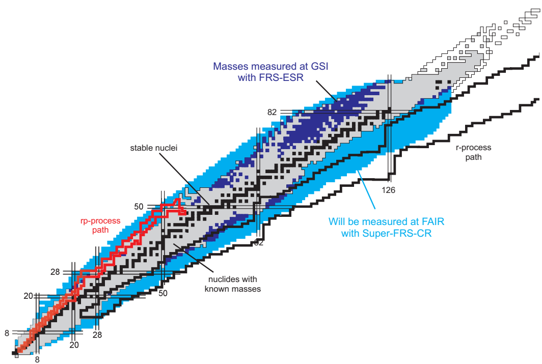
Figure 10: The FAIR reach in nuclear masses (light blue). Masses measured at GSI are shown in dark blue
