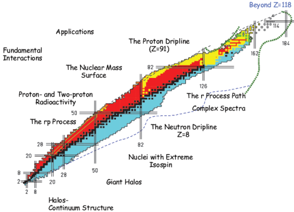
Figure 9: The many opportunities for nuclear physics with RIBs at FAIR.
