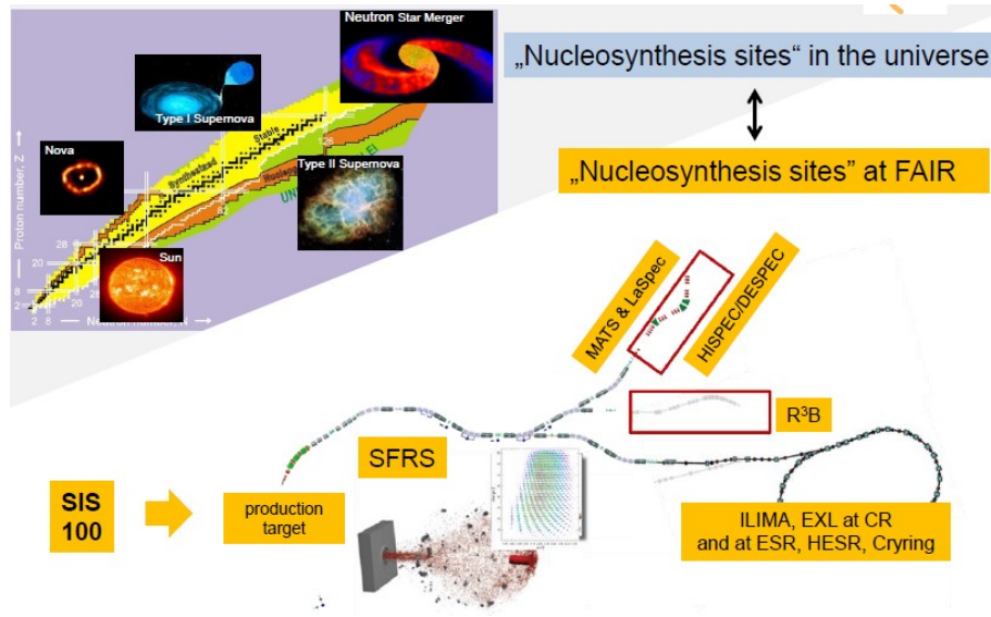
Figure 8: Layout of the nuclear physics RIB experiments at FAIR with the fragmentation target, the Super FRS and the High-Energy, Low-Energy and Ring Branches (see text). As indicated by the nuclear chart, exotic nuclei are crucial for astrophysical nucleosynthesis processes: neutron-deficient nuclei for novae and x-ray bursters and exotic nuclei with strong neutron excess for supernovae and neutron-star mergers. As discussed in the next section, FAIR will allow to produce many of these exotic nuclei and to determine their properties.
