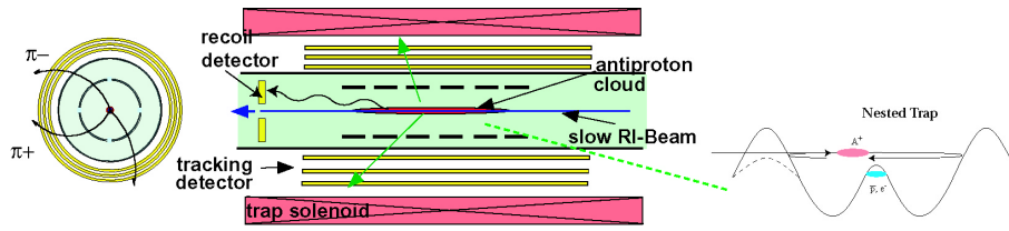
Figure 14: Schematic setup for the experiment Exo+pbar as proposed for FLAIR [181]. Antiprotonic atoms are formed in a solenoid magnet (center) containing a nested Penning trap (right). The proposed detection method is to track charged particles inside the solenoid (left) and to extract halo factors from the number of charged pions produced in the annihilation of the antiproton with a nucleon at the nuclear surface. From [172].
