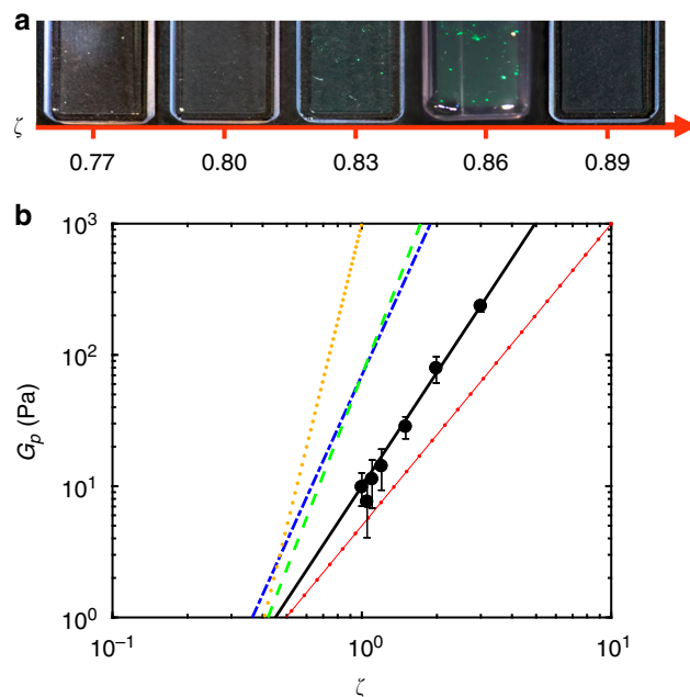
Fig. 2 Phase behavior and G' plateau of suspensions of ultra-low crosslinked (ULC) microgels. a Image of a series of samples of ultra-low crosslinked microgels of increasing volume fraction in water. b Plateau value of G' , G_p (black circles), versus the generalized volume fraction, \zeta . Black line: data fit with G_p \propto \zeta^m . Dotted, dashed, dotted-dashed and line-with-dots lines are taken from refs. 11,13,22,33 , see text for details
