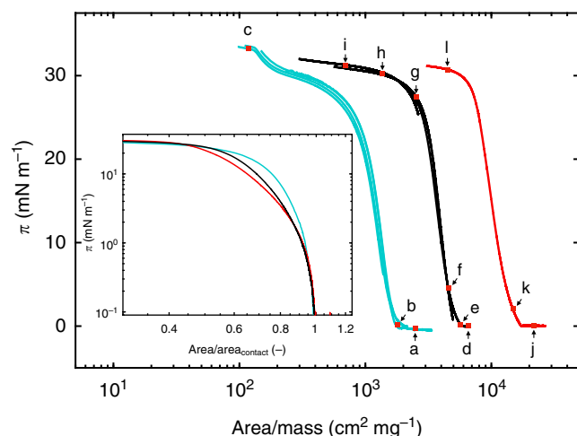
Fig. 3 Compression isotherms for linear, ultra-low crosslinked (ULC) and regular crosslinked microgels. Surface pressure, \pi , versus the area normalized by added mass of microgels (Area/Mass) for 5 mol% crosslinked microgels (cyan lines), ULC microgels (black lines) and linear poly( N -isopropylacrylamide) (pNIPAM; red line) at T = 20.0 \pm 0.5^\circ\text{C} . The red squares with letters a–l indicate the \pi values of the atomic force micrographs in Fig. 4a–l. Inset: Plot of \pi versus the trough area normalized by the trough area at the contact point, Area/Area contact , of 5 mol% crosslinked microgels (cyan line), ULC microgels (black line) and linear pNIPAM (red line) at T = 20.0 \pm 0.5^\circ\text{C} in log–log scale
