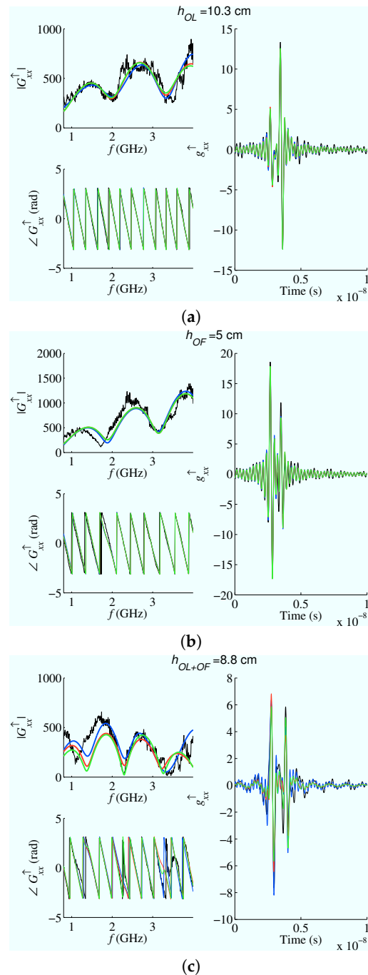
Figure 3. Measured (black curves) and modeled Green's functions in the frequency and the time domains for selected litter thickness levels of the (a) OL, (b) OF and (c) OL-OF configurations of the controlled experiment. The blue curves correspond to modeled Green's functions for the model considering only frequency dependence of litter effective electrical conductivity, reported by André et al. [33], the red curves represent modeled Green's functions for the model accounting for both surface roughness and frequency dependence of litter effective electrical conductivity, and the green curves are modeled Green's functions for the model considering surface roughness only.
