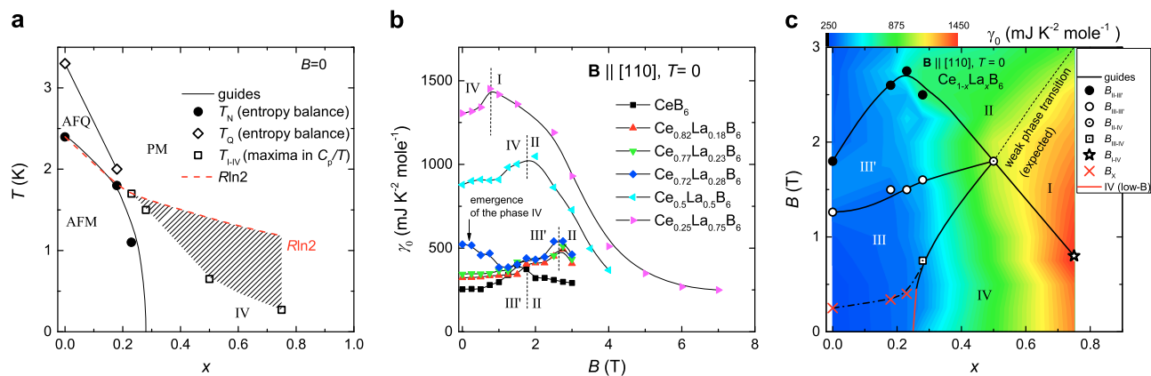
Fig. 5 The B = 0 x - T phase diagram, B -dependent and x -dependent \gamma_0 , and T = 0 x - B phase diagram of \text{Ce}_{1-x}\text{La}_x\text{B}_6 . a B = 0 x - T phase diagram is shown. It is completed by placing coordinates of specific heat anomalies in the x - T plane. The I-IV transition with transition temperature T_{\text{I-IV}} becomes broad above x \simeq 0.3 . The region of broad transitions is roughly coincident with the hatched area between the S_p = R\ln 2 isentropic line and the T_{\text{I-IV}}(x) . b The Sommerfeld coefficient as a function of B with different values of x is presented. Locations of local maxima (see short vertical dashed lines) are coincident with the critical points extrapolated from the lowest- T MCE anomalies. c The black dot and the white circle designate B_{\text{II-III'}} and B_{\text{III-IV}} , determined by the MCE analysis, respectively. The high-entropy region exists below B_x and the black dash-dotted line connects \times symbols as a guide to the eye. The red segment for the low- B III-IV phase boundary is to emphasize large increase of \gamma_0 upon entering the phase IV which can be confirmed in b . B_{\text{II-IV}} (white dotted-circle), and B_{\text{I-IV}} (white star) are also determined by the MCE analysis (see Supplementary Figs. 2 and 3, and Supplementary Note 3). The background is contour plot of \gamma_0(x, B)
