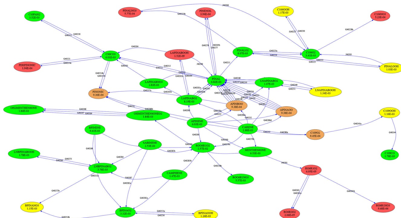
Figure 4. Skeletal reduction of terpene chemistry in the MOM reaction scheme (only C 10 species are shown here). Vertex colors and OIC values correspond to those in Table 3; only the green and yellow species are kept in the reduced mechanism.
