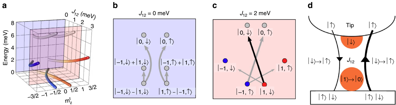
Figure 3 | State evolution of the combined spin system. (a) Simulated evolution of the state energies and the total magnetic moments, m_z^t , of the combined spin system, S_1 = 1 and S_2 = 1/2 , with Heisenberg coupling J_{12} . The colour code shows the projected magnetic moment ( S_{1,z} ) of the S_1 subsystem (blue: -1 , red: +1 ). (b) 2D cut at J_{12} = 0 meV. Grey arrows show the main excitation channels from the two degenerate ground states. This scheme is a doublet of the one shown in Fig. 1f due to the additional spin degree of S_2 . (c) 2D cut at J_{12} = 2 meV. The coupling introduces a strong polarization of the states. Angular momentum conservation only allows \Delta m_z = 0, \pm 1 transitions, suppressing the excitation to the energetically lower states (thin grey arrows). The transitions to the energetically higher states strongly depends on the spin distributions in tip and sample as well as on the tunnelling direction. (d) Illustration of the origin of the bias asymmetry for the transition depicted as black arrow in c.
