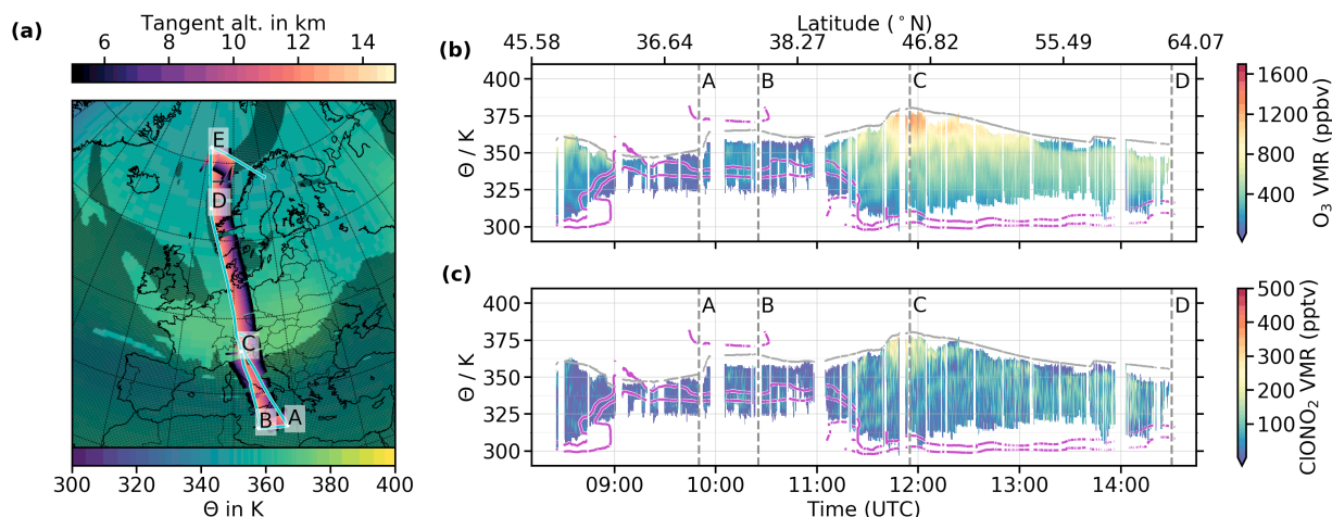
Figure 5. Flight PGS06 (12 January 2016): (a) Flight path (cyan) on a map with MERRA2 potential temperatures (lower colorbar) at typical HALO cruise altitude of 13 km. Regions outside the polar vortex (according to Nash et al. (1996) at \theta = 370 K) are marked with a grey shadow. Way points are marked with capital letters. The tangent altitudes of GLORIA measurements are shown in the upper colorbar. Right panels: GLORIA cross section of (b) O 3 and (c) ClONO 2 (using GLORIA potential temperature). The flight level (approximated using MERRA2 potential temperature) is marked with a grey line and white spaces mark regions without data. The MERRA2 potential vorticities of 2 and 4 PVU are marked with magenta lines and way points are marked with grey vertical dashed lines.
