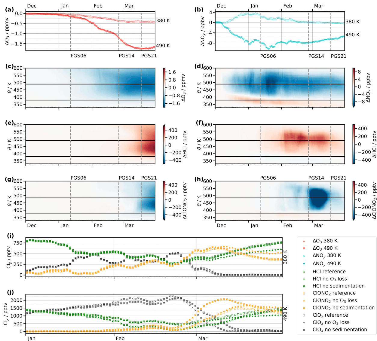
Figure 10. CLaMS vortex average (equivalent latitude > 75^\circ\text{N} ) time series for ozone loss at 380 K and 490 K (a), and as cross section (c). Denitrification is presented in the same manner (b,d). Differences in HCl and \text{ClONO}_2 between a reference simulation and a simulation without the influence of ozone depletion (e,g) or PSC sedimentation (f,h). Altitudes of 380 K and 490 K, which are illustrated in other panels, are marked with horizontal lines. The bottom panels show \text{ClO}_x (black), HCl (green), and \text{ClONO}_2 (orange) for the reference simulation (open squares), and for the sensitivity simulations without ozone depletion (+) and without PSC sedimentation (x) at 380 K (i) and 490 K (j). Please note that these time series, in contrast to others in this figure, start in January.
