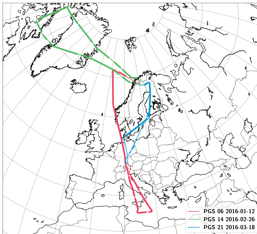
Figure 1. Flight paths of flights PGS06 (12 January 2016), PGS14 (26 February 2016) and PGS21 (18 March 2016) on which GLORIA measurements were performed. Aircraft positions with measurements in GLORIA high spectral resolution mode are marked as bold lines.
