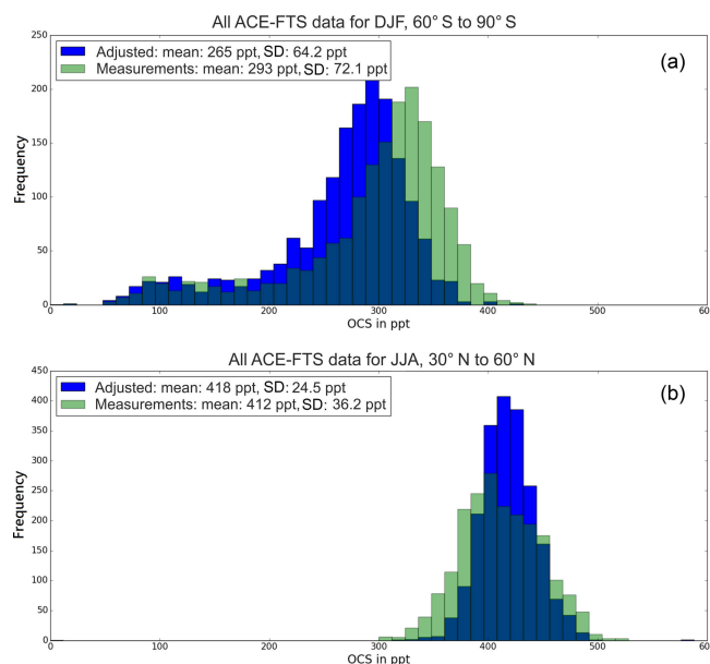
Figure 3. Comparison of the distributions and resulting mean and standard deviation values of measured (green) OCS and the adjusted measurements using Eq. (2) (blue) for the same time–latitude bins indicated by the black (a) and red (b) boxes in Fig. 1. Histograms include all 12 years of ACE-FTS OCS mixing ratio measurements at 16 km altitude.
