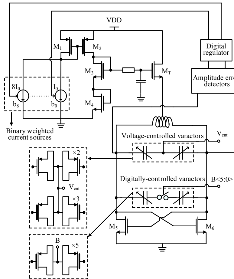
Figure 3.7: VCO architecture.
