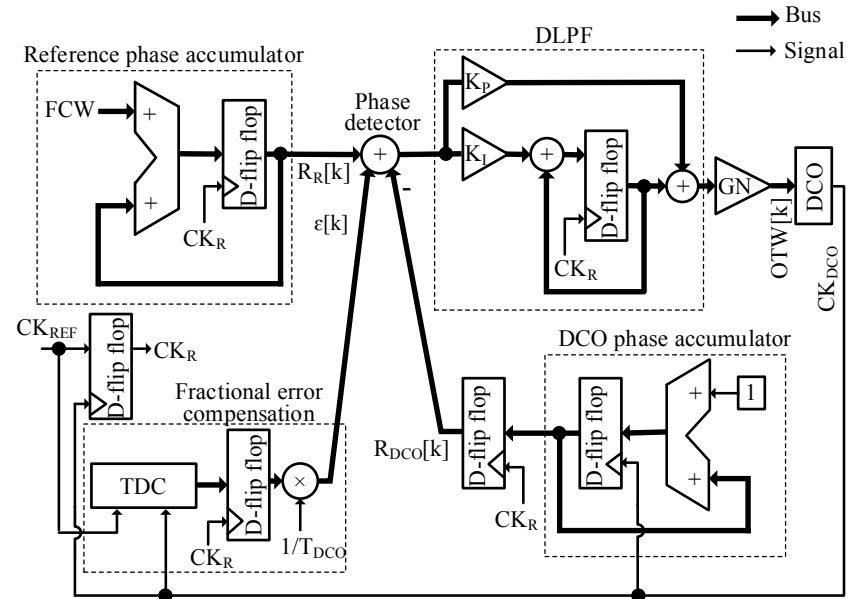
Figure 4.2: Accumulator-based digital PLL block diagram in Simulink.
