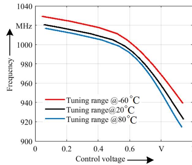
Figure 3.28: PLL tuning range at different temperatures.
