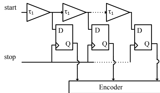
Figure 4.13: Block diagram of delay-line TDC.
