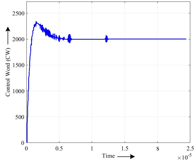
Figure 4.30: Control word of the DCO in the digital PLL.
