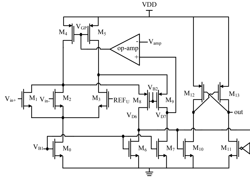
Figure 3.13: Schematic of amplitude error detector.
