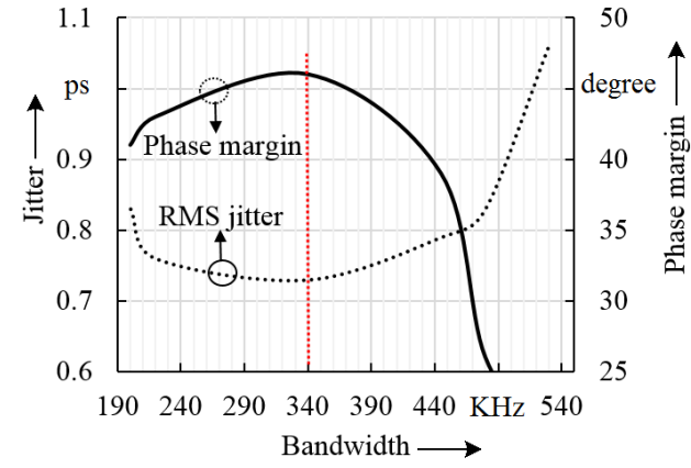
Figure 3.3: Phase margin and RMS jitter.
