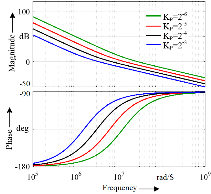
Figure 4.22: Bode plot of H_{ol}(s) for \zeta = \sqrt{2}/2 .
