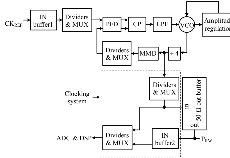
Figure 3.24: Top view of the PLL core and clocking system.
