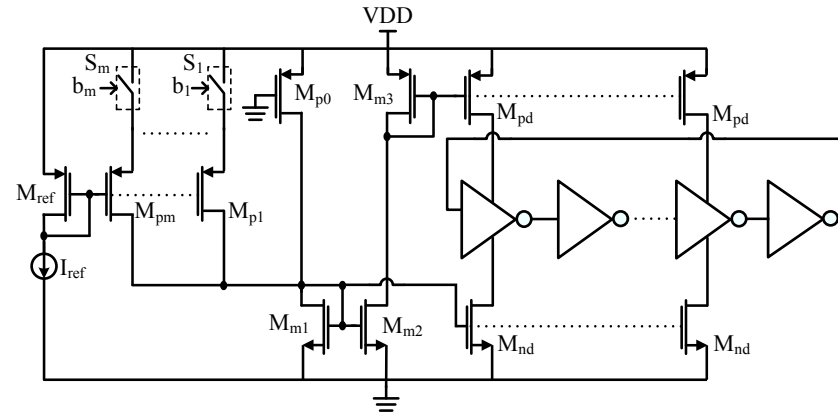
Figure 4.7: Ring DCO using current starving.
