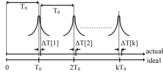
Figure 4.26: Development of accumulative jitter.
