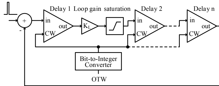
Figure 4.10: Proposed DCO model in Simulink.
