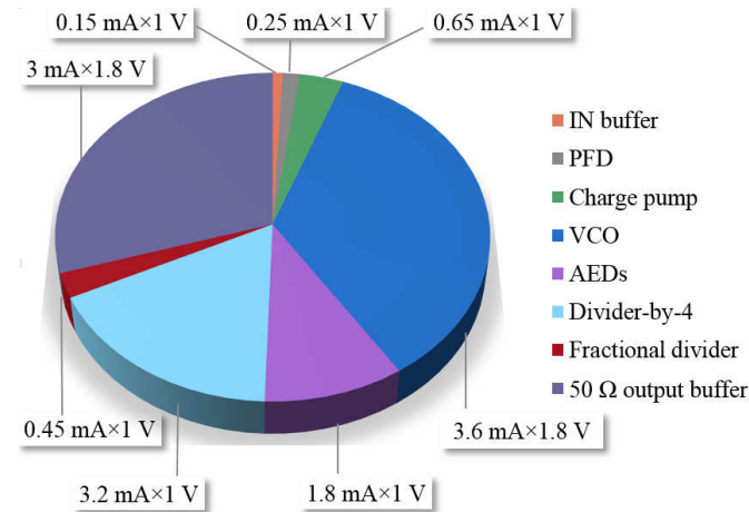
Figure 3.30: Power consumption of PLL's blocks.
