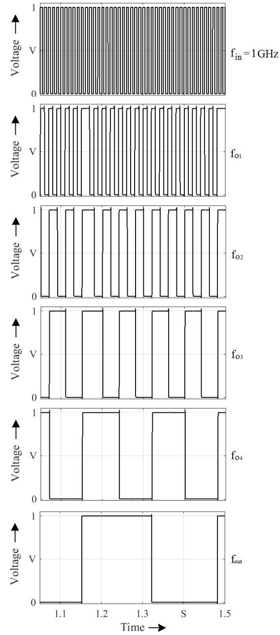
Figure 3.22: Transient simulation of five bit multi-modulus divider.
