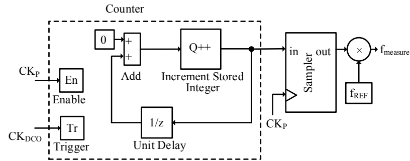
Figure 4.31: Frequency monitoring of the digital PLL in Simulink.
