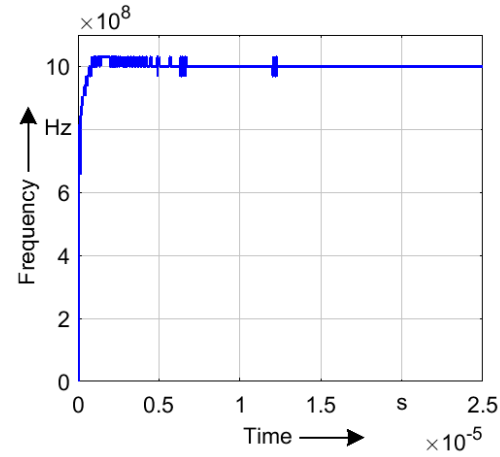
Figure 4.32: Measured frequency of the DCO.
