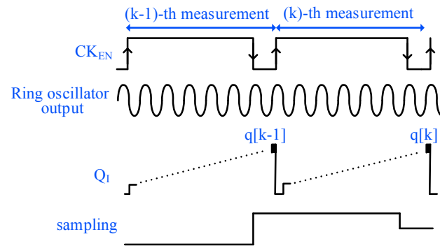
Figure 4.17: Operation of the proposed TDC by its waveforms.
