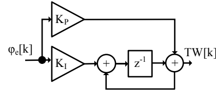
Figure 4.18: DLPF z-domain model.
