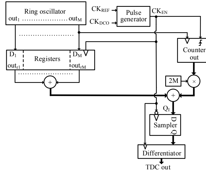
Figure 4.16: Proposed TDC design in Simulink.
