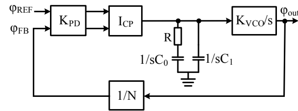
Figure 3.2: The Laplace domain representation of the PLL.
