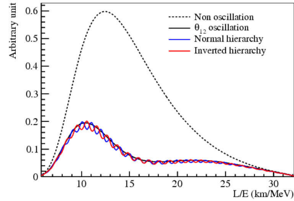
Figure 2.3: Reactor neutrino spectra [6].
