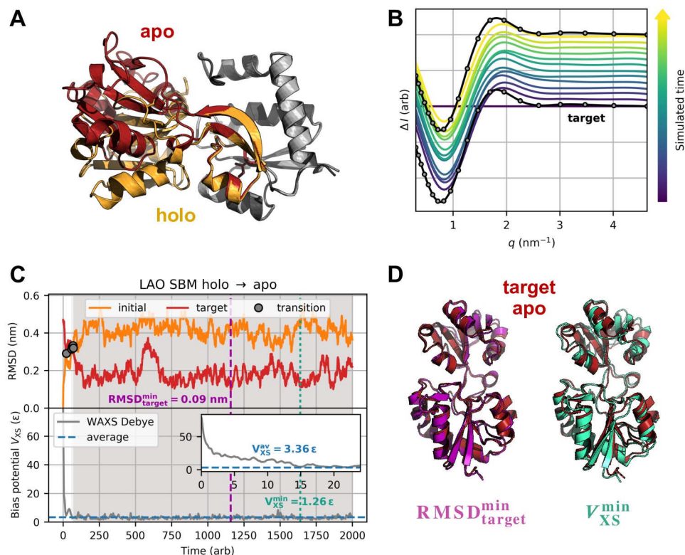
Fig 3. Method validation using the example of LAO protein's holo-to-apo transition. Results are shown for parameters (T, k_x) = (50, 9 \cdot 10^{-11} \text{ } \epsilon) . (A) LAO protein test system. LAO protein undergoes a large-scale conformational transition upon ligand binding, meaning the lobes are clearly separated in the unliganded state (apo form, red), whereas in mutual contact with lysine ligand bound (holo form, orange). Congruent parts in holo and apo conformation are depicted in grey. (B) Artificial target data for the holo-to-apo transition (grey circles). 20 q points between 0.3 \text{ nm}^{-1} and 4.6 \text{ nm}^{-1} were included. Theoretical difference intensities of simulated structures (blue to yellow) were plotted with small offsets and approached the target curve in the course of the simulation. (C) Initial and target RMSD (top) and bias energy (bottom) versus simulated time. The refinement involved one instantaneous transition from initial holo to target apo state in terms of intersecting RMSD curves (grey dots). With the simulation approaching its designated target state, the bias potential minimized accordingly. (D) Best structures as measured by target RMSD and bias potential. \text{RMSD}_{\text{target}}^{\text{min}} structure (purple) and V_{\text{XS}}^{\text{min}} structure (turquoise) exhibit target RMSDs of 0.09 \text{ nm} and 0.16 \text{ nm} , respectively.
