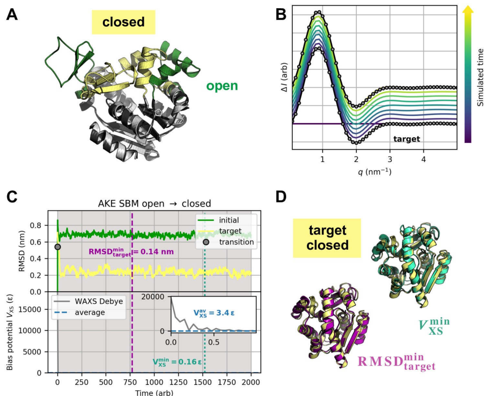
Fig 2. Method validation using the example of AKE's open-to-closed transition. Results are shown for parameters (T, k_r) = (50, 8 \cdot 10^{-9} \epsilon) . (A) AKE test system. Open (green) and closed (yellow) conformations with CORE domain (grey) spatially aligned. (B) Artificial target data (grey circles) were computed from absolute Debye intensities. Theoretical difference curves of simulated structures (blue to yellow) almost perfectly match the target data and were plotted with small offsets. (C) Initial and target RMSD (top) and bias energy (bottom) versus simulated time. (D) Best structures as measured by target RMSD and bias energy. \text{RMSD}_{\text{target}}^{\text{min}} structure (purple) and V_{XS}^{\text{min}} structure (turquoise) exhibit target RMSDs of 0.14 nm and 0.20 nm, respectively.
